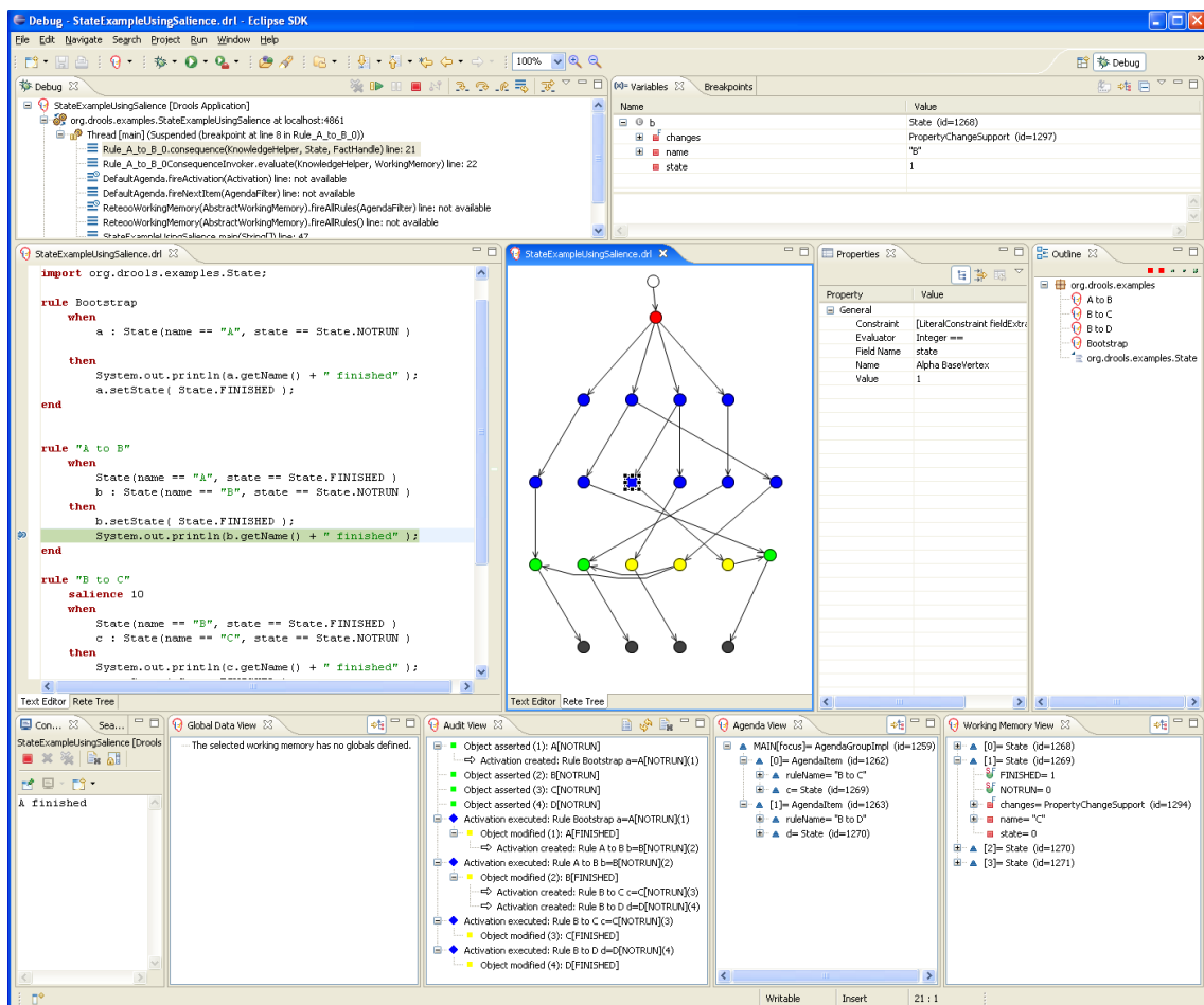
Figure 8.11. Debugging
