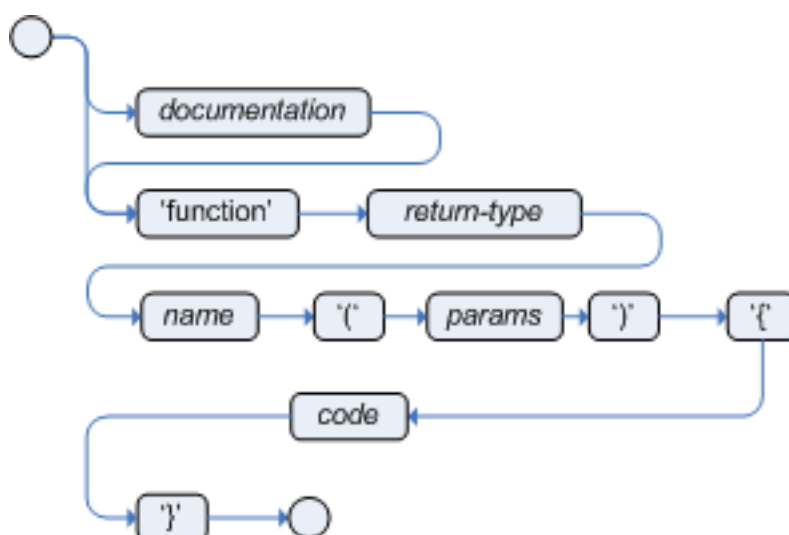
Figure 5.7. function
