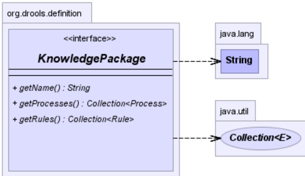
Figure 4.4. KnowledgePackage
