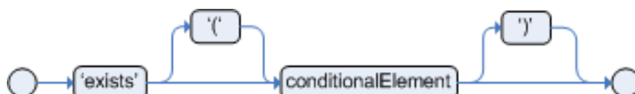
Figure 5.24. exists
