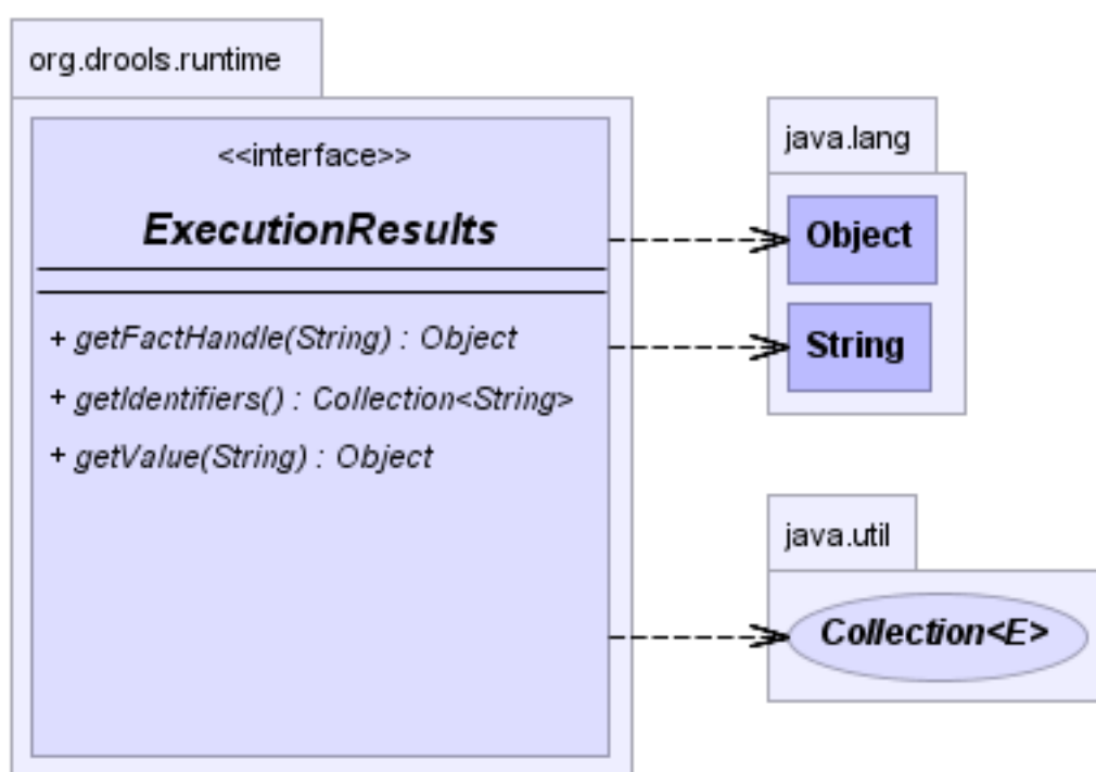
Figure 4.28. ExecutionResults
