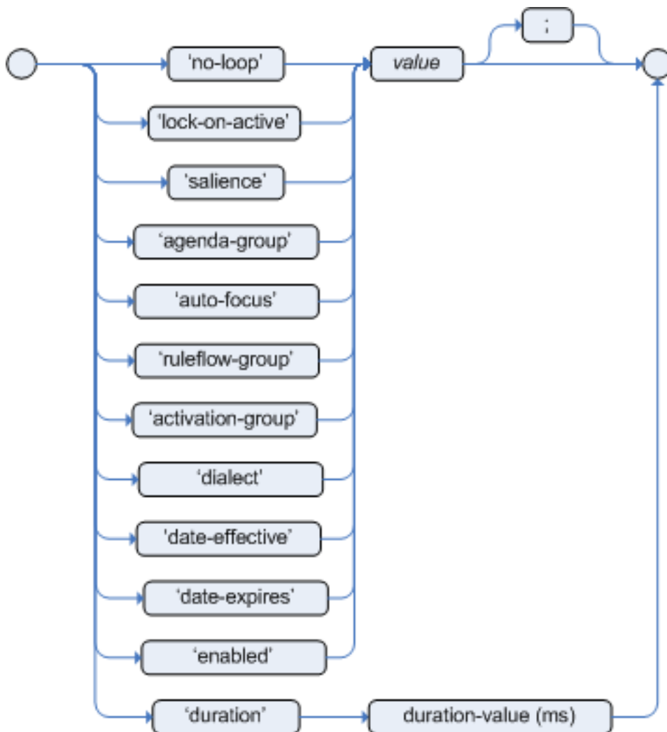
Figure 5.11. rule attributes
