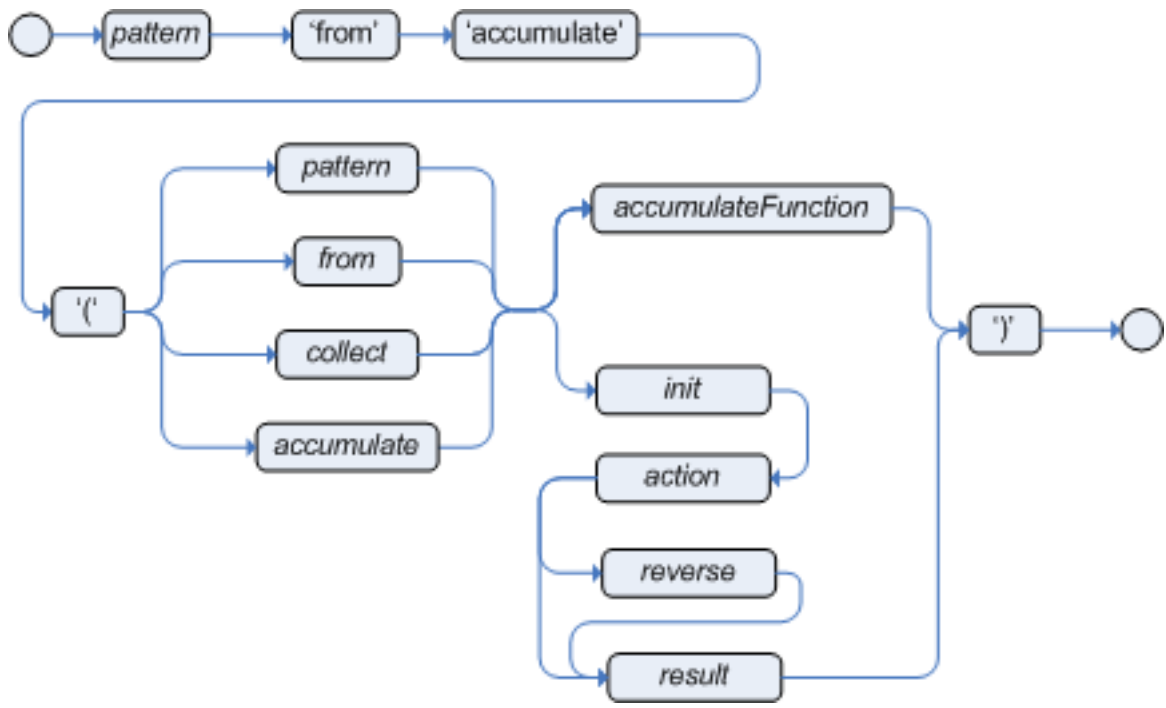
Figure 5.28. accumulate
