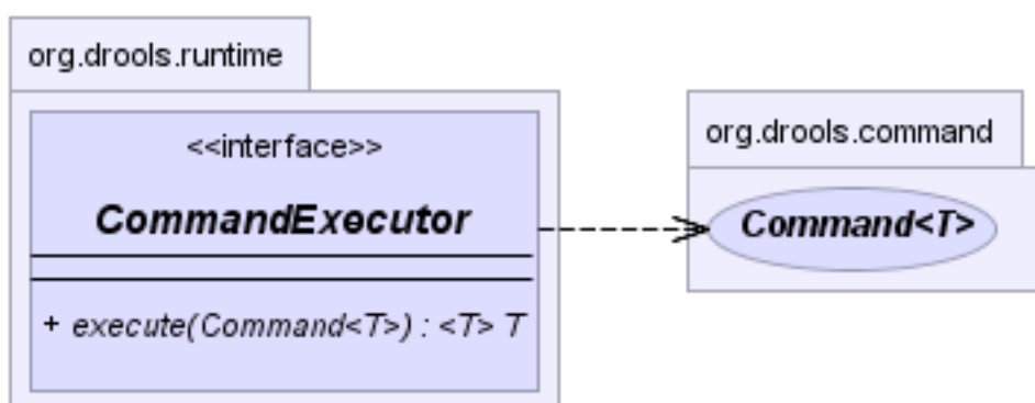
Figure 4.27. CommandExecutor
