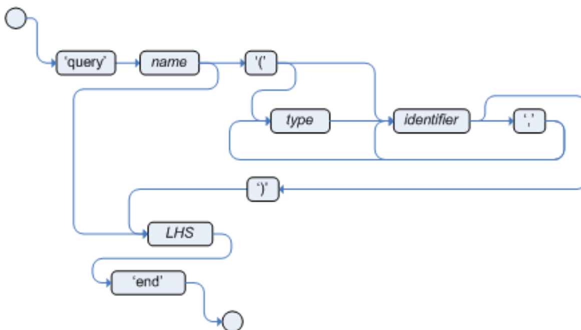
Figure 5.30. query
