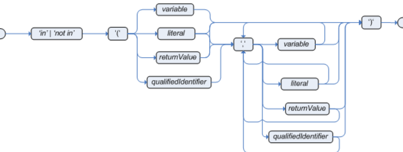
Figure 5.17. compoundValueRestriction
