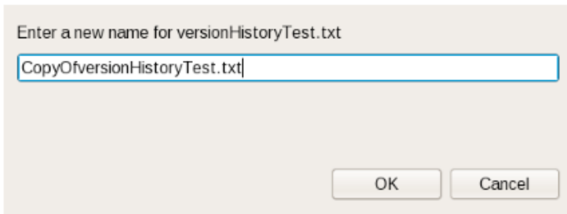
Figure 9.27. Copy
