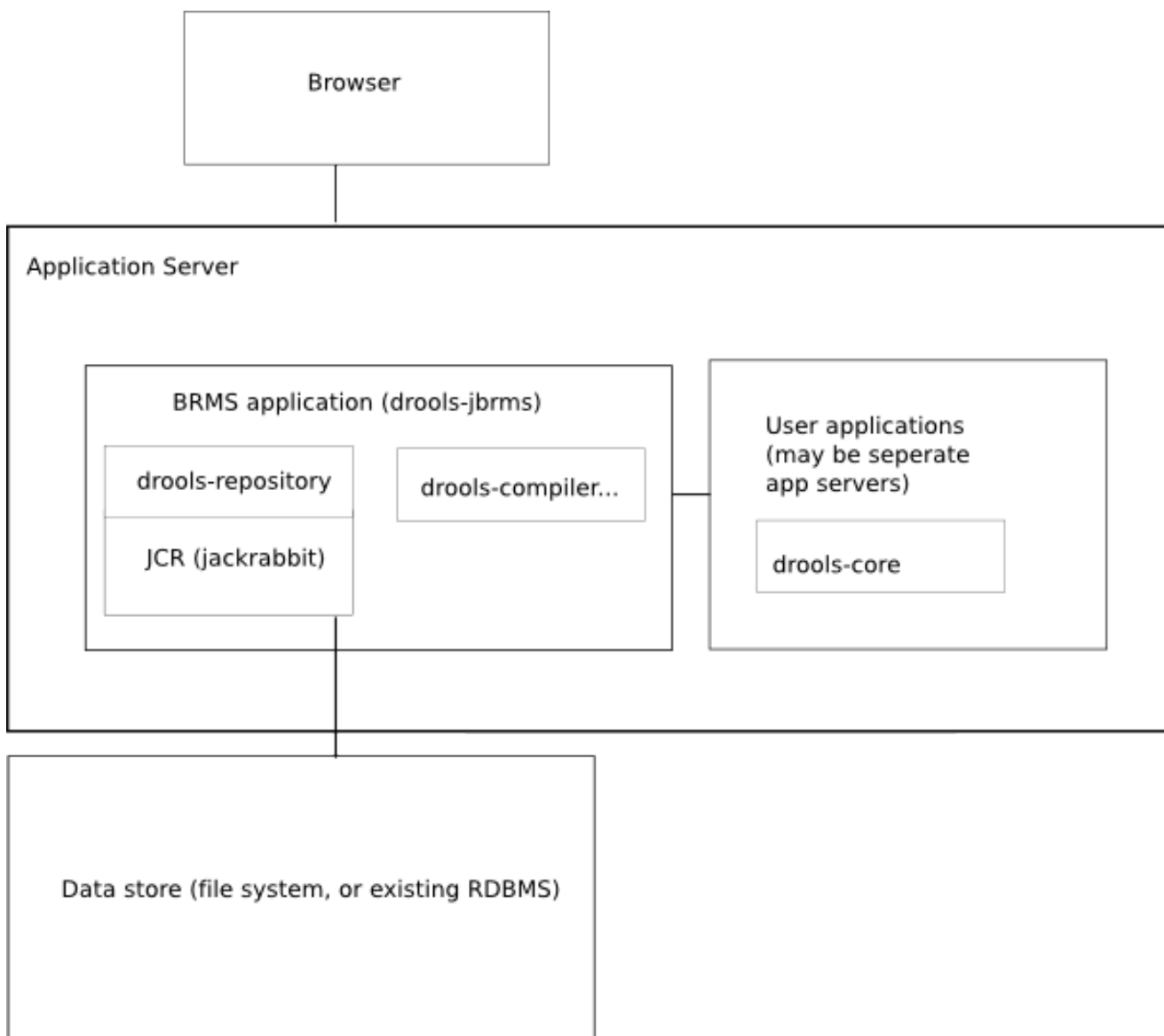
Figure 16.1. Architectural diagram
