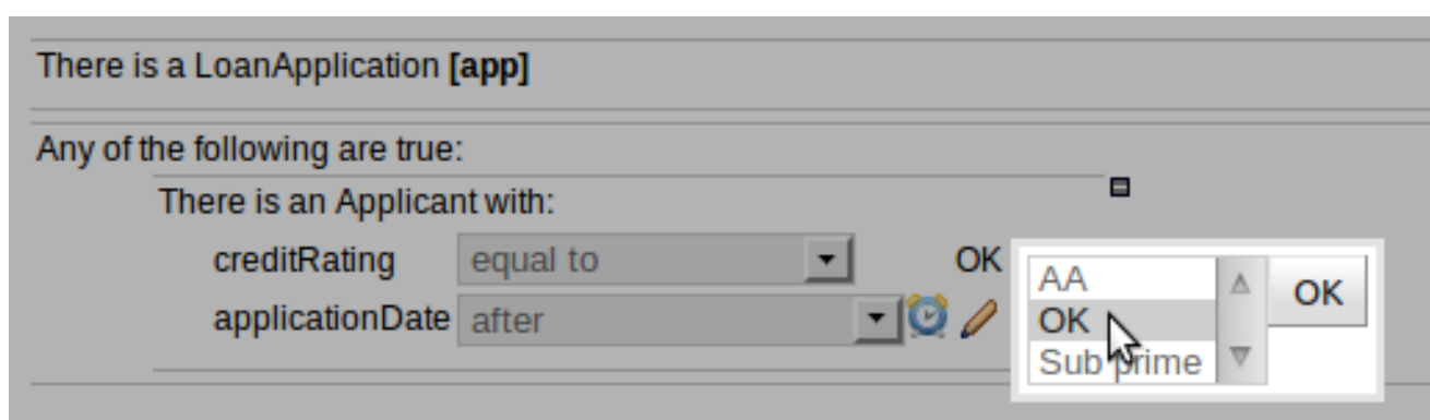
Figure 4.19. Data enumeration showing as a drop down list
