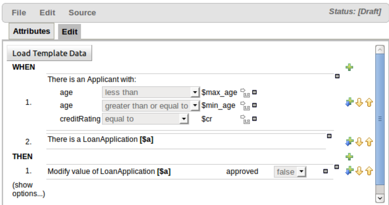
Figure 4.36. Rule template in the guided editor
