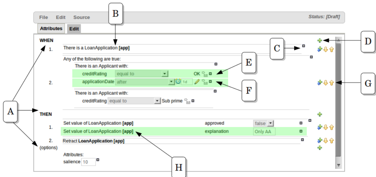
Figure 4.18. The guided BRL editor
