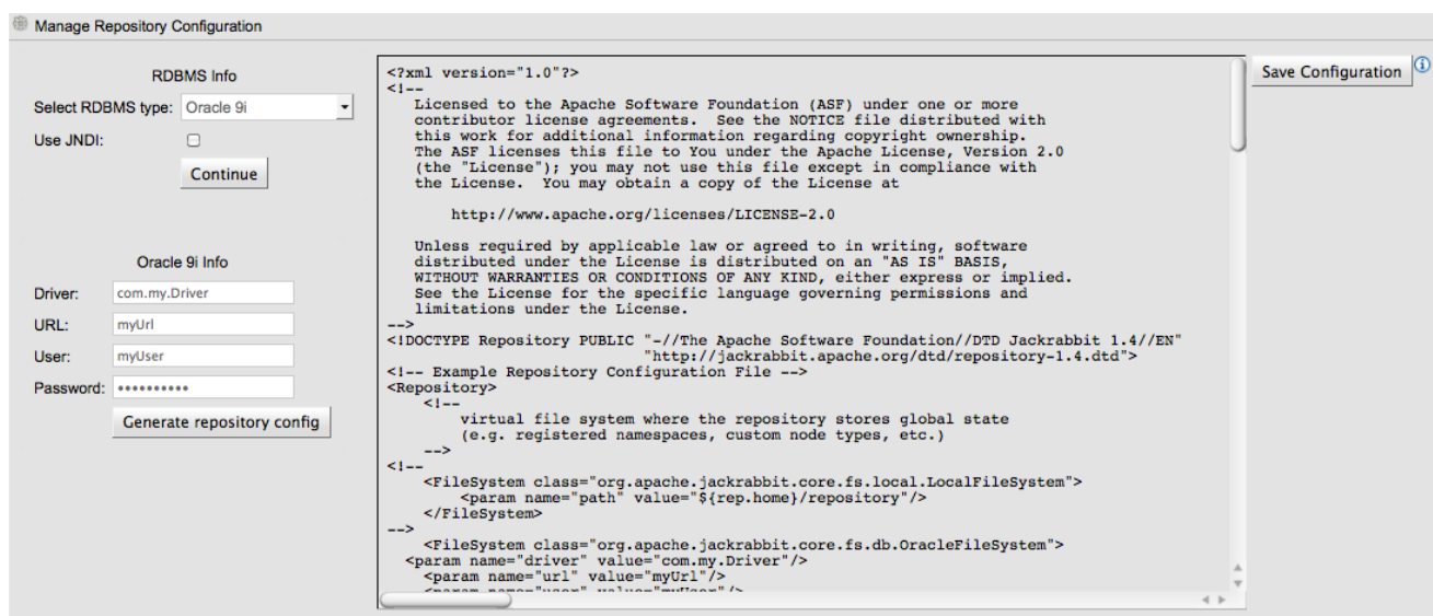
Figure 11.4. Generated repository.xml
