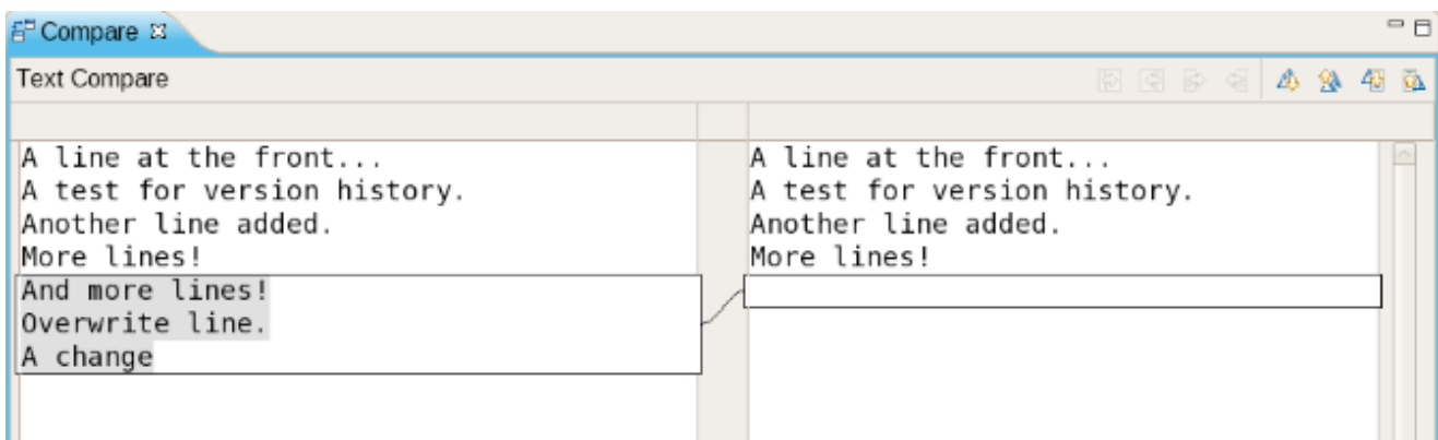
Figure 9.20. Compare
