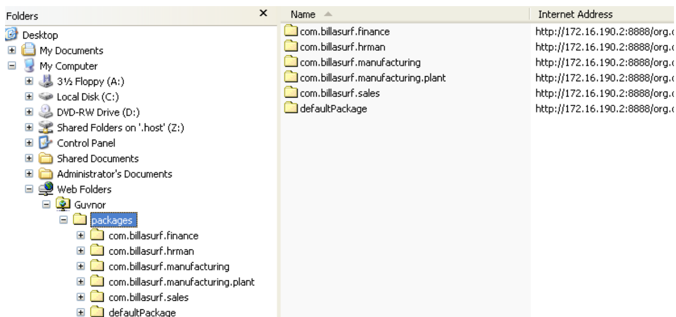
Figure 9.4. Windows webdav
