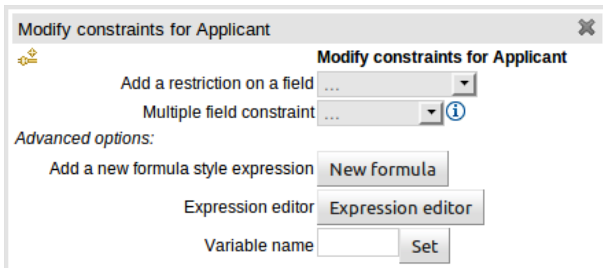
Figure 4.23. Adding constraints
