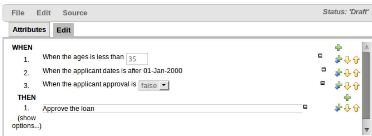
Figure 4.24. DSL rule
