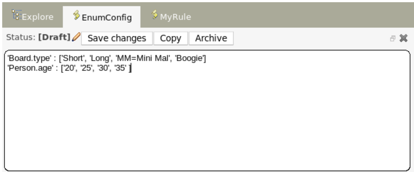
Figure 4.55. Data enumeration
