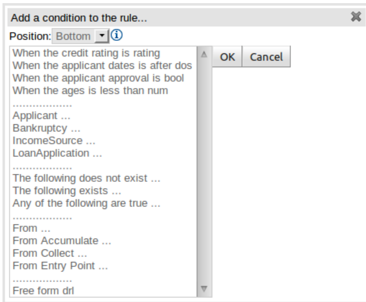
Figure 4.22. Adding Patterns
