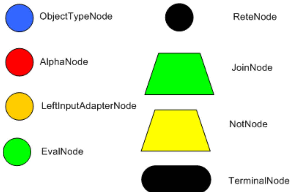
Figure 3.3. Rete Nodes
