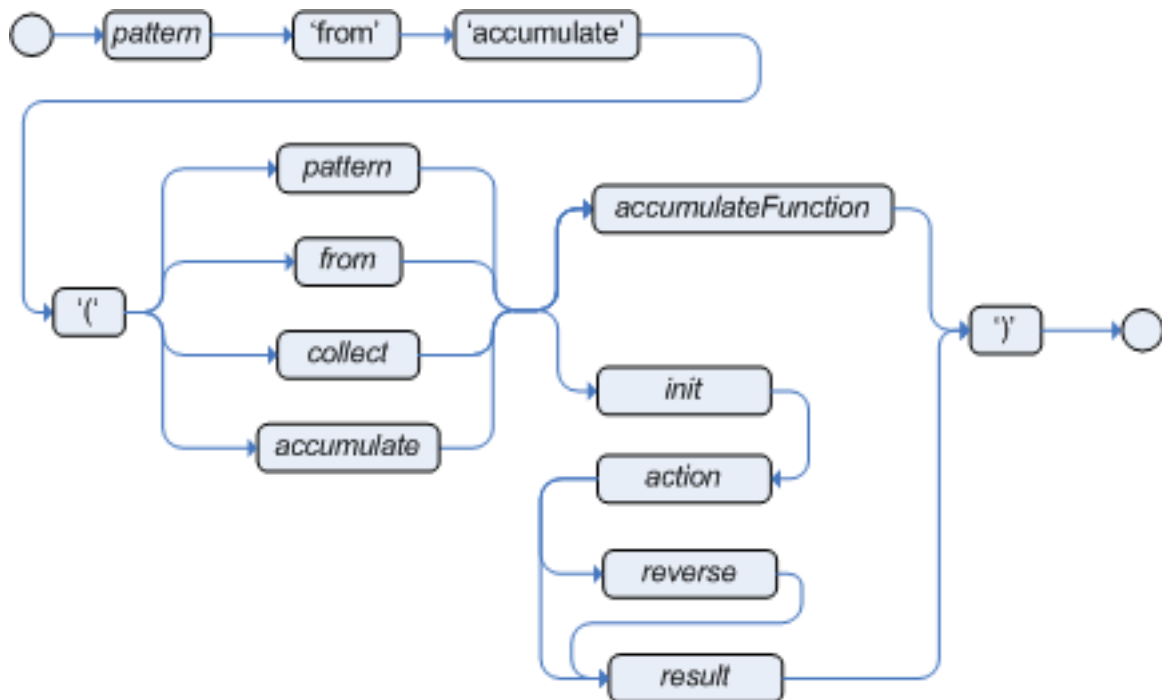
Figure 5.28. accumulate
