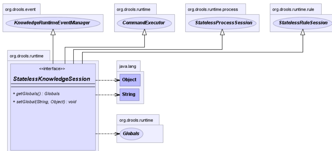
Figure 4.26. StatelessKnowledgeSession
