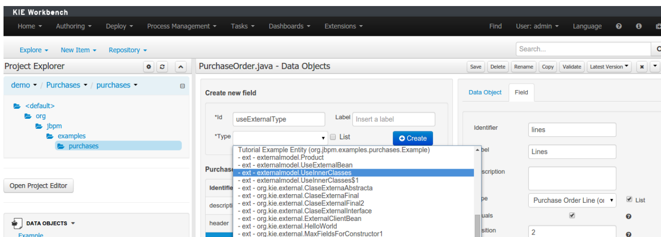
Figure 16.72. Identifying external objects.
