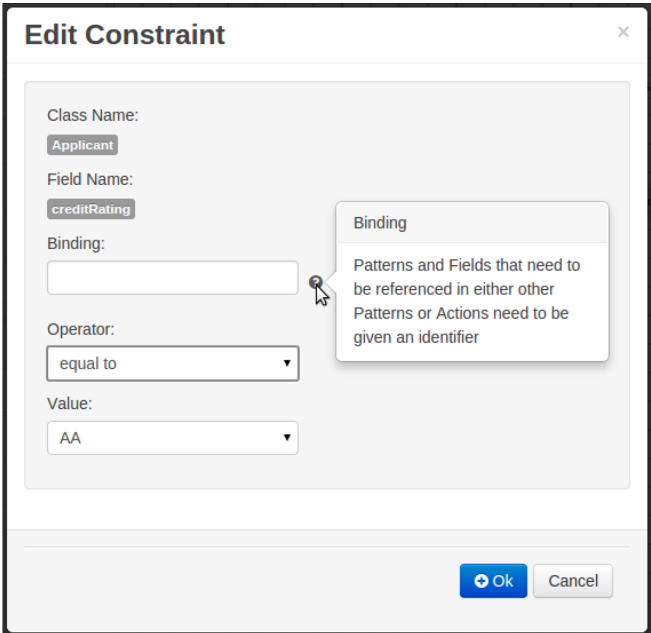
Figure 17.54. Guided Decision Trees - Field Constraint Editor
