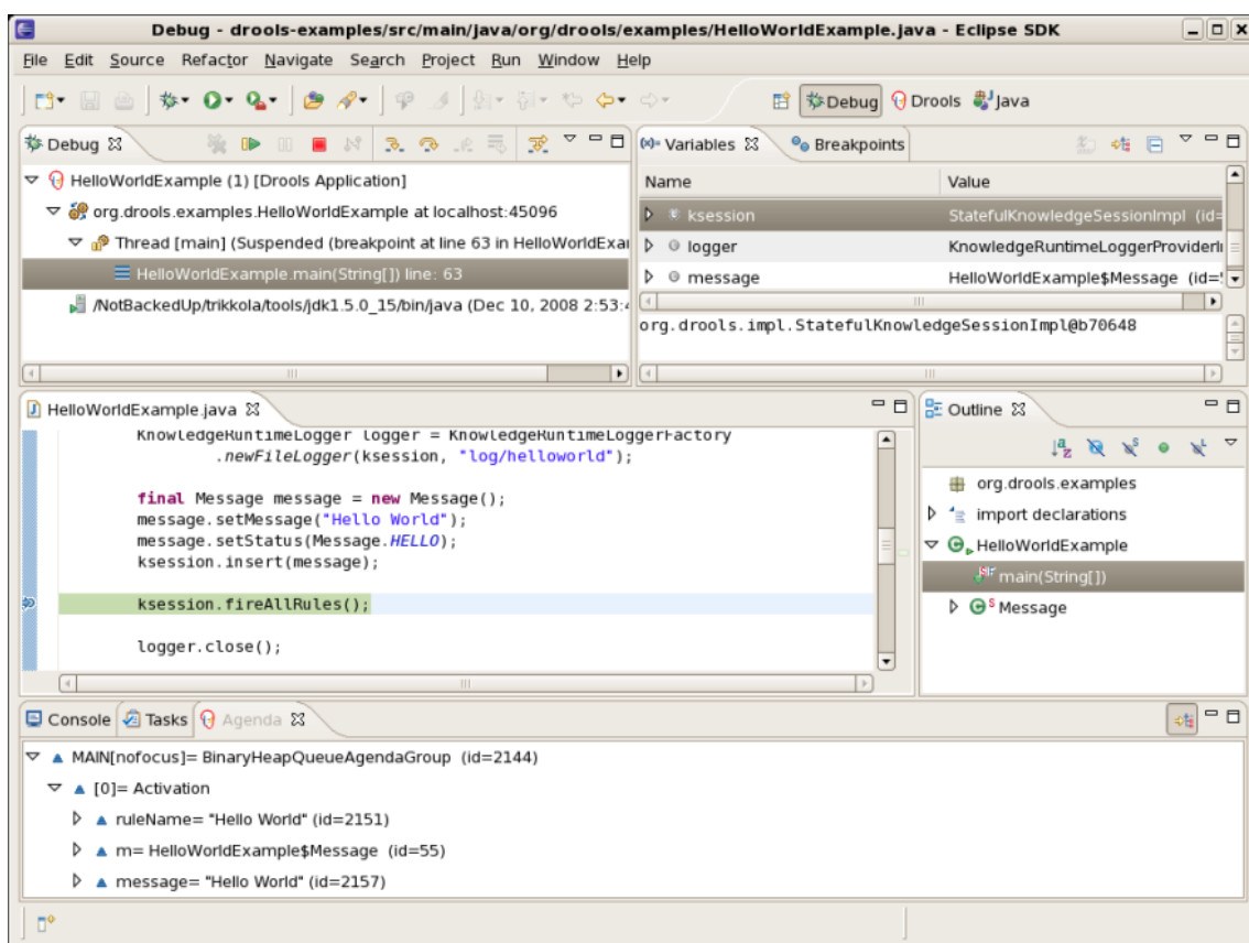
Figure 21.1. Hello World: fireAllRules Agenda View
