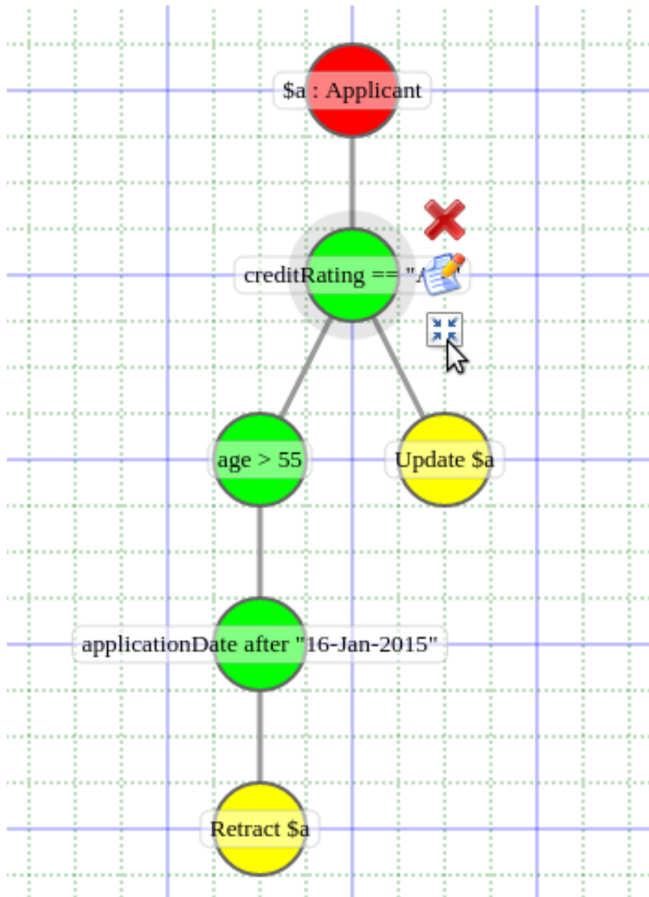
Figure 17.58. Guided Decision Trees - Collapsing nodes
