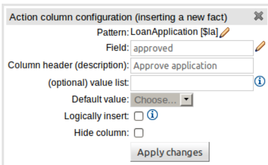
Figure 17.30. Set the value of a field on a new fact popup
