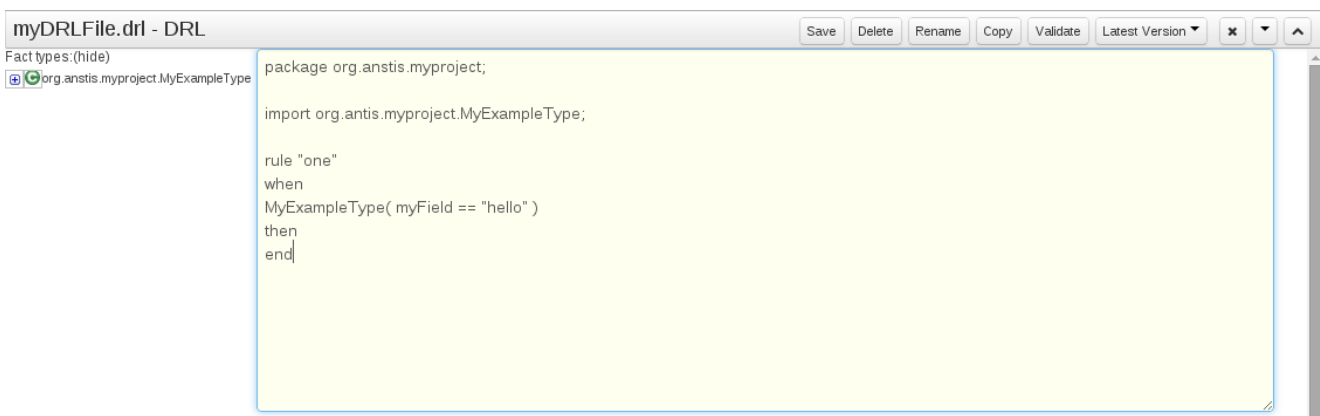
Figure 16.15. Defining a rule
