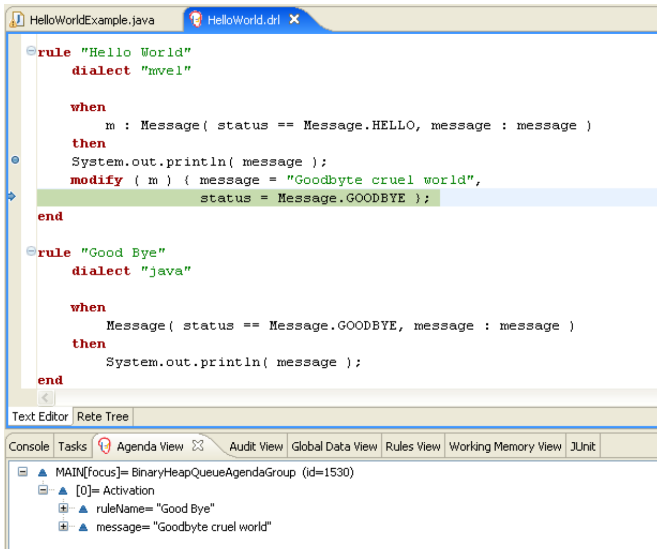
Figure 21.2. Hello World: rule "Hello World" Agenda View
