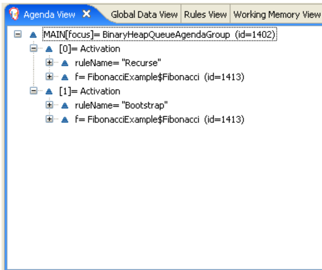
Figure 21.7. Fibonacci Example: "Recurse" Agenda View 1
