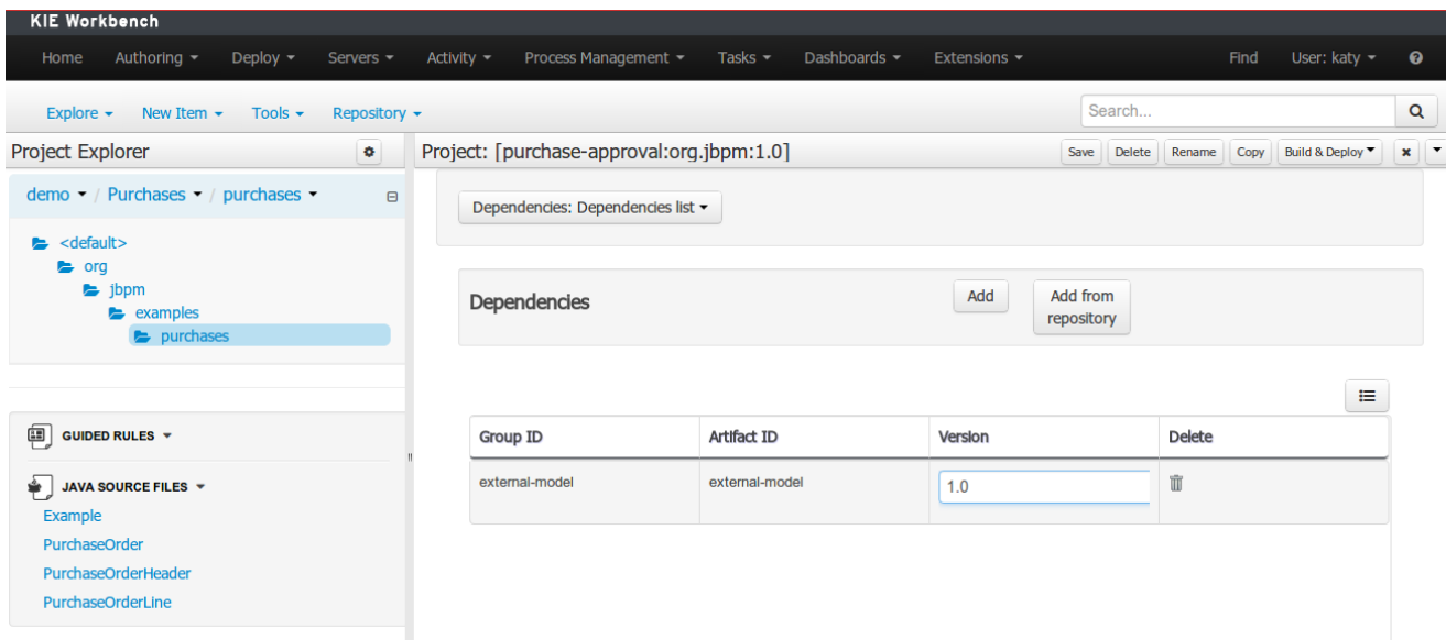
Figure 16.63. Dependency line edition.
