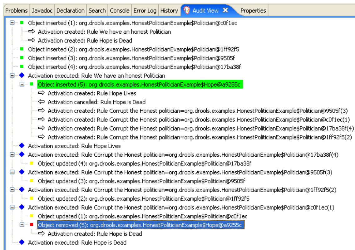
Figure 21.17. Honest Politician Example Audit View
