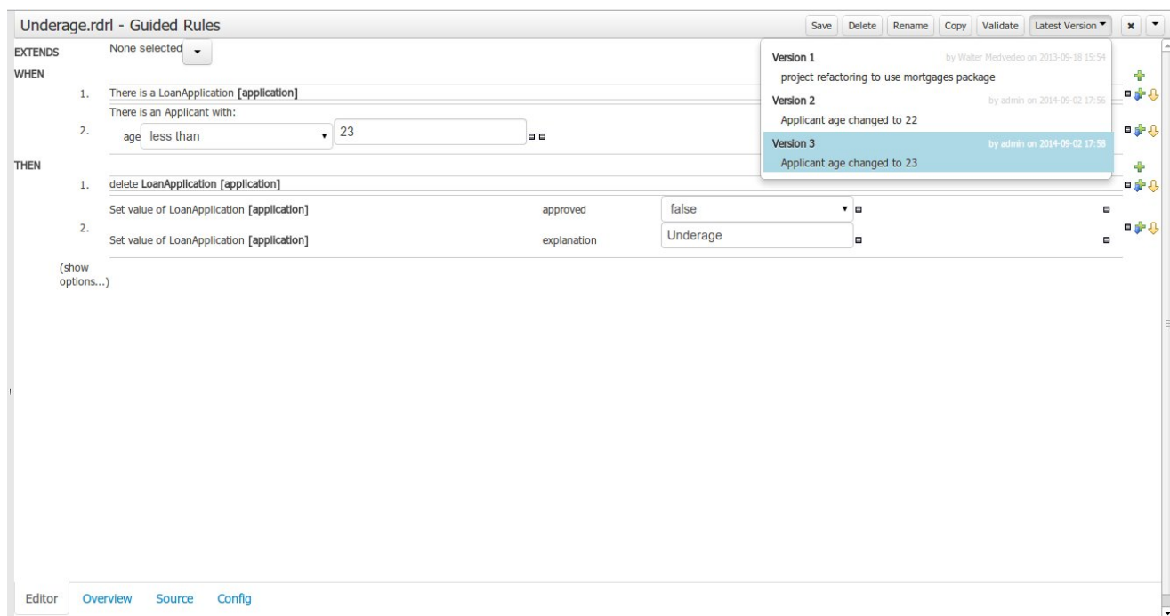
Figure 2.14. Version selection dropdown
