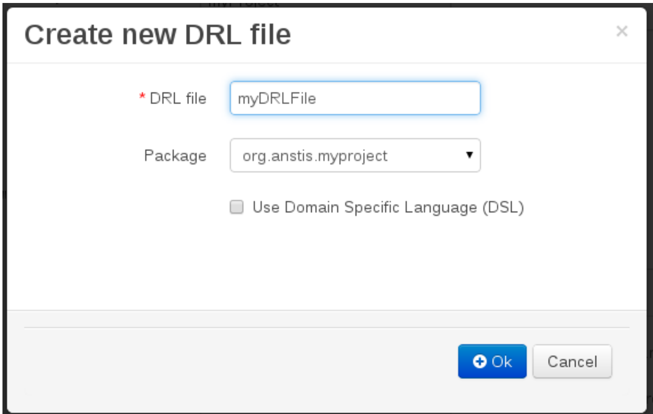
Figure 16.14. Entering file name for rule
