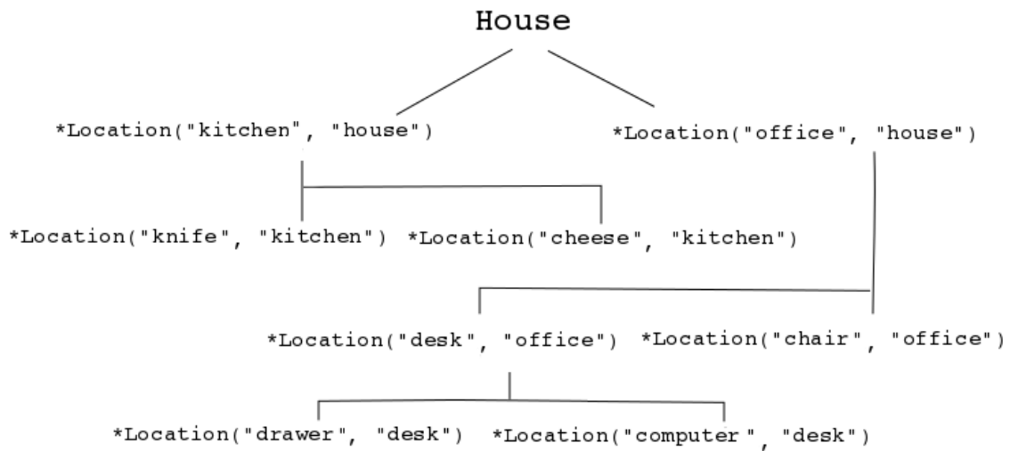
Figure 21.46. Transitive Reasoning Graph of a Drawer
