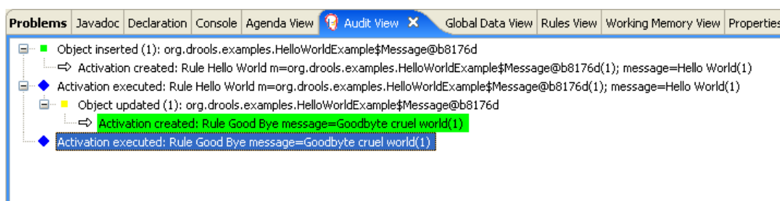
Figure 21.3. Hello World: Audit View
