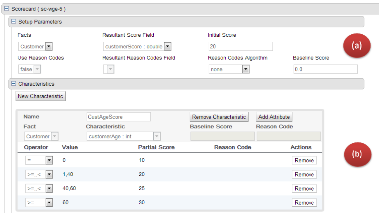
Figure 17.61. Scorecard Asset - Guided Editor
