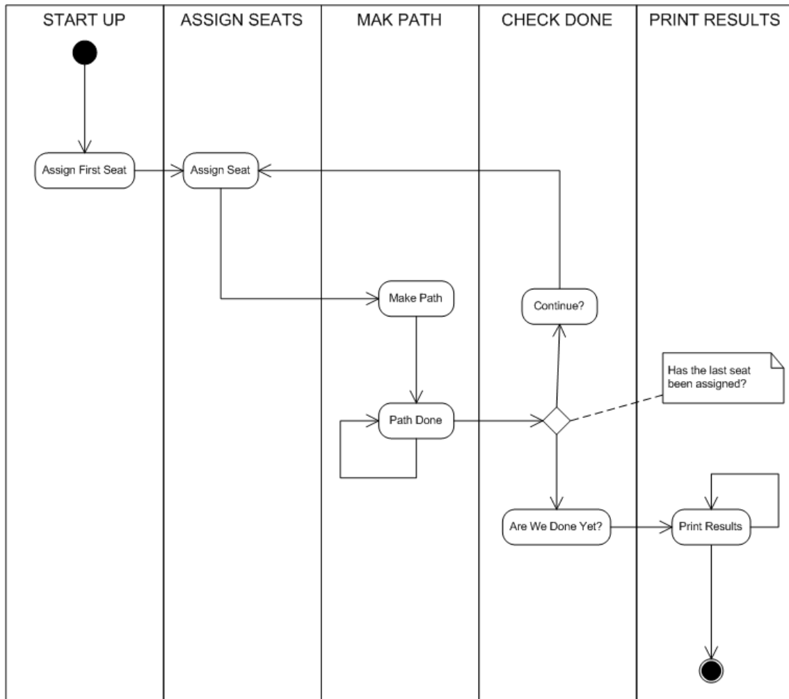
Figure 21.41. Manners Activity Diagram
