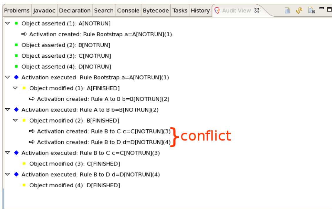
Figure 21.4. Salience State Example Audit View
