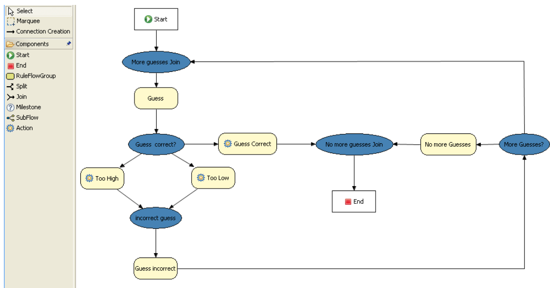
Figure 21.23. RuleFlow for the NumberGuess Example
