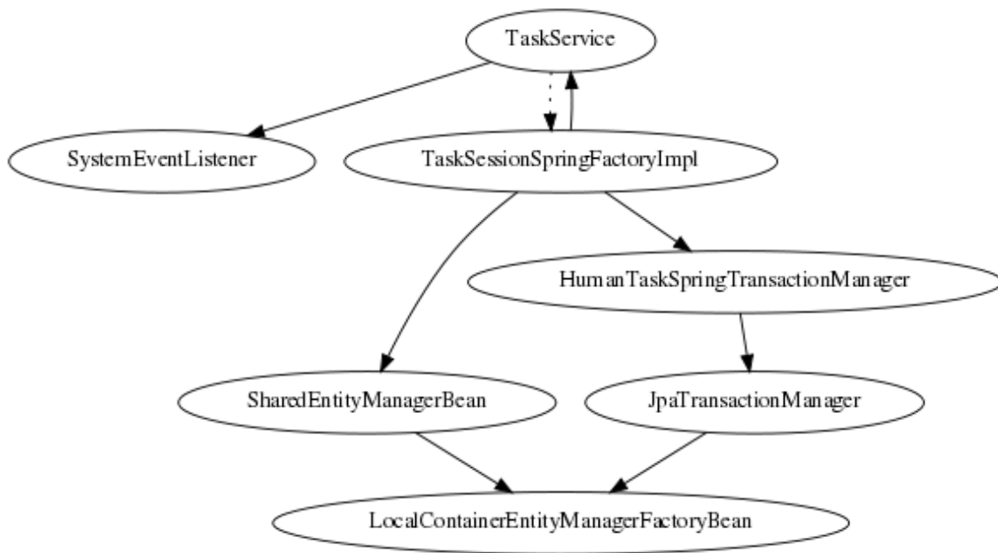
Figure 12.22. Spring Human Task integration injection dependencies
