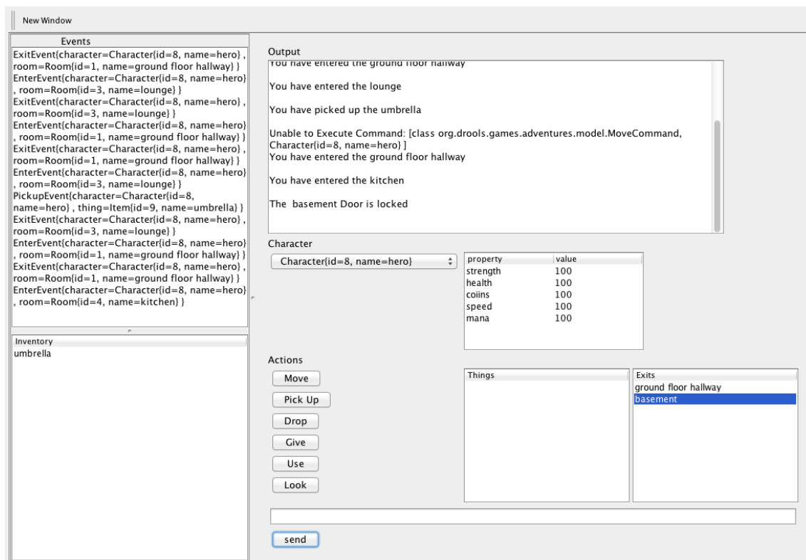
Figure 21.31. Text Adventure Screenshot
