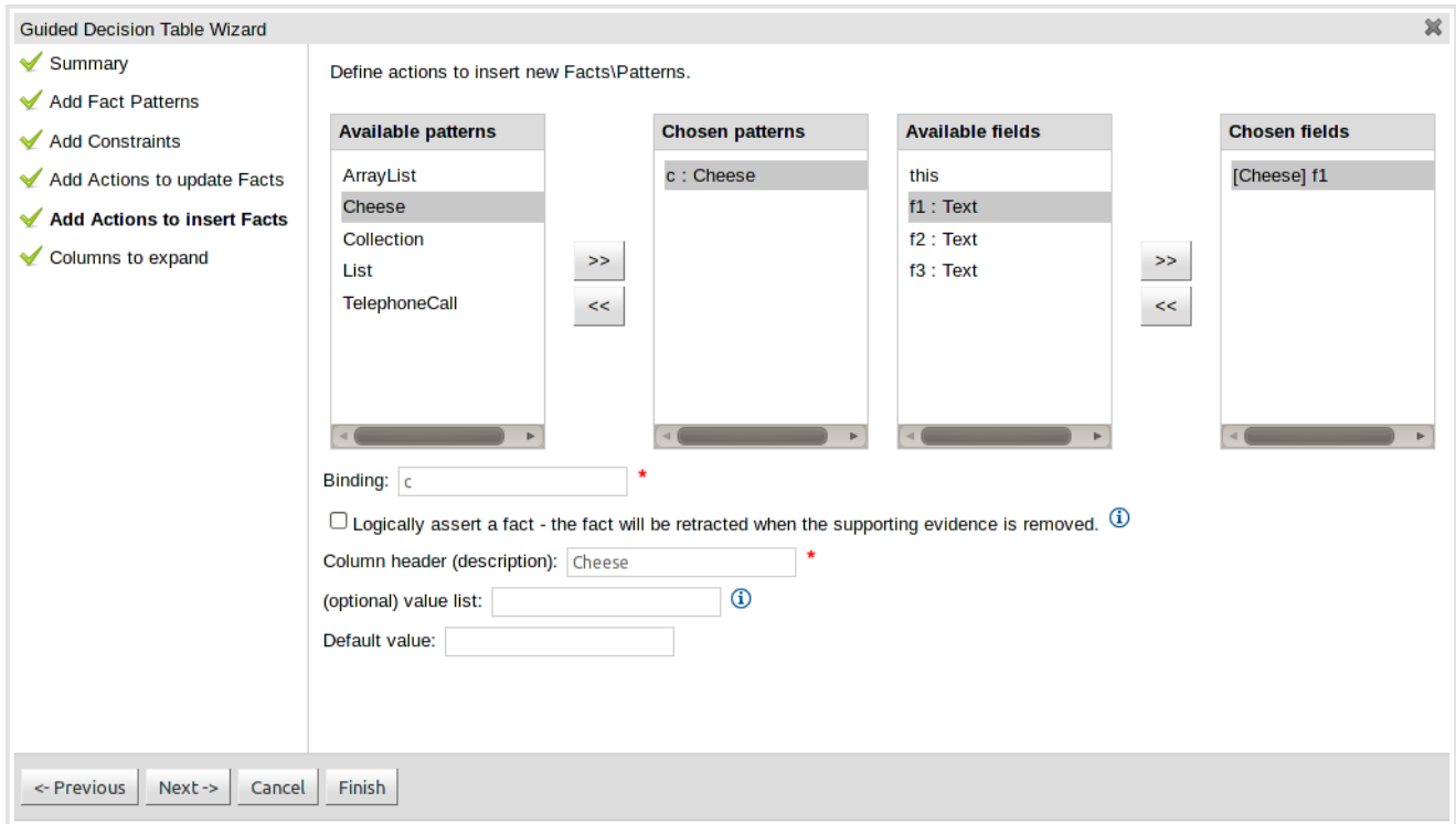
Figure 17.42. Add Actions to insert facts page
