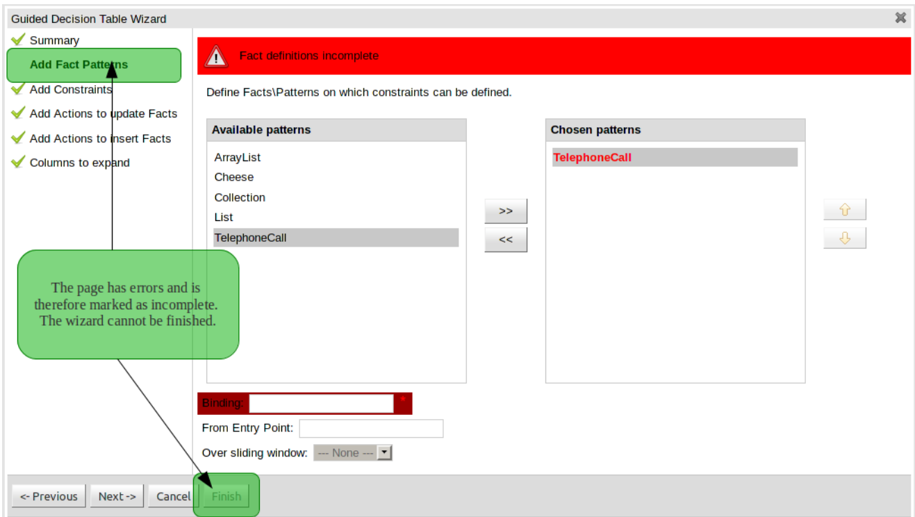
Figure 17.39. Example of an incomplete Fact definition
