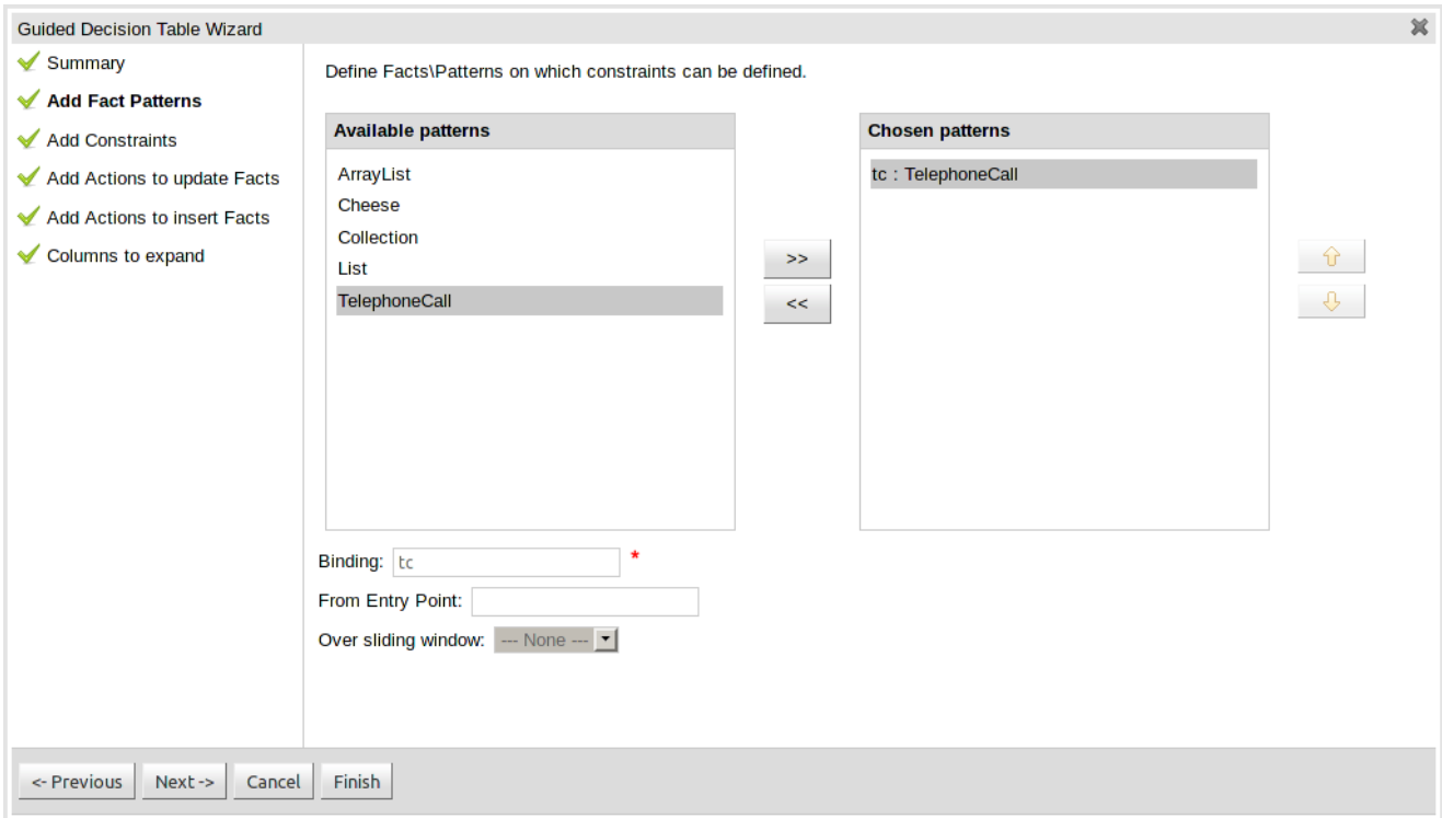
Figure 17.38. Add Fact Patterns page
