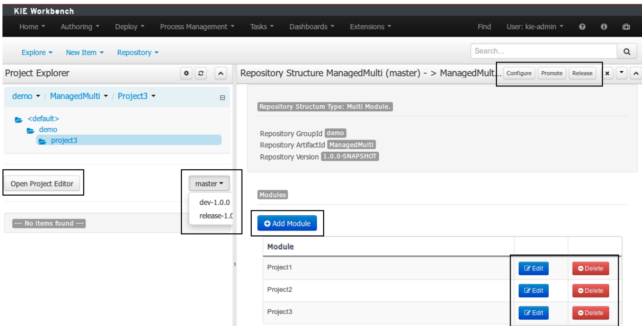
Figure 16.97. Managed Repositories Operations
