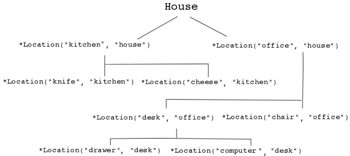
Figure 21.45. Transitive Reasoning Graph of a House
