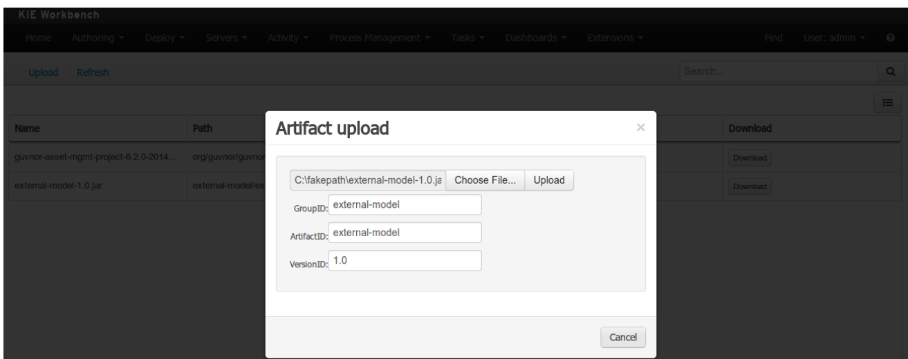
Figure 18.75. Enter GAV manually.
