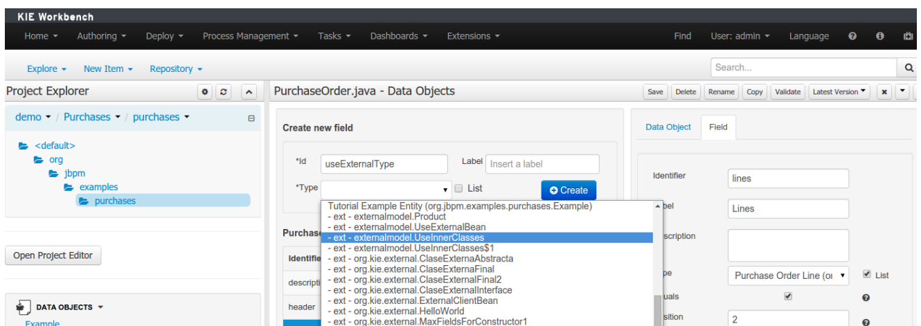
Figure 18.77. Identifying external objects.
