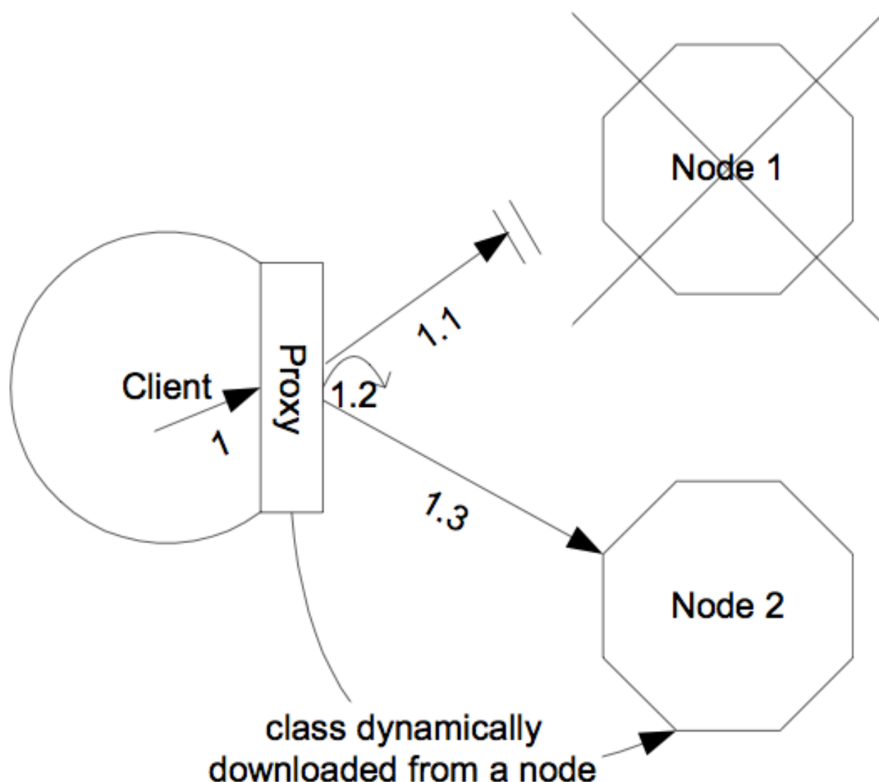
Figure 16.2. The client-side interceptor (proxy) architecture for clustering
