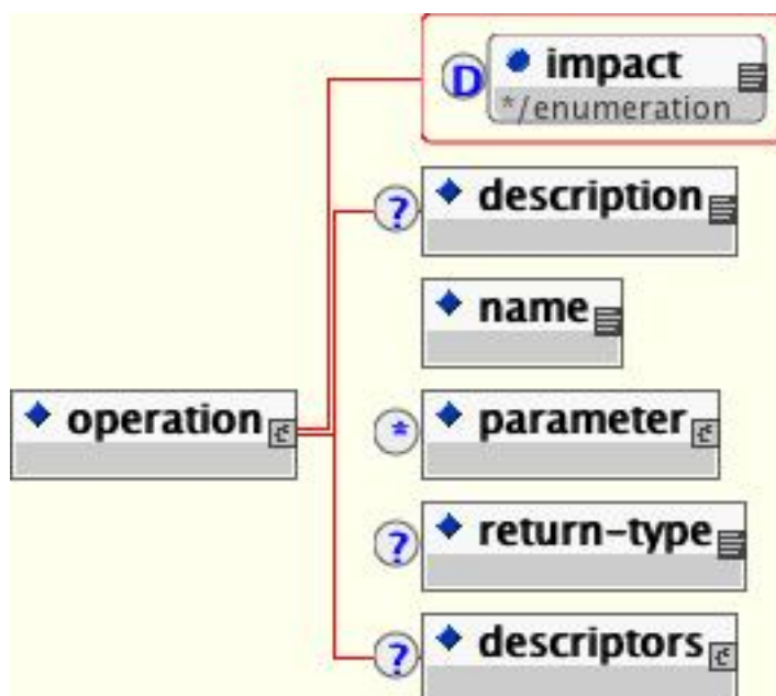
Figure 2.10. The XMLEBean operation element and its content model
