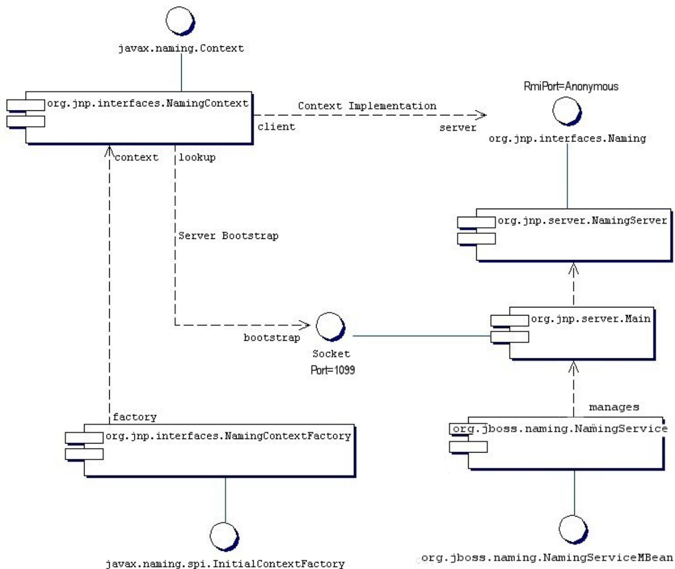
Figure 3.1. Key components in the JBossNS architecture.
