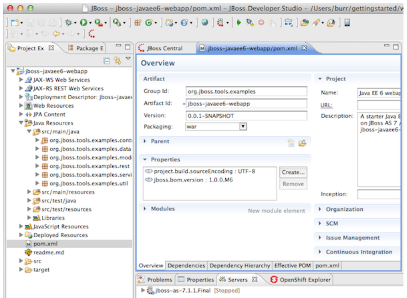
Figure 4.1: Project Explorer
