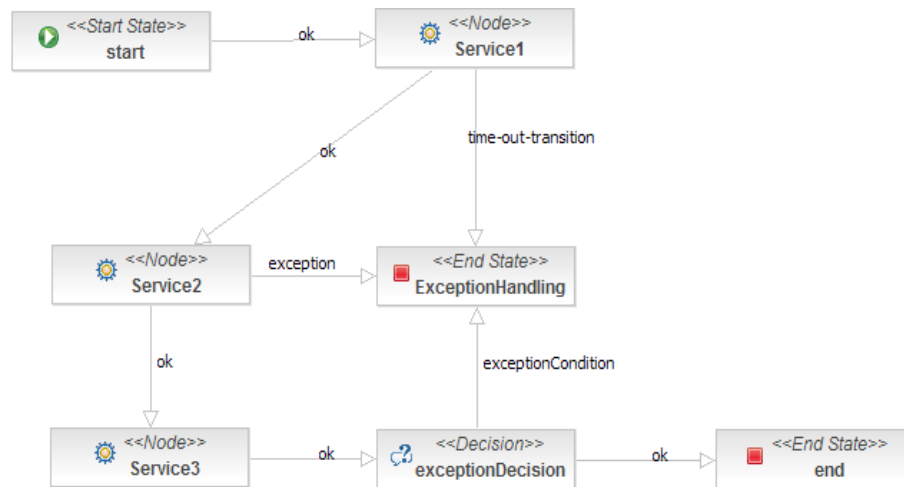
Figure 5. Three exception handling scenarios: time-out, exception-transition and exception-decision.
