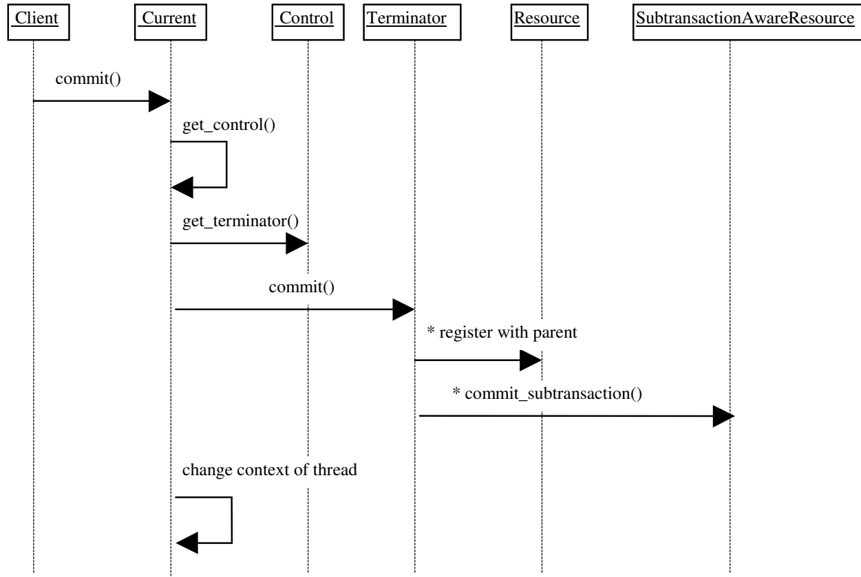
Figure 15: Subtransaction commit.
