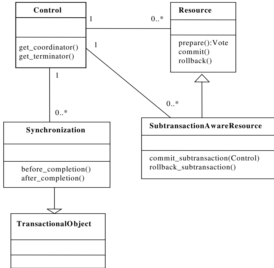
Figure 13: Transaction relationship.
