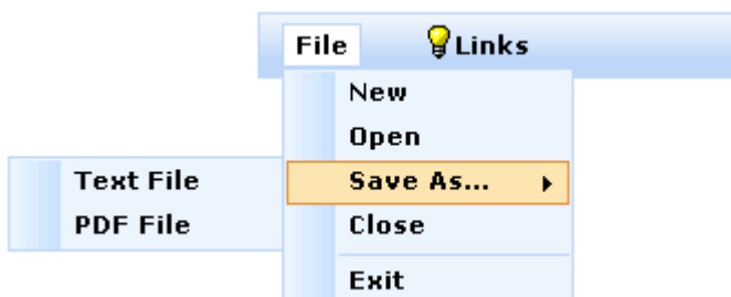
Figure 6.61. Using the "direction" attribute
