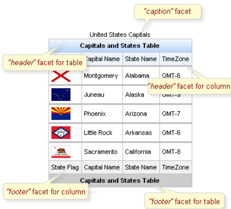
Figure 6.38. <rich:dataTable> component with facets
