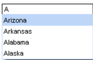
Figure 8.1. <rich:autocomplete>
