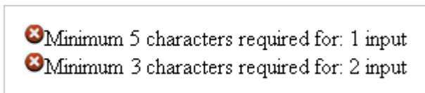
Figure 13.2. rich:messages component
