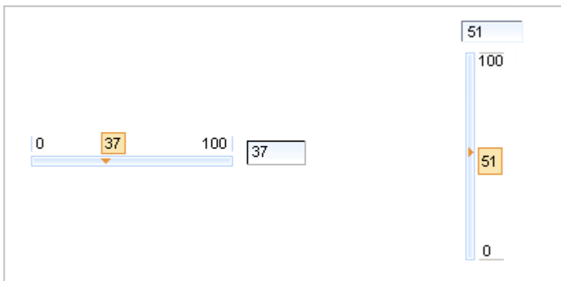
Figure 8.4. <rich:inputNumberSlider>
