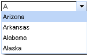
Figure 8.6. <rich:select>
