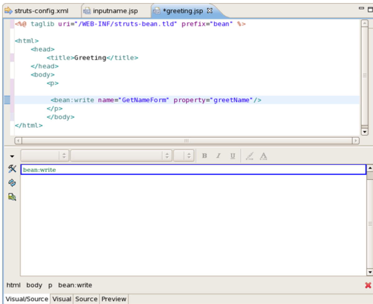
Figure 4.3. Editor Window
