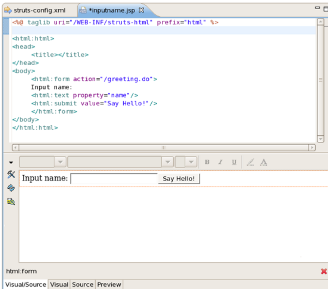
Figure 4.2. Editor Window
