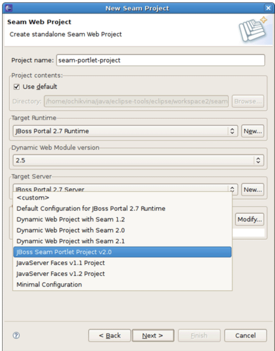
Figure 5.8. Project Facets
