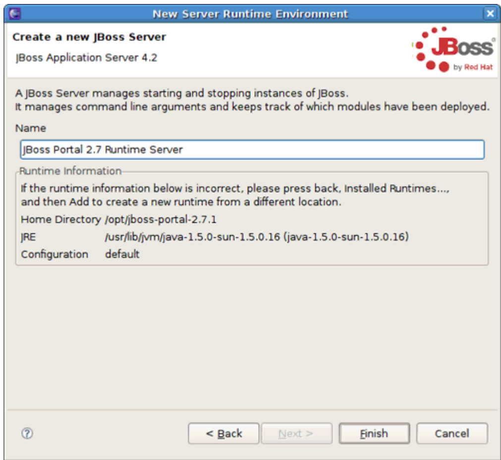
Figure 3.4. Target Server
