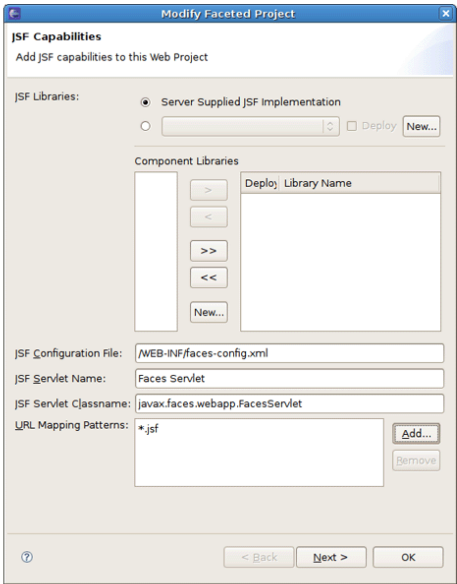
Figure 4.10. JSF Capabilities
