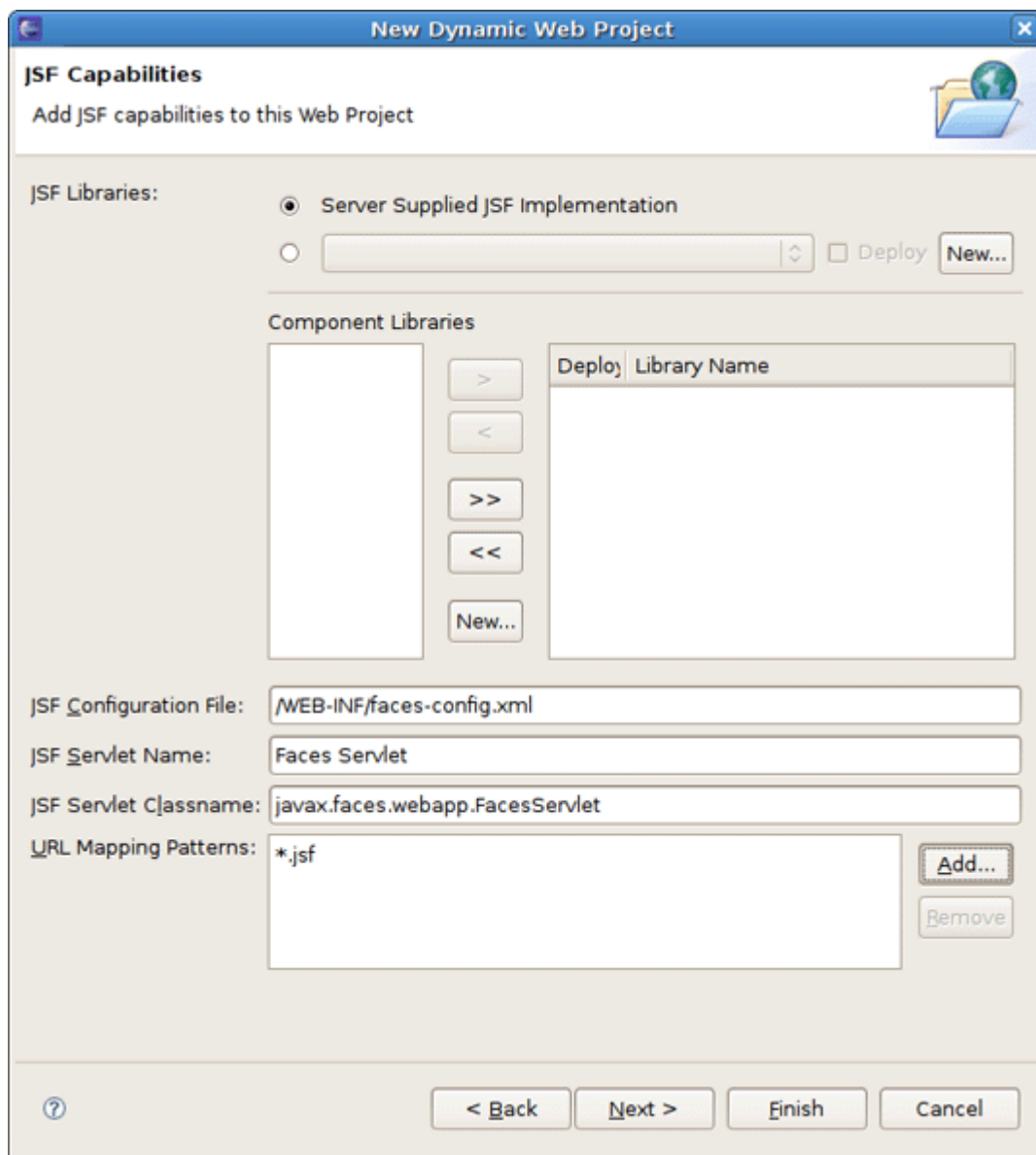
Figure 4.3. JSF Capabilities
