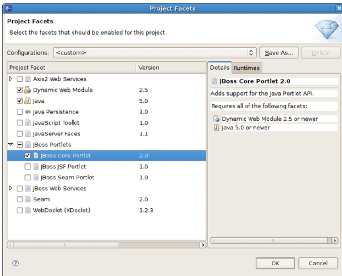
Figure 3.6. Enabling the Portlet Facet
