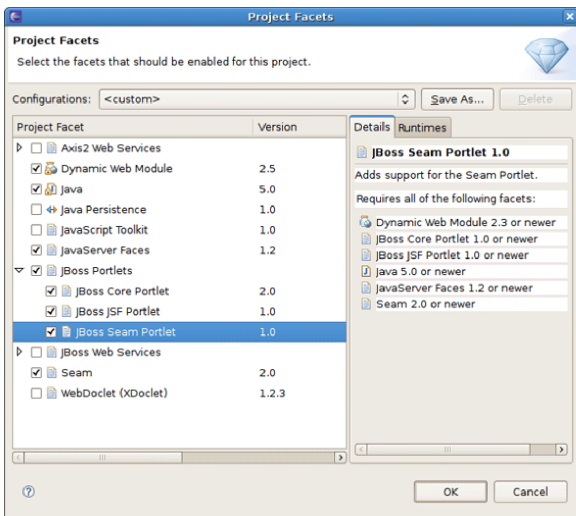
Figure 5.2. Project Facets
