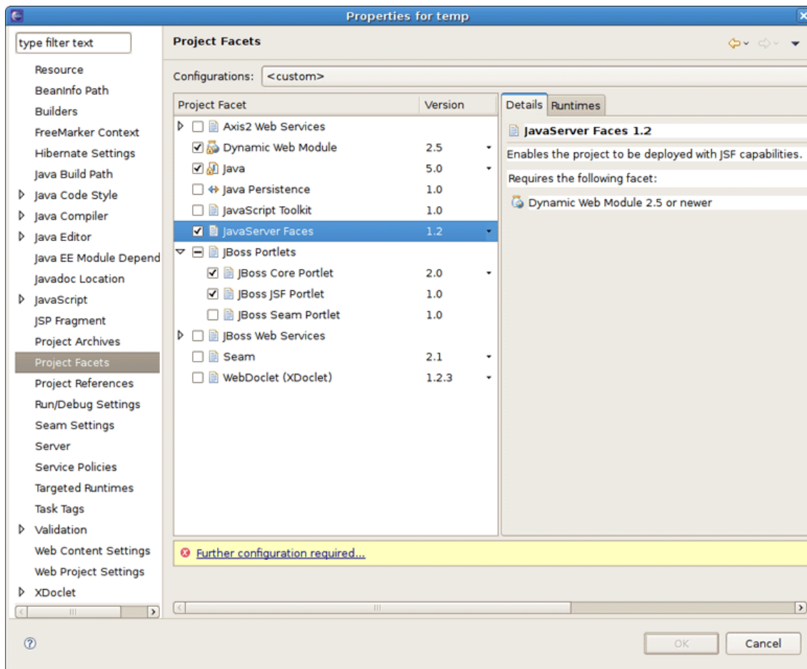
Figure 4.9. Project Facets
