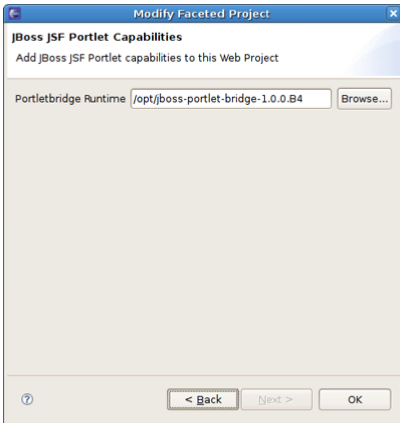
Figure 4.11. Project Facets
