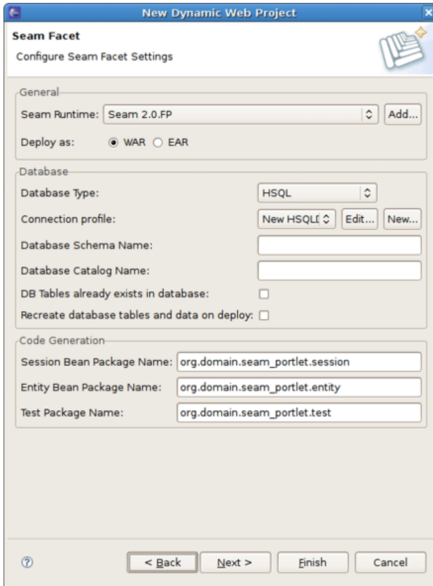
Figure 5.3. Seam Facet Settings
