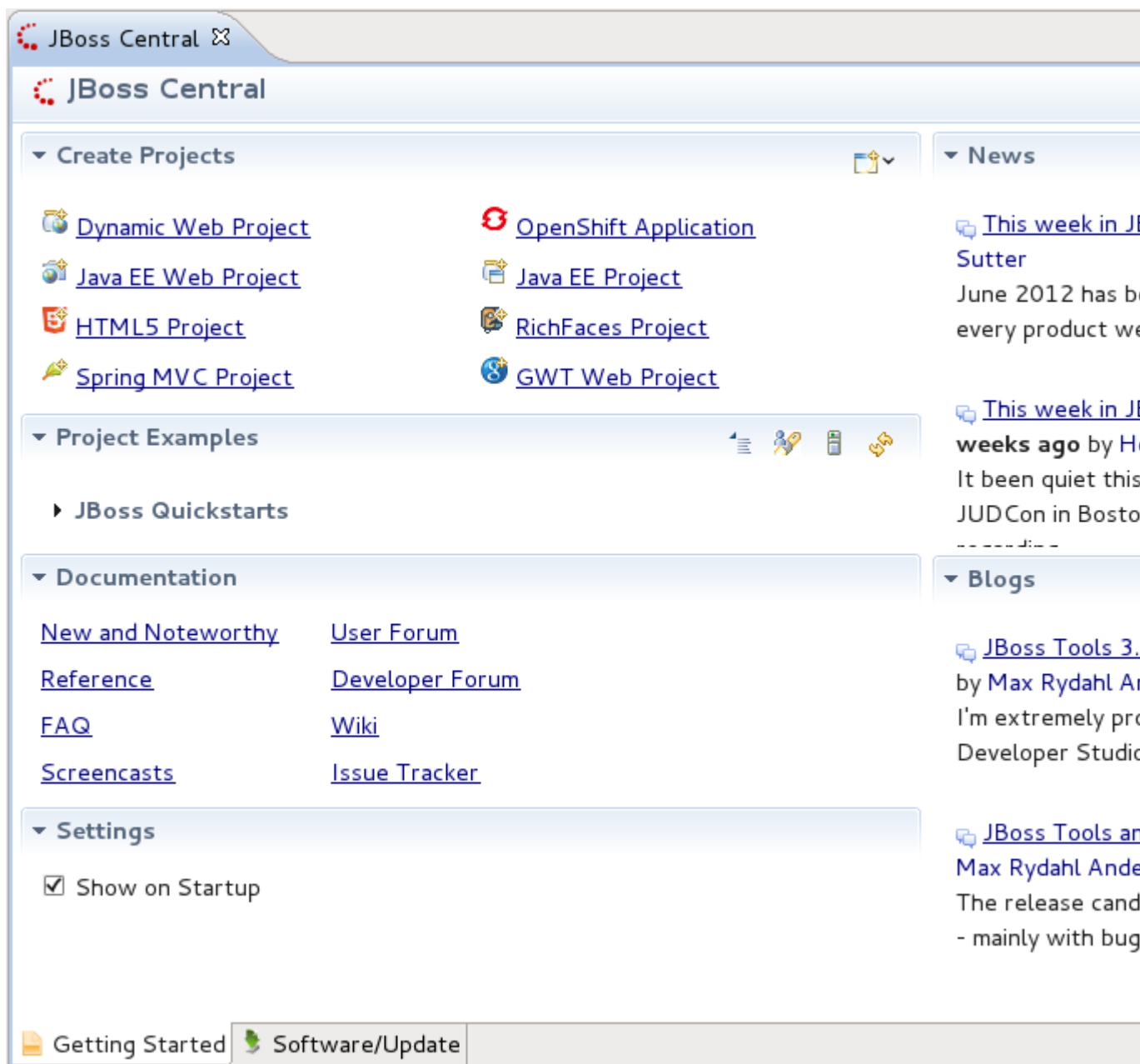
Figure 2.3. JBoss Central
