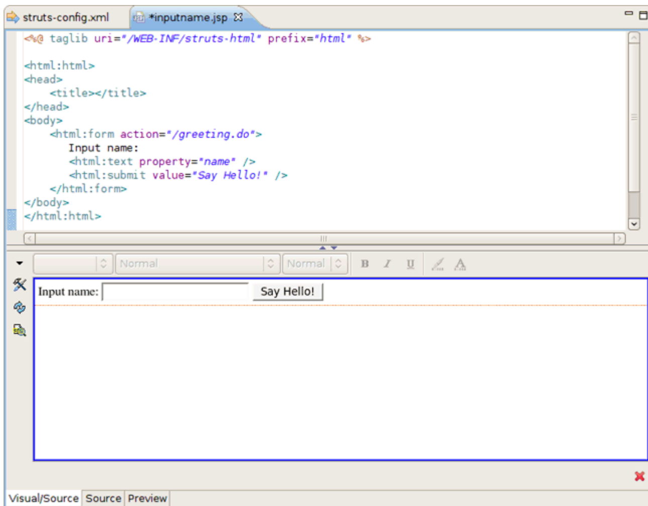
Figure 4.2. Editor Window
