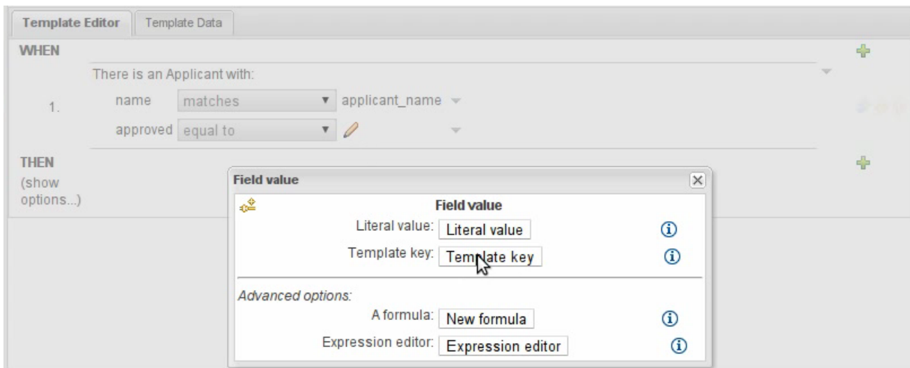
Figure 3.60. Adding a Template Key in the 'WHEN' Section
