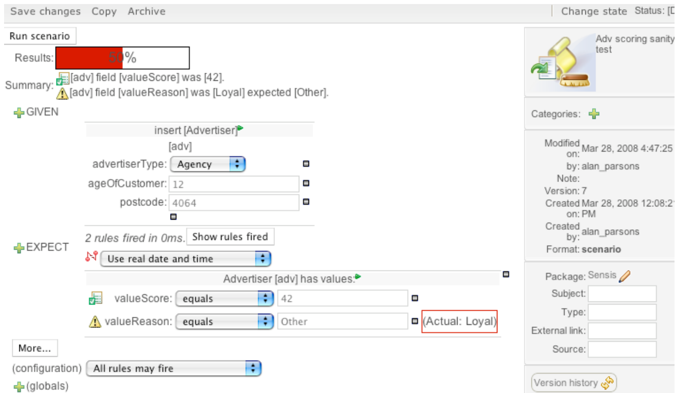
Figure 3.81. Running single scenario
