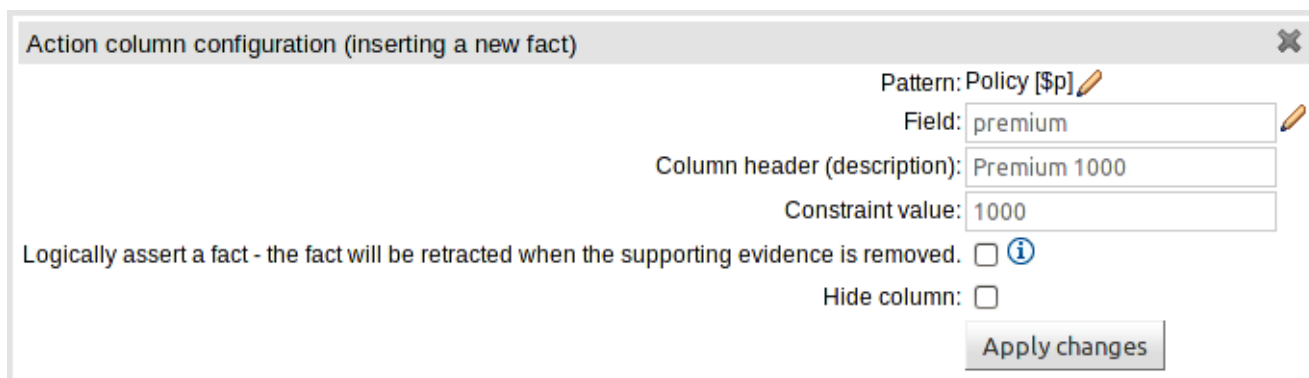
Figure 3.14. Editing an action in the editor
