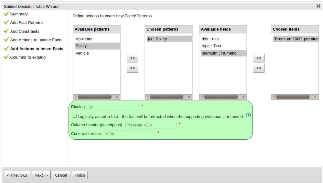
Figure 3.11. Defining Limited Entry actions with the Wizard
