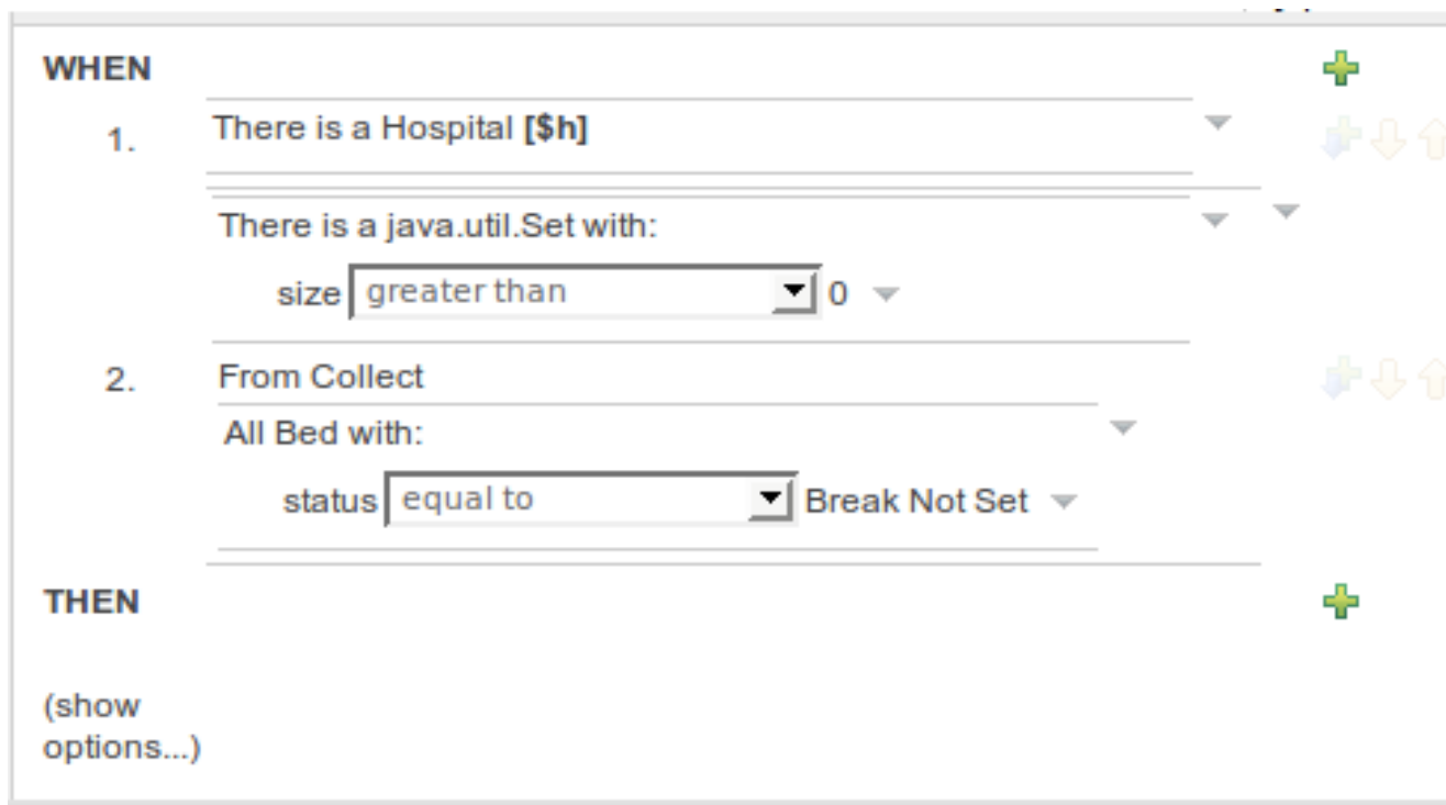
Figure 3.58. From Collect CE Builder
