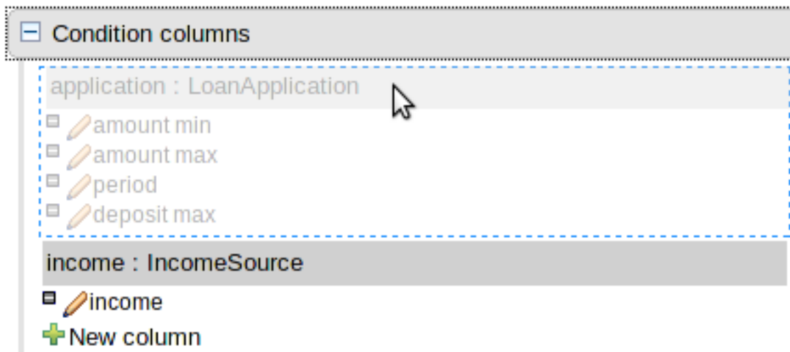
Figure 3.16. Re-arranging Condition patterns
