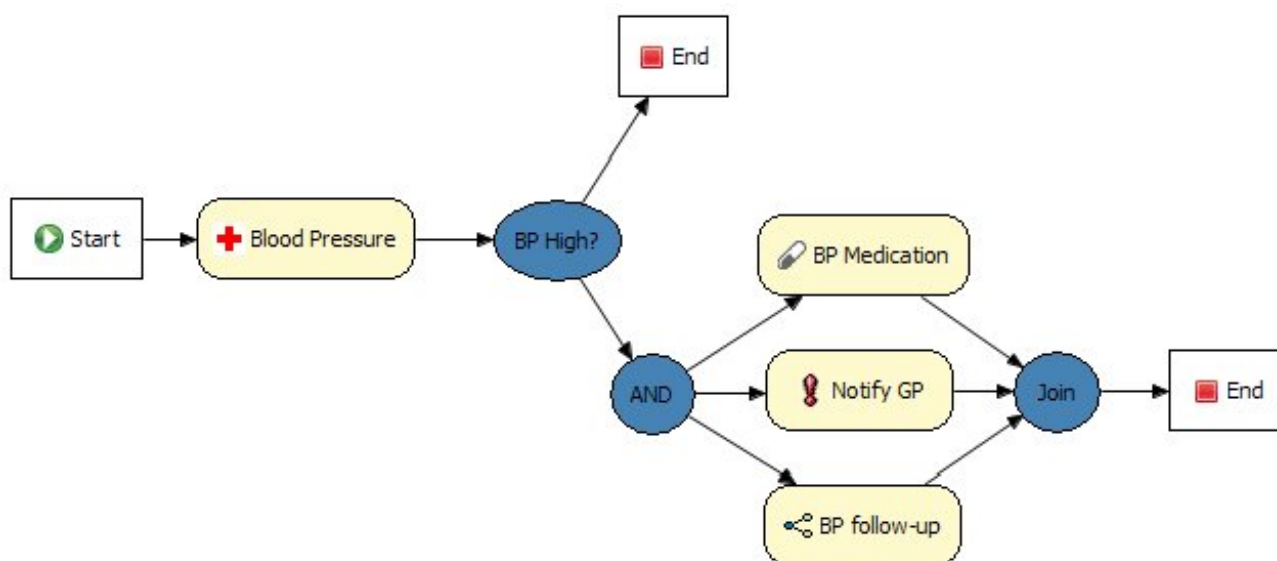
Figure 3.87. Work items
