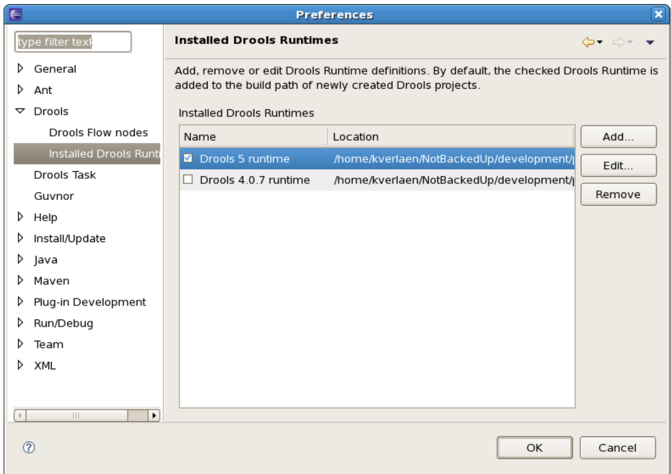
Figure 3.89. Run times
