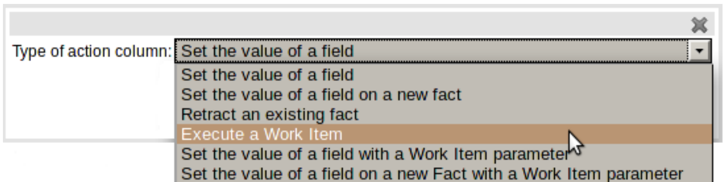
Figure 3.22. New Actions
