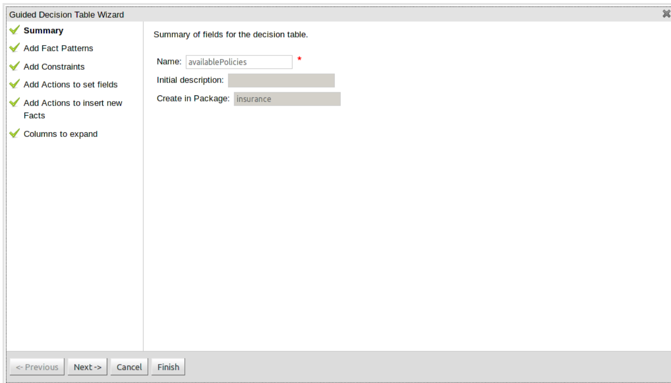
Figure 3.33. Summary page
