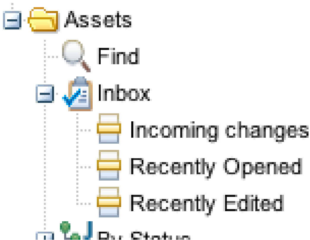
Figure 3.55. Inbox Categories
