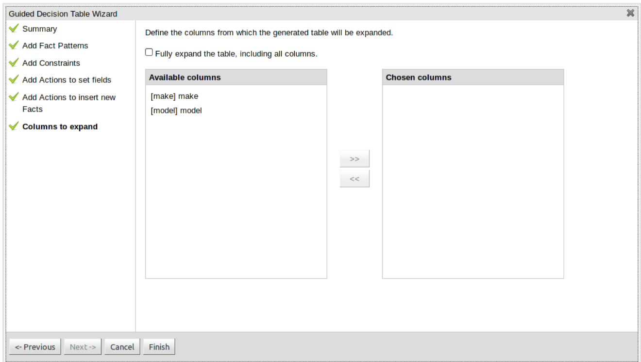
Figure 3.39. Choose how rows are created - select the columns you want to expand upon
