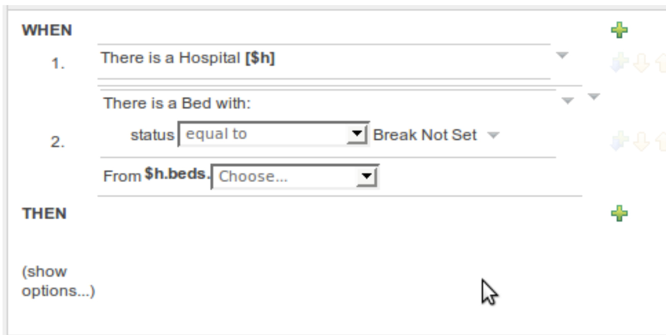
Figure 3.57. From CE Builder
