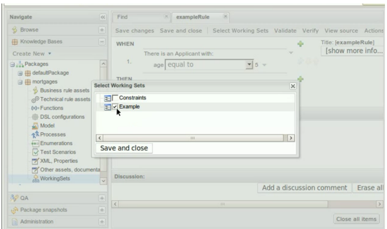
Figure 3.72. Select the working set to validate the age field
