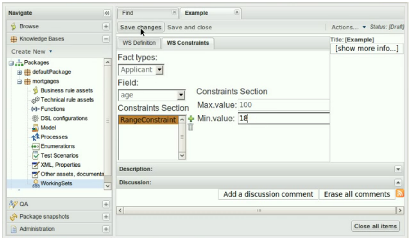
Figure 3.71. A example range constraint
