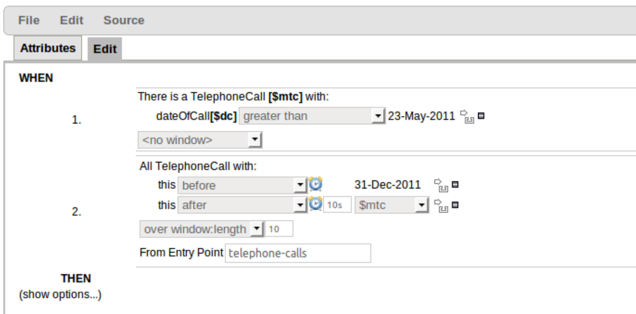
Figure 3.45. Complex Event Processing
