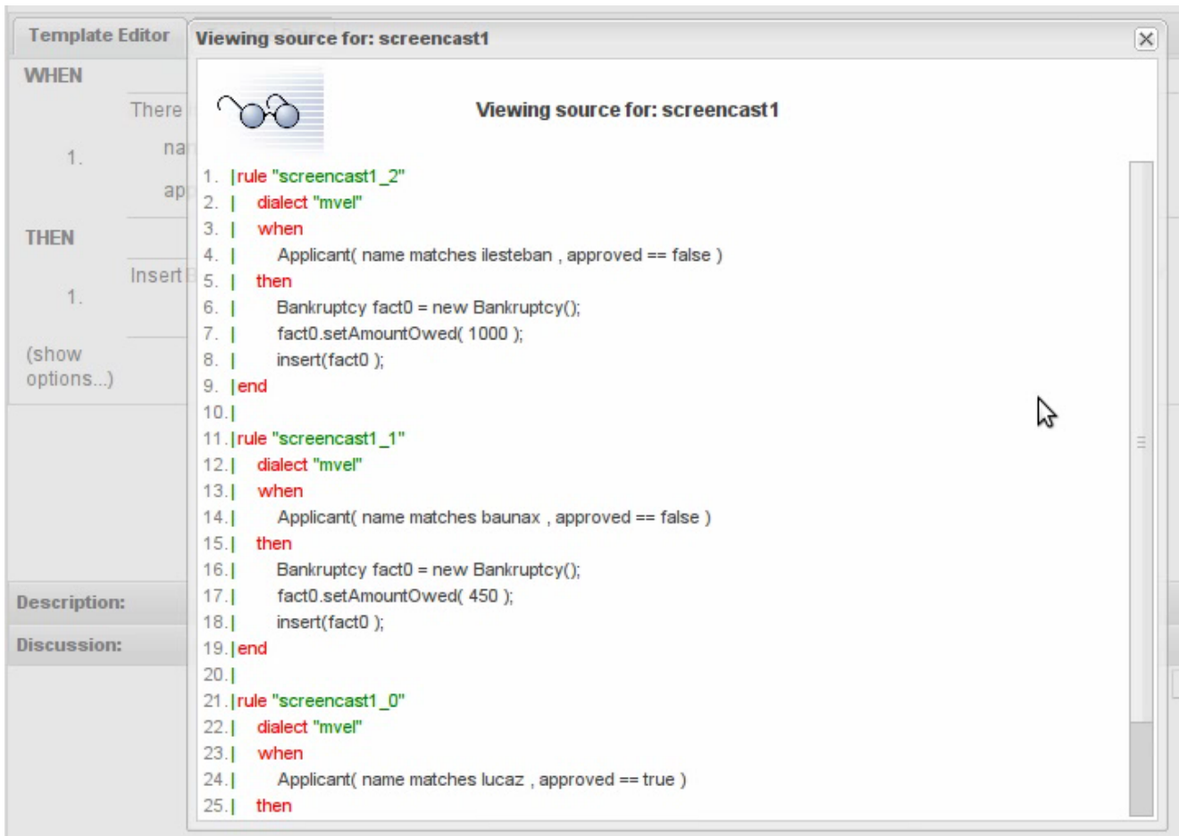
Figure 3.63. Each Row generates a Rule
