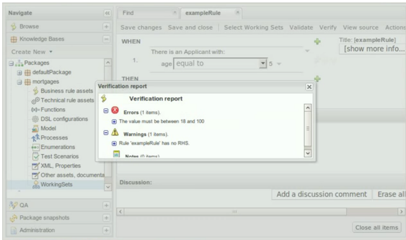
Figure 3.73. A age of 5 is invalid
