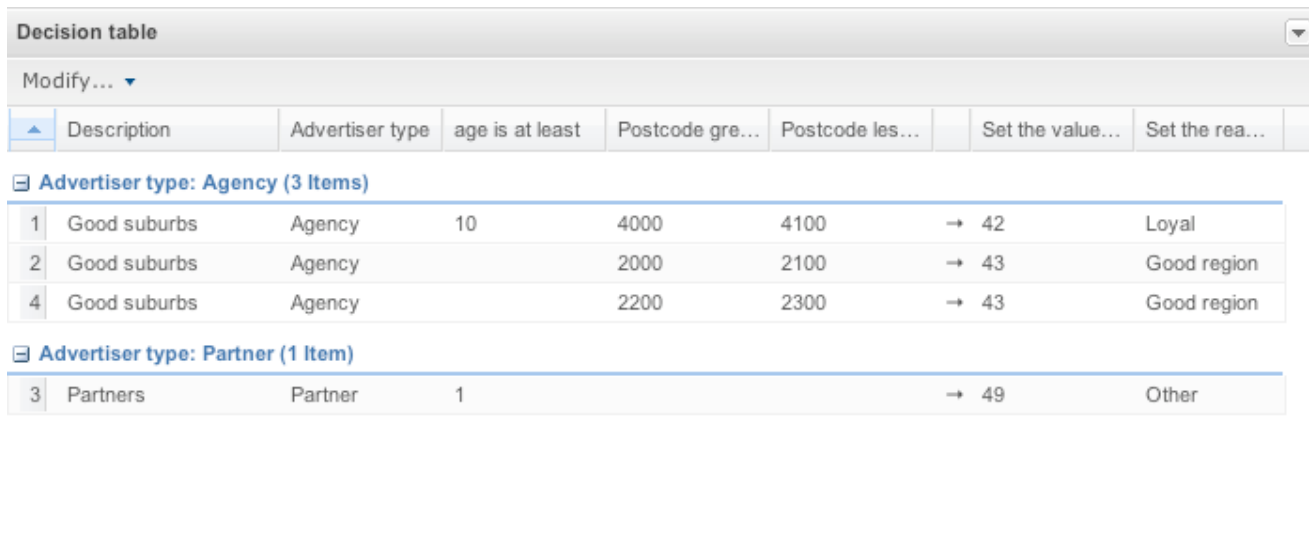
Figure 3.79. Web based decision table editor
