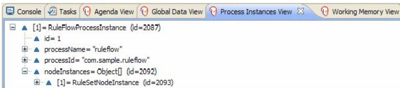
Figure 3.84. Rule Flow properties
