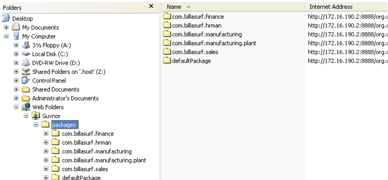
Figure 3.82. WebDAV
