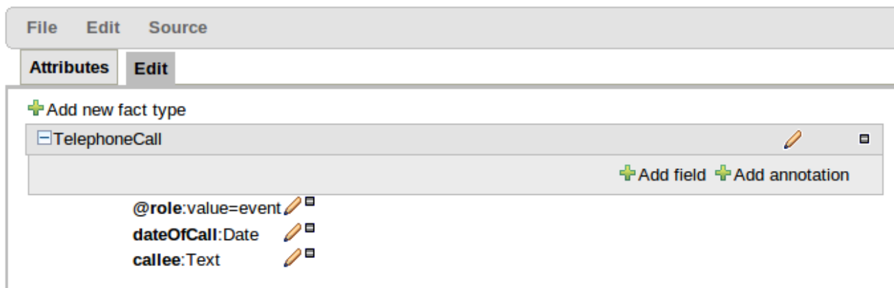
Figure 3.43. Annotations
