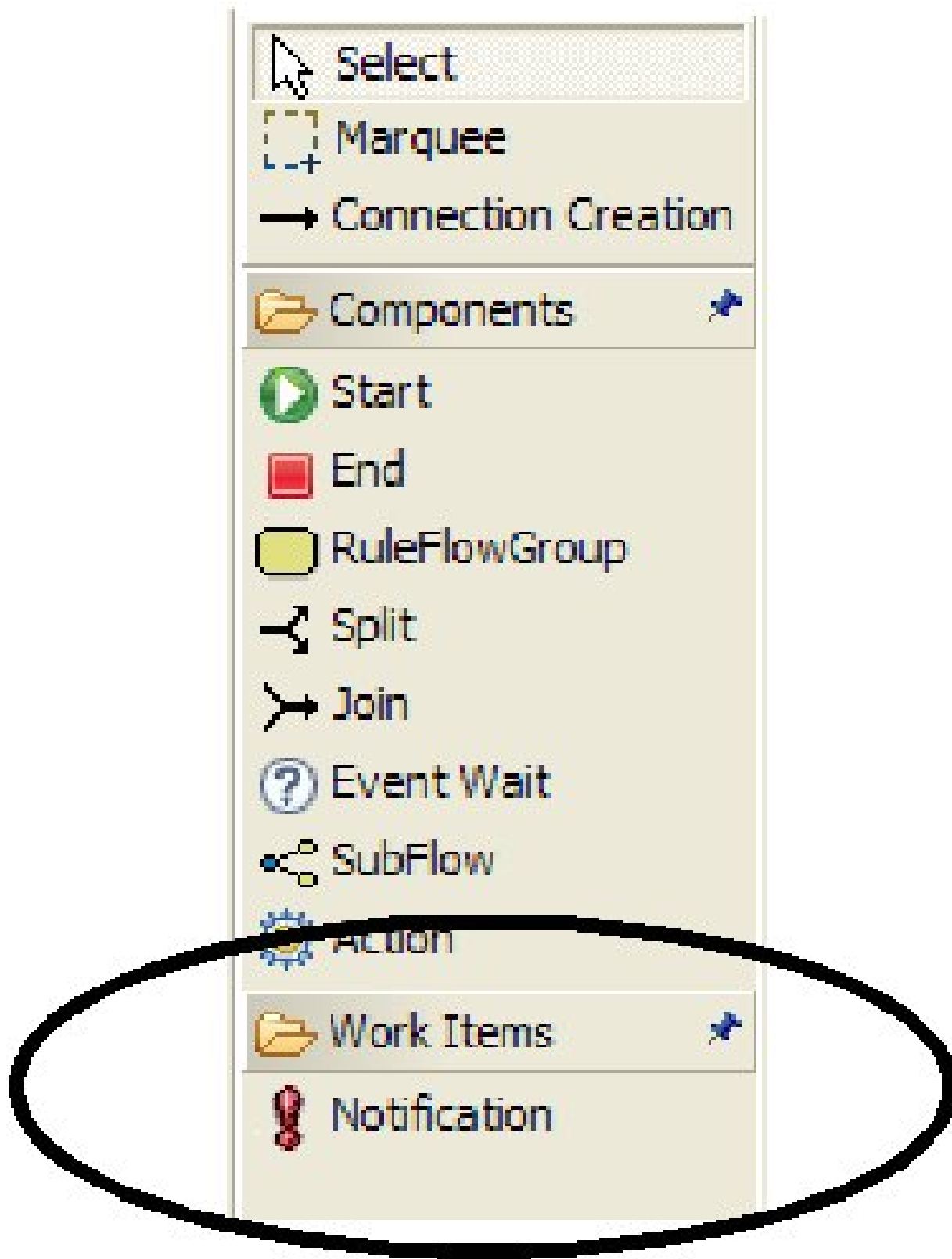
Figure 3.88. Notification
