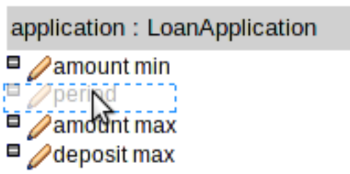
Figure 3.17. Re-arranging columns
