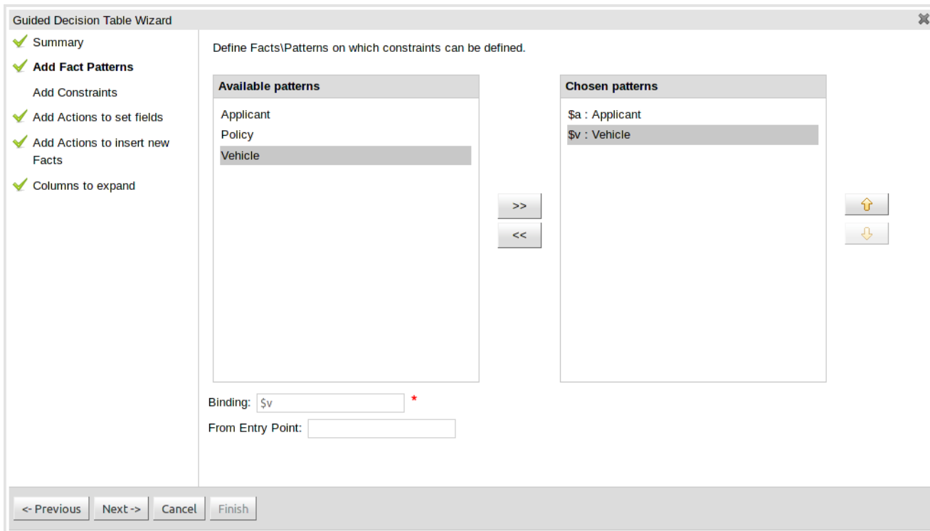
Figure 3.34. Add facts
