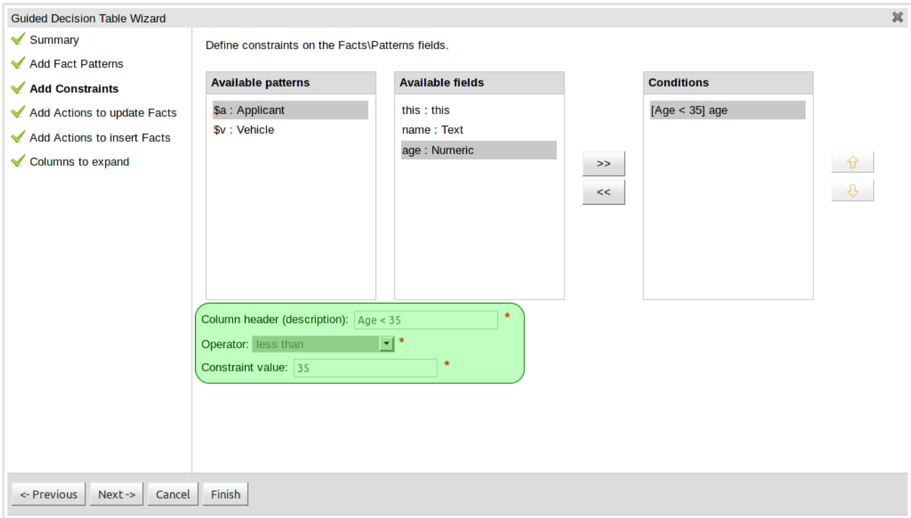
Figure 3.10. Defining Limited Entry constraints with the Wizard
