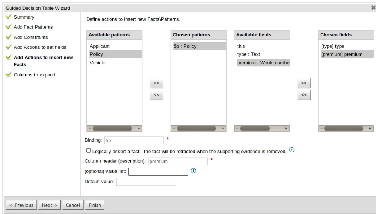
Figure 3.37. Add actions to insert new facts
