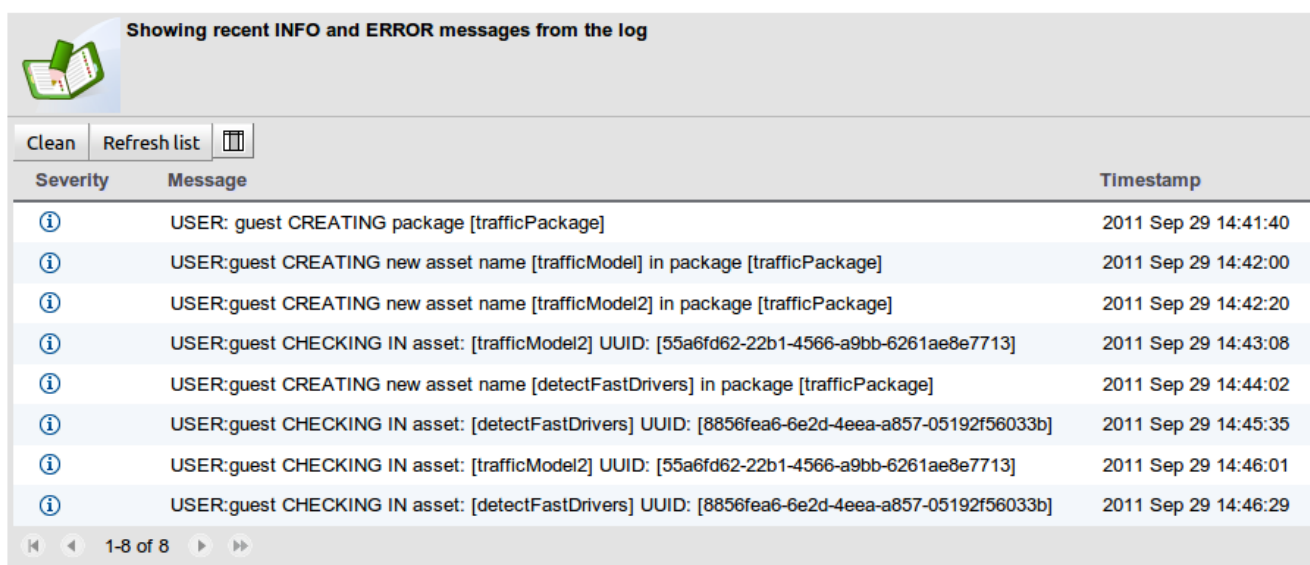
Figure 8.7. Event log
