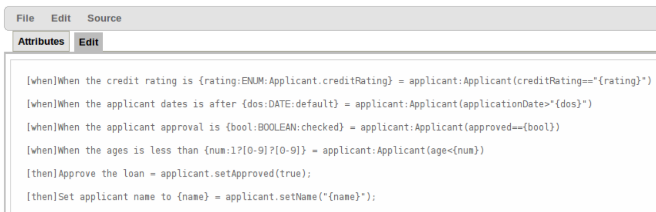
Figure 4.78. DSL rule
