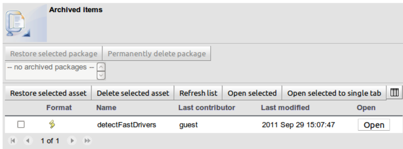
Figure 8.6. Archived items
