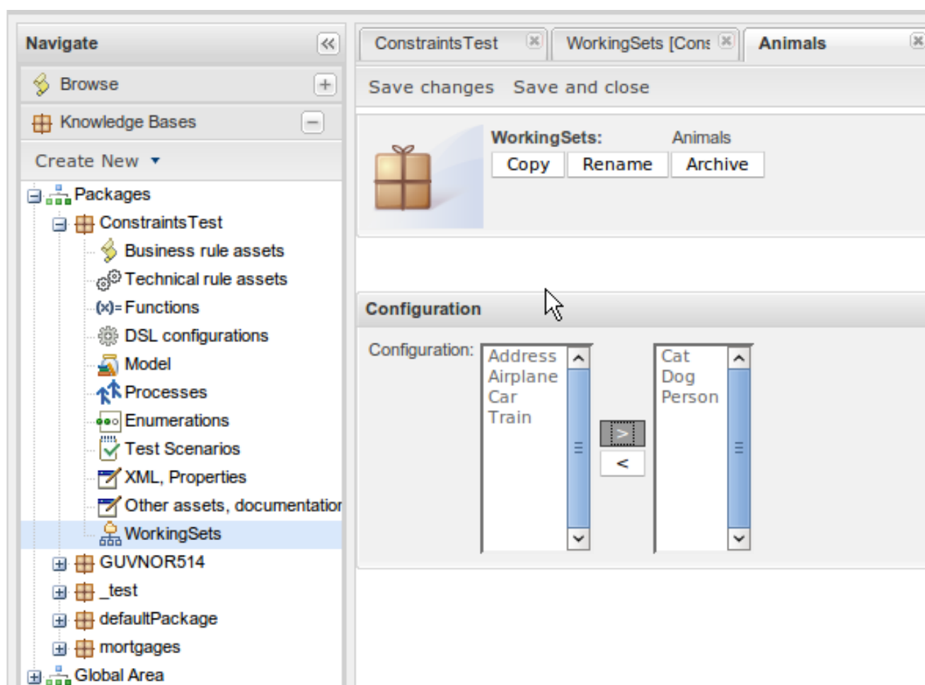
Figure 4.74. Create Animals Working Set
