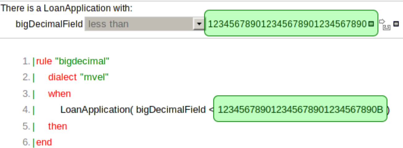
Figure 4.29. Example of using a BigDecimal
