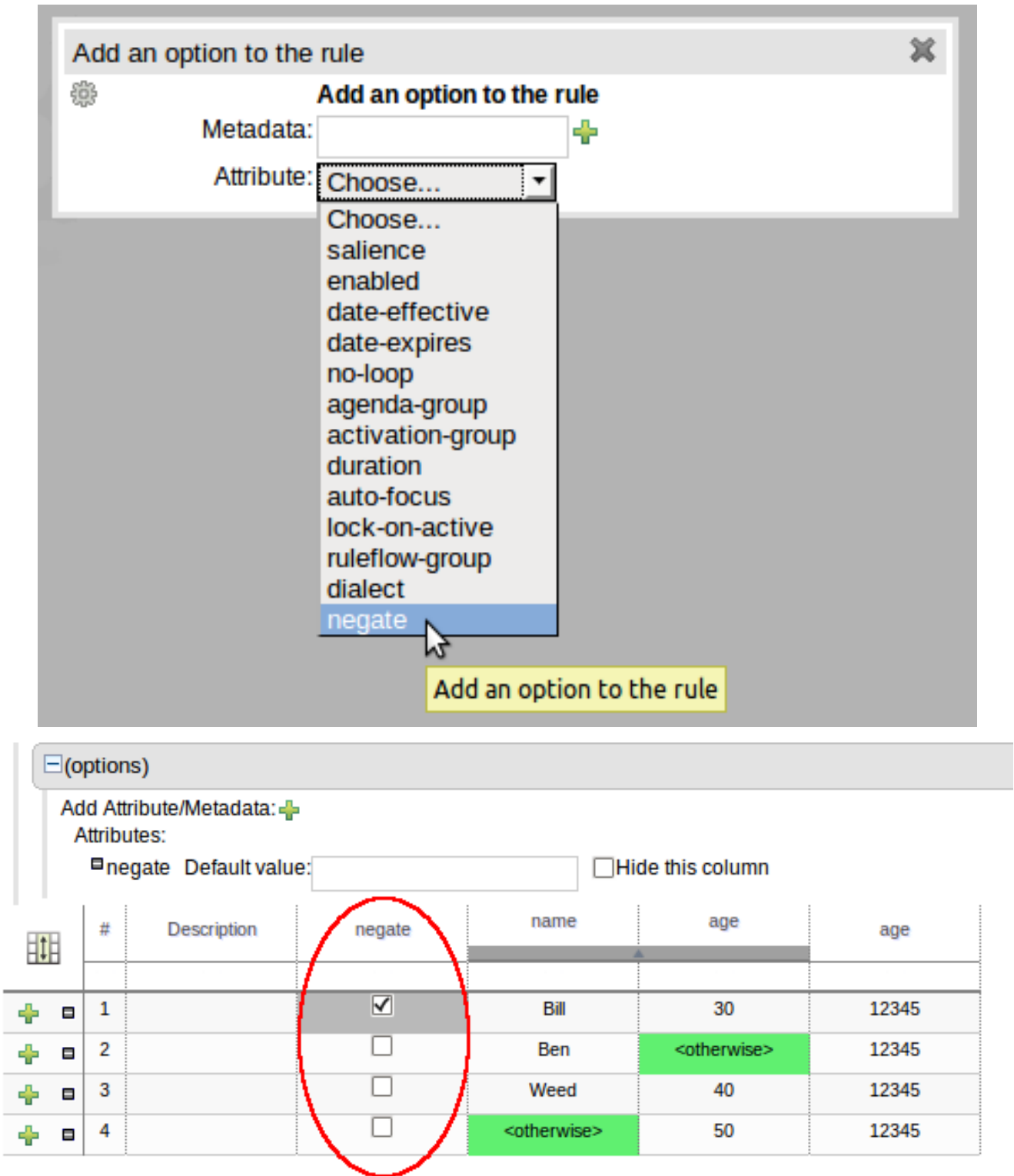
Figure 4.60. Negation of rules
