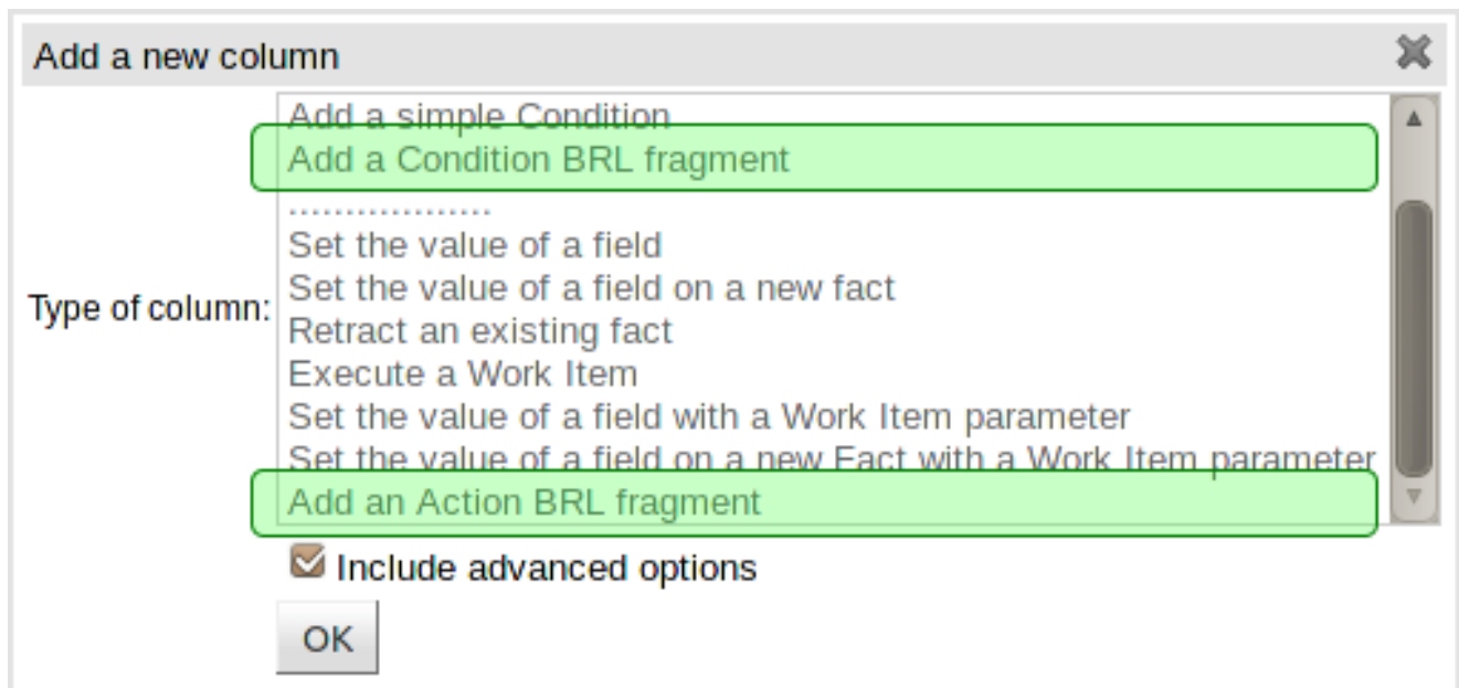
Figure 4.18. Adding a BRL fragment
