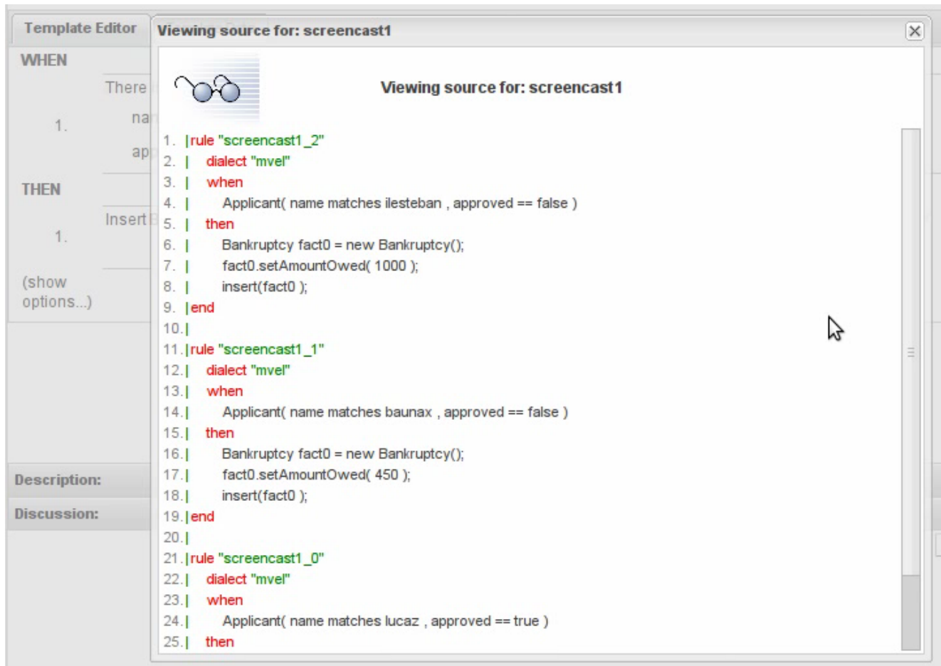
Figure 4.72. Each Row generates a Rule
