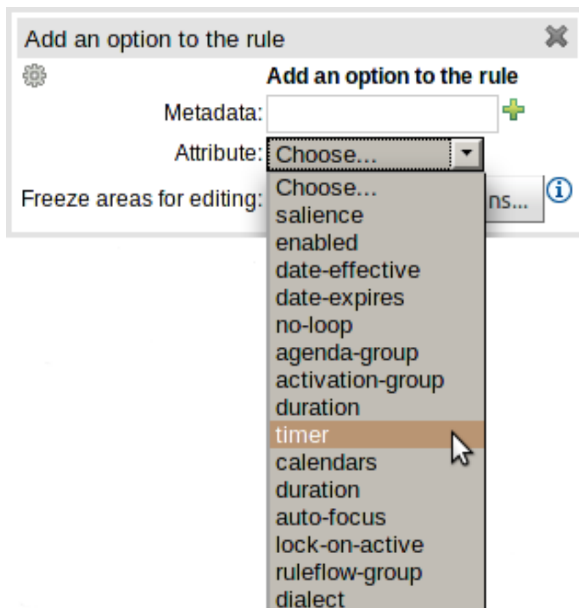
Figure 4.25. Timer and Calendar
