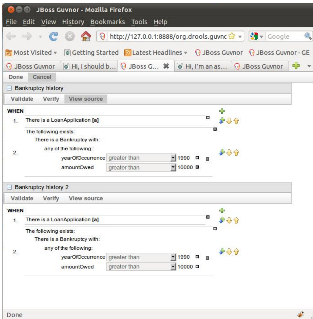
Figure 10.1. Embedded Editor with 2 BRL Rules
