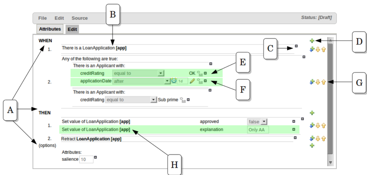
Figure 4.20. The guided BRL editor
