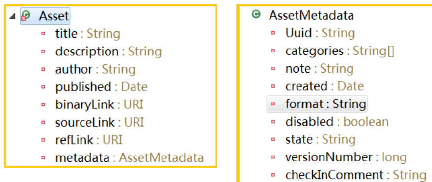
Figure 9.3. UML representation of the Asset Object
