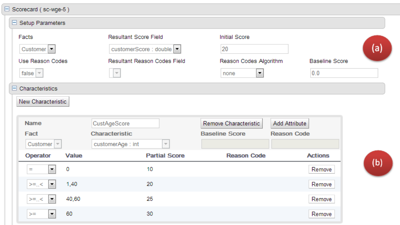
Figure 16.47. Scorecard Asset - Guided Editor
