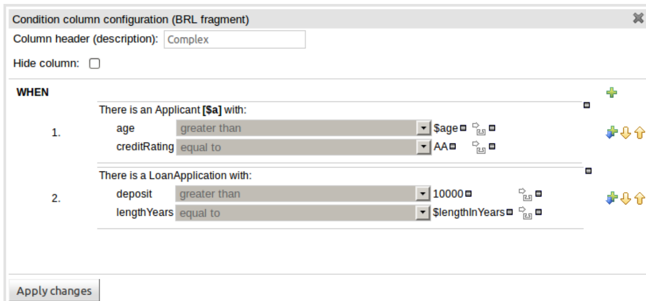
Figure 16.29. Defining a Condition with BRL
