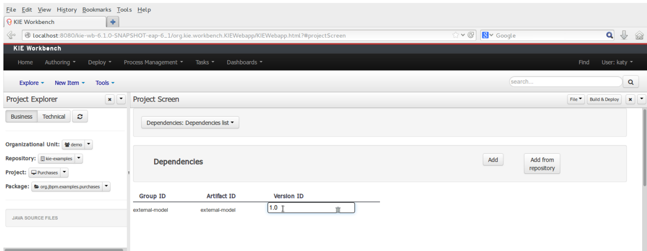
Figure 15.66. Dependency line edition.
