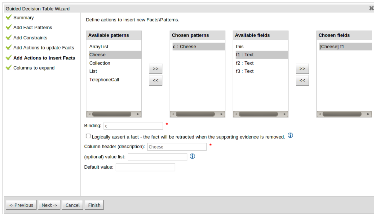
Figure 16.39. Add Actions to insert facts page
