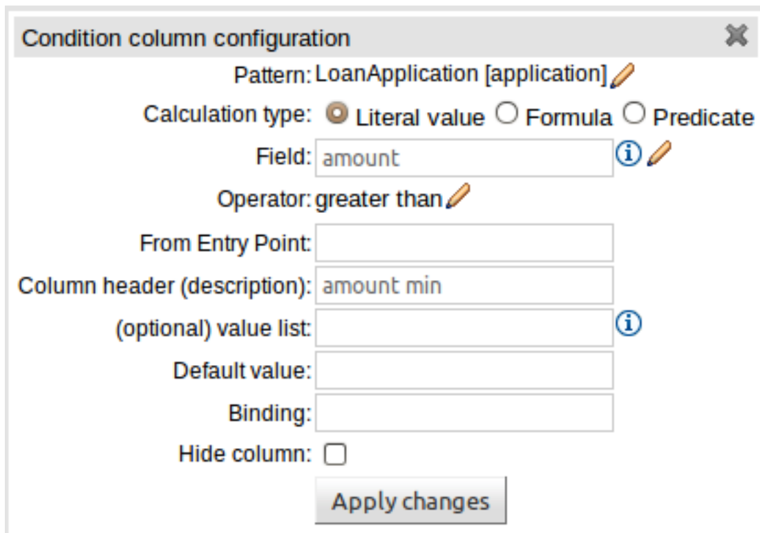
Figure 16.25. Simple Condition popup
