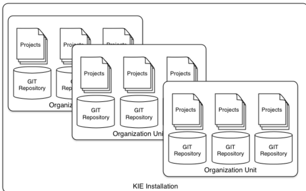
Figure 4.26. Installation Overview
