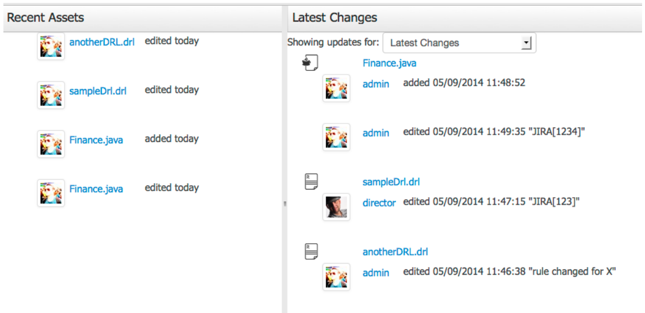
Figure 2.37. Timeline Perspective
