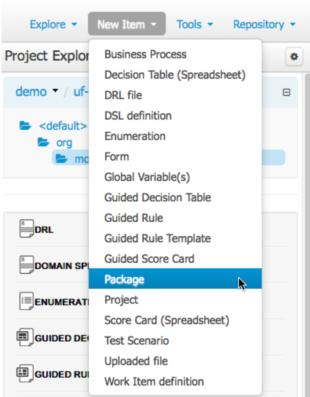
Figure 19.1. New Package
