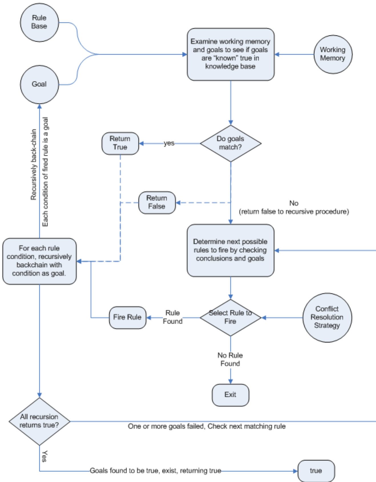
Figure 5.3. Backward Chaining
