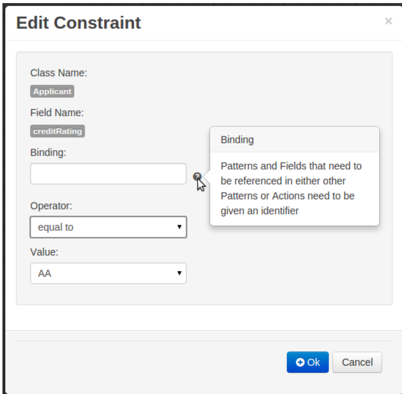
Figure 19.54. Guided Decision Trees - Field Constraint Editor
