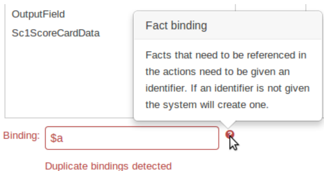
Figure 2.28. New Guided Decision Table Wizard validation
