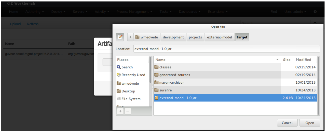
Figure 18.91. File browser.
