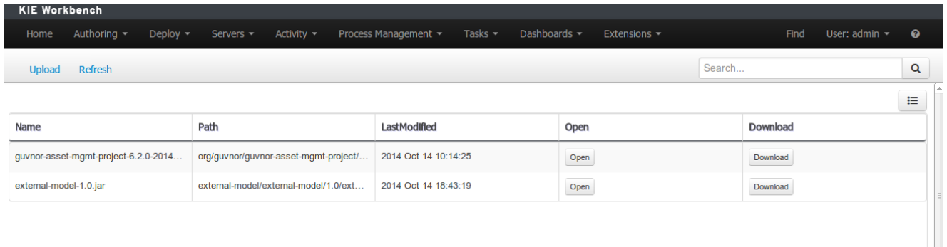
Figure 18.93. Files list.
