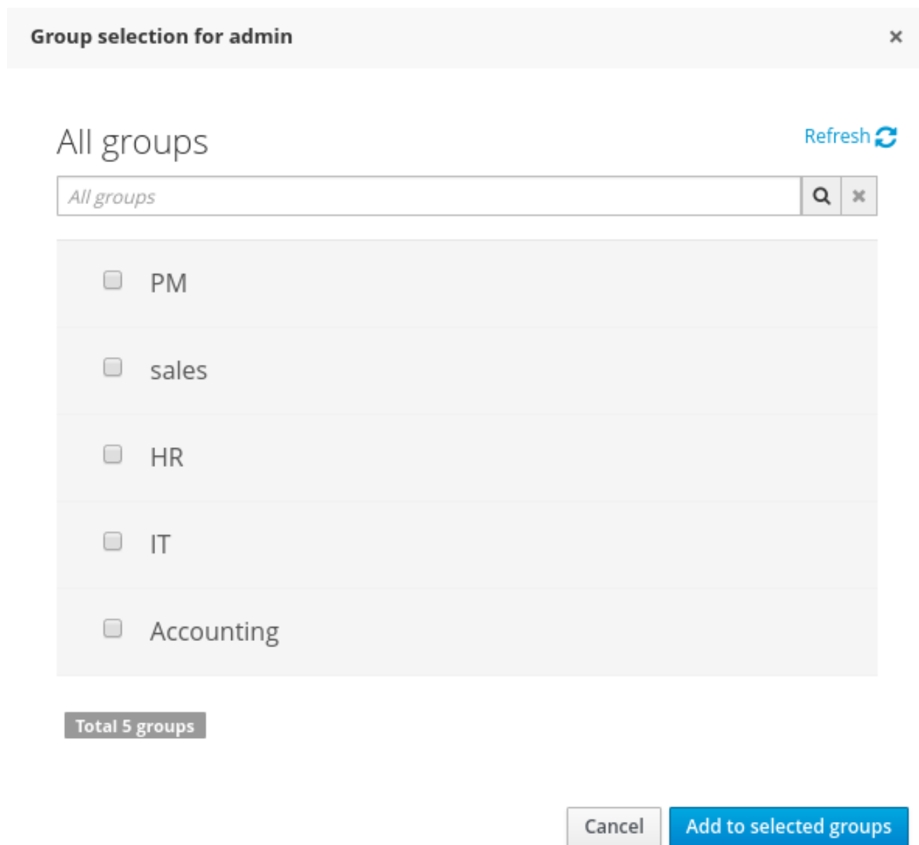
Figure 18.126.
