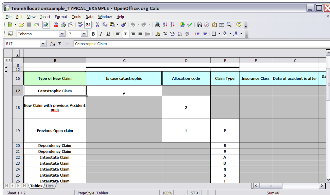
Figure 6.13. Using OpenOffice.org
