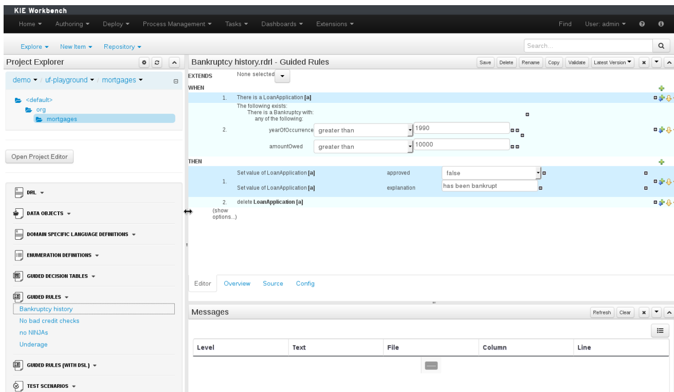
Figure 18.20. Resizing
