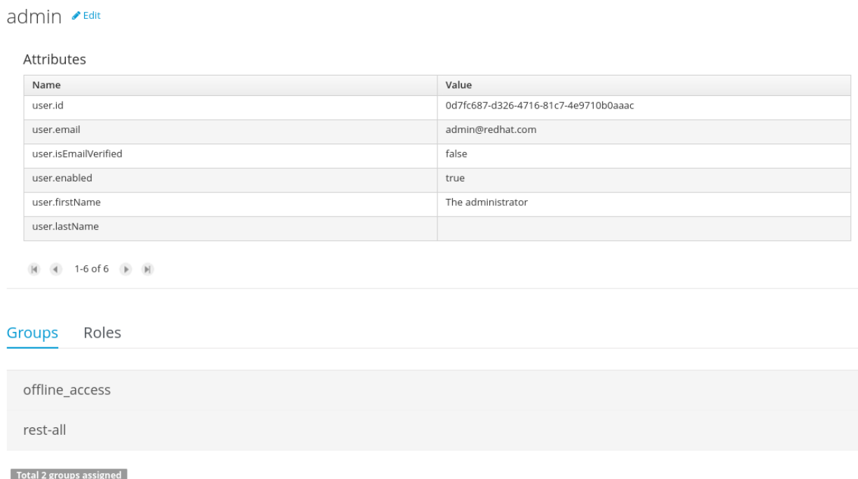
Figure 18.123.
