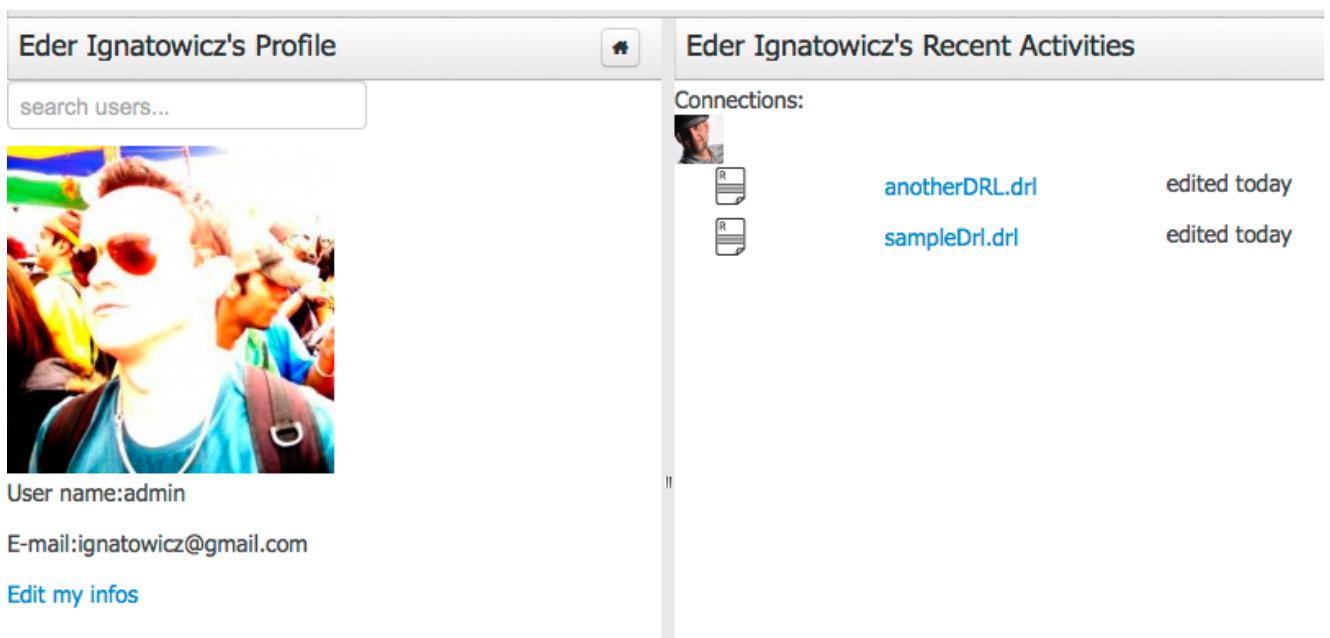
Figure 2.38. People Perspective
