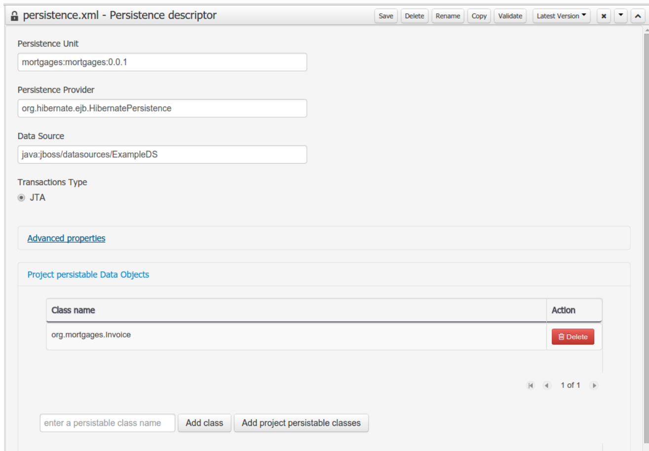
Figure 2.24. Persistence configuration
