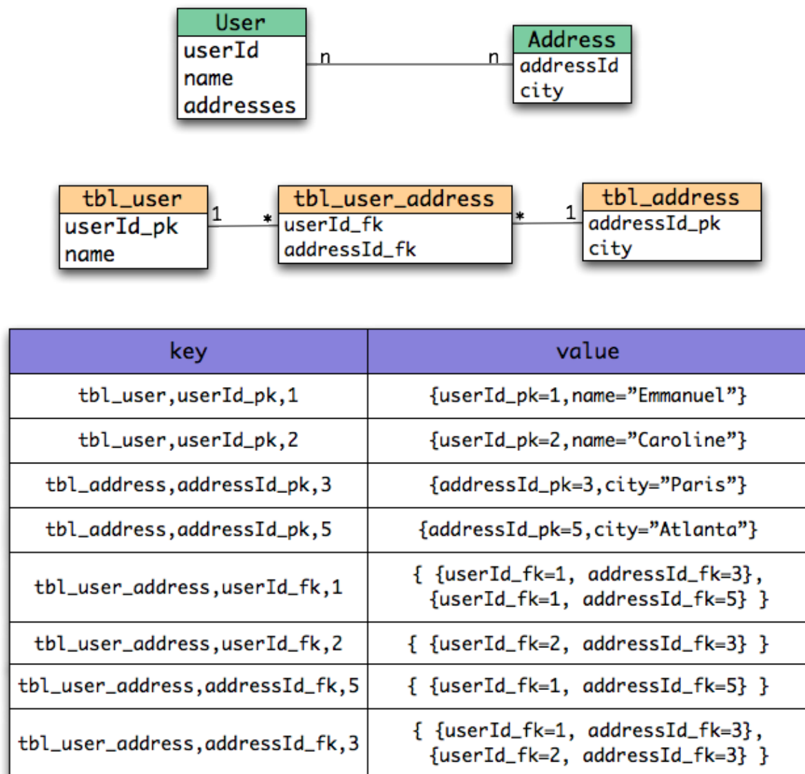
Figure 4. Storing associations
