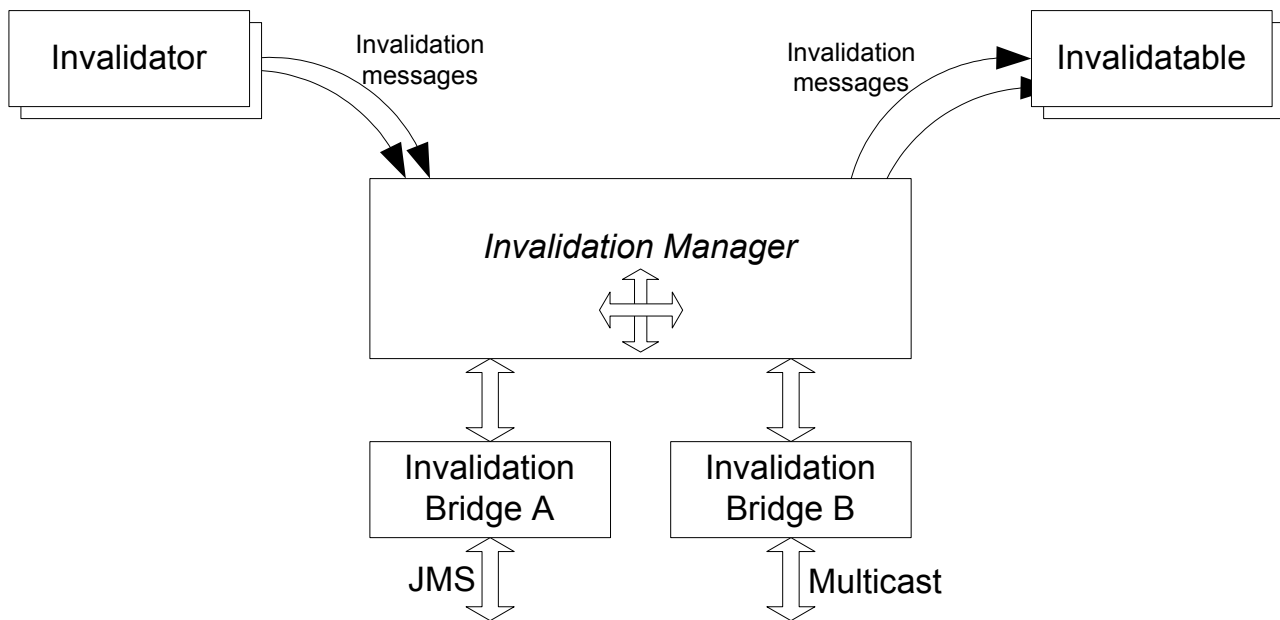
Figure 10 Cache Invalidation Framework Architecture
