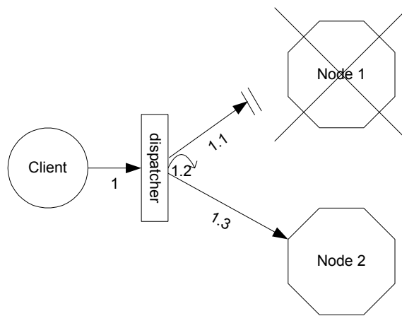
Figure 5. Dispatcher-managed fail-over
