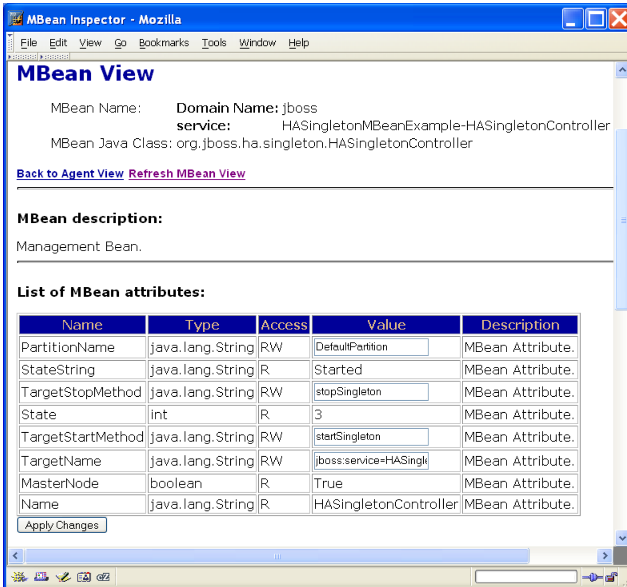
Figure 19. Controller MBean View. “MasterNode” is True on only one of the nodes
