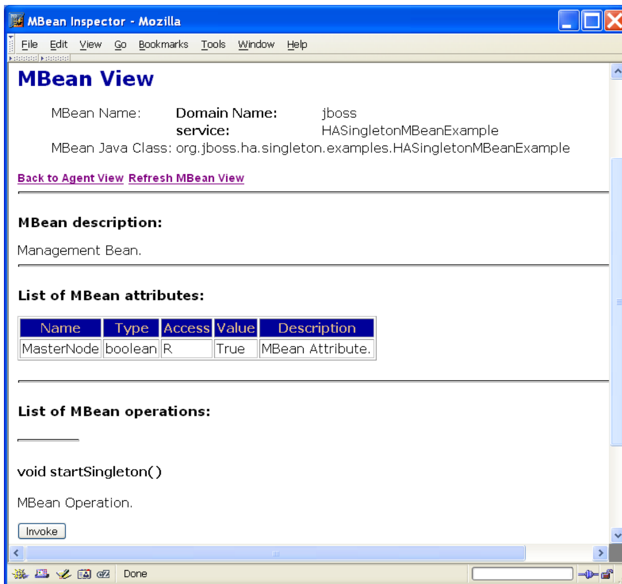
Figure 20. Sample singleton MBean View. “MasterNode” has the same value as “MasterNode” on the controller MBean
