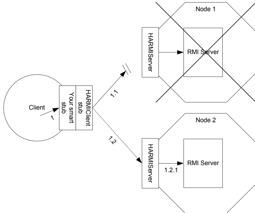
Figure 17. HARMIServer coupled with a pre-existing smart stub
