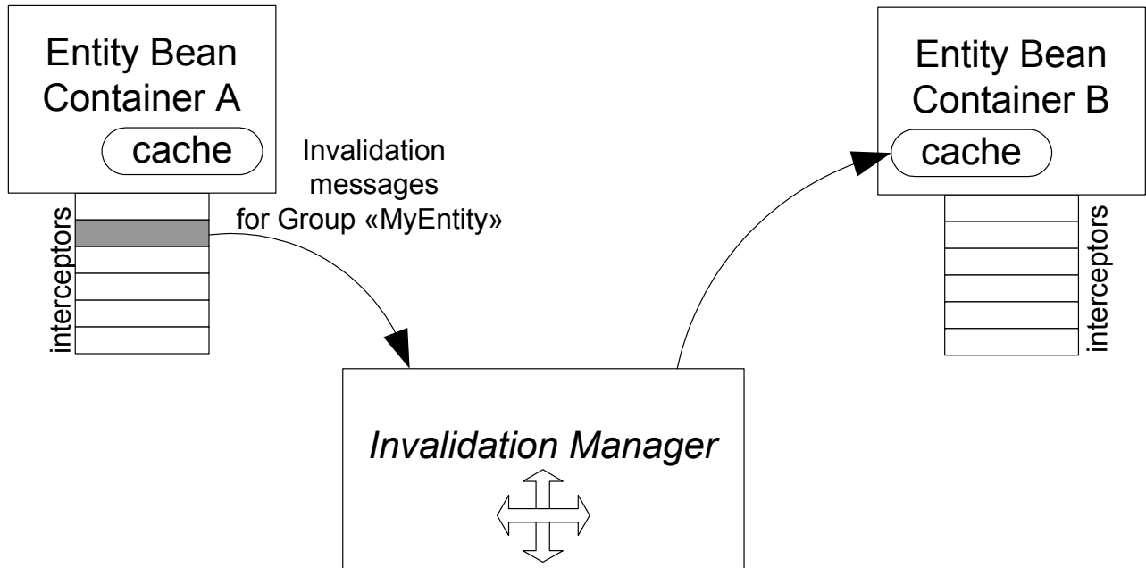
Figure 11 Cache Invalidation Framework Integration in EJB
