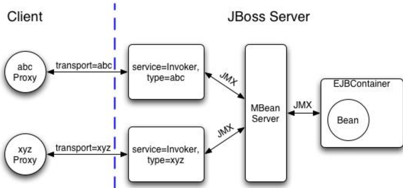
Figure 5.3. The transport invoker server side architecture
