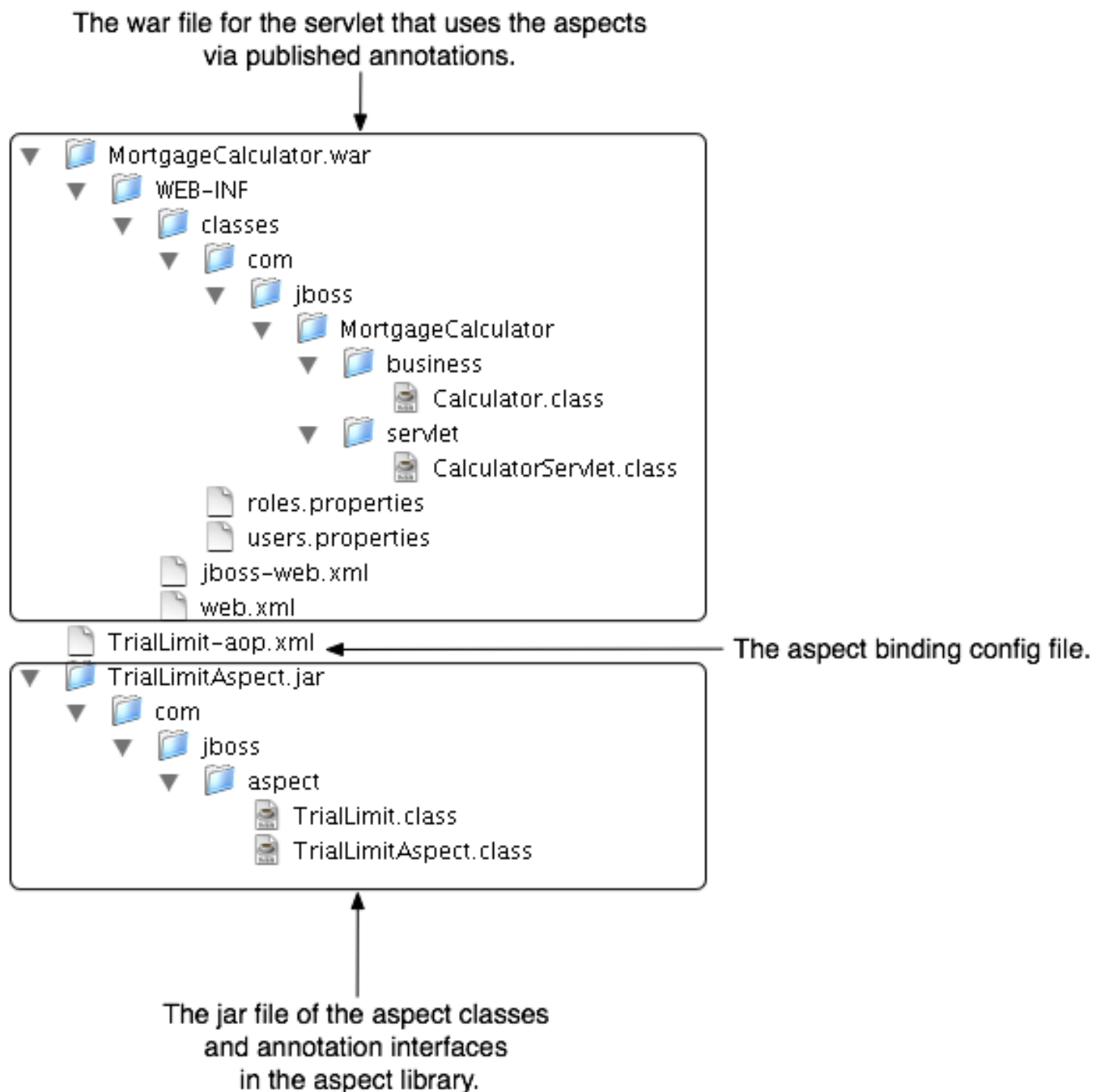
Figure 14.6. The aspect library, binding configuration file and web application are deployed separately.
