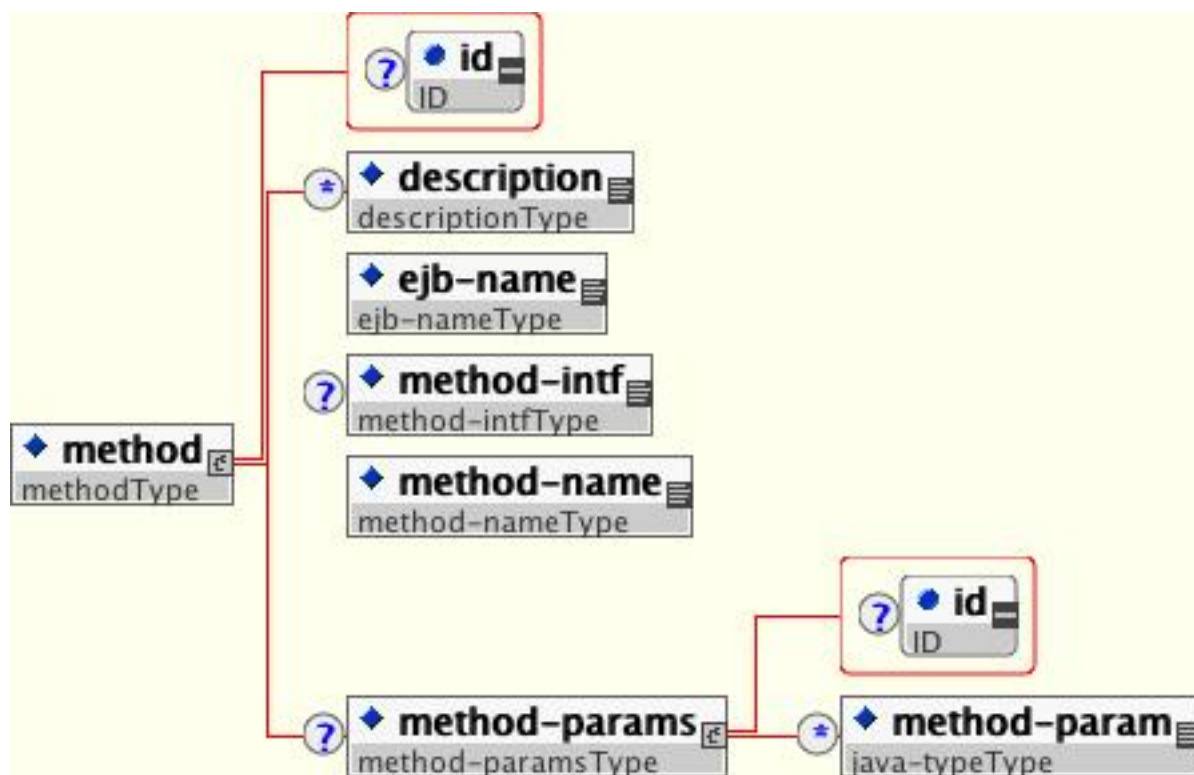
Figure 8.5. The method element
