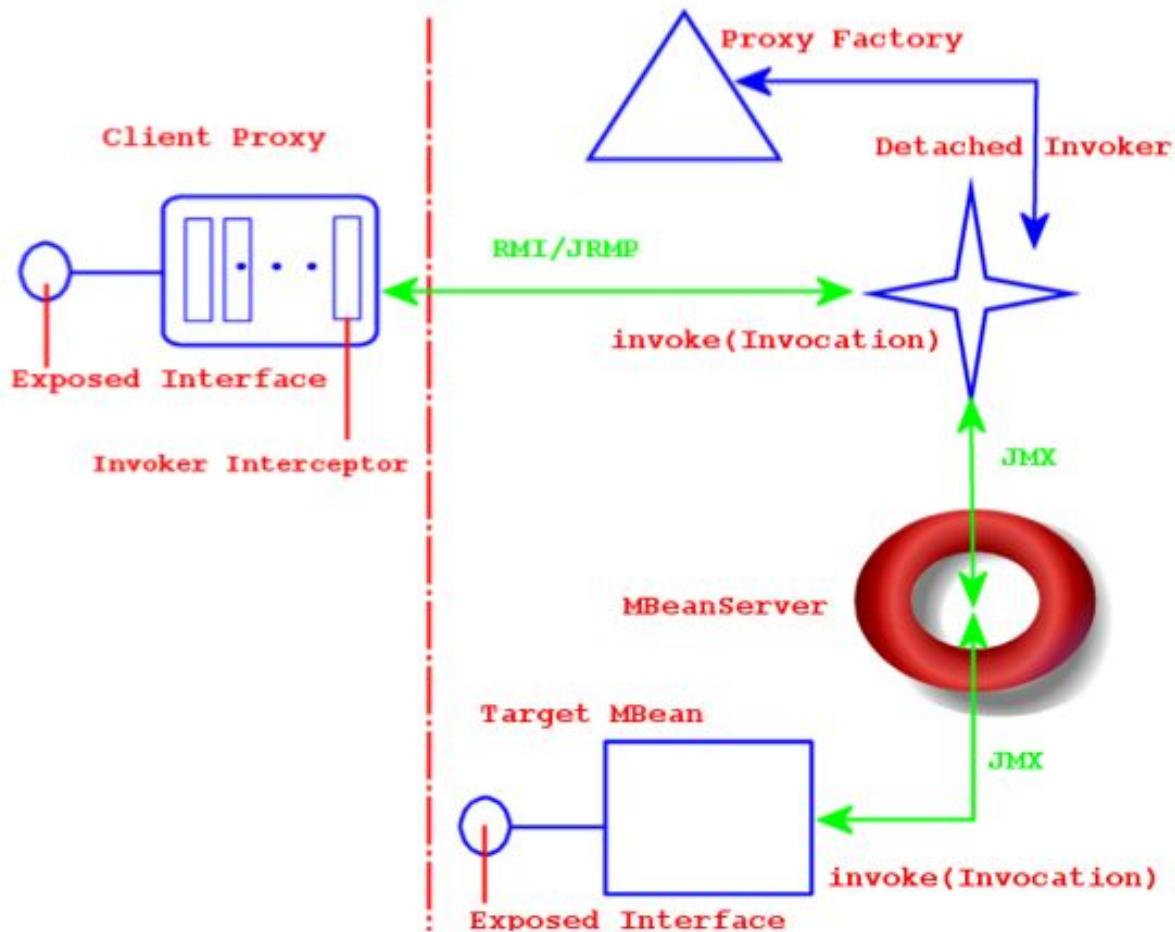
Figure 2.23. The main components in the detached invoker architecture
