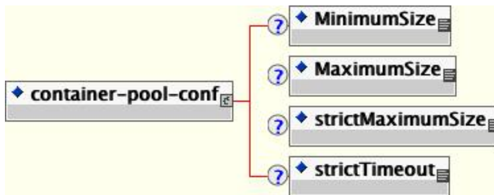
Figure 5.5. The container-pool-conf element DTD
