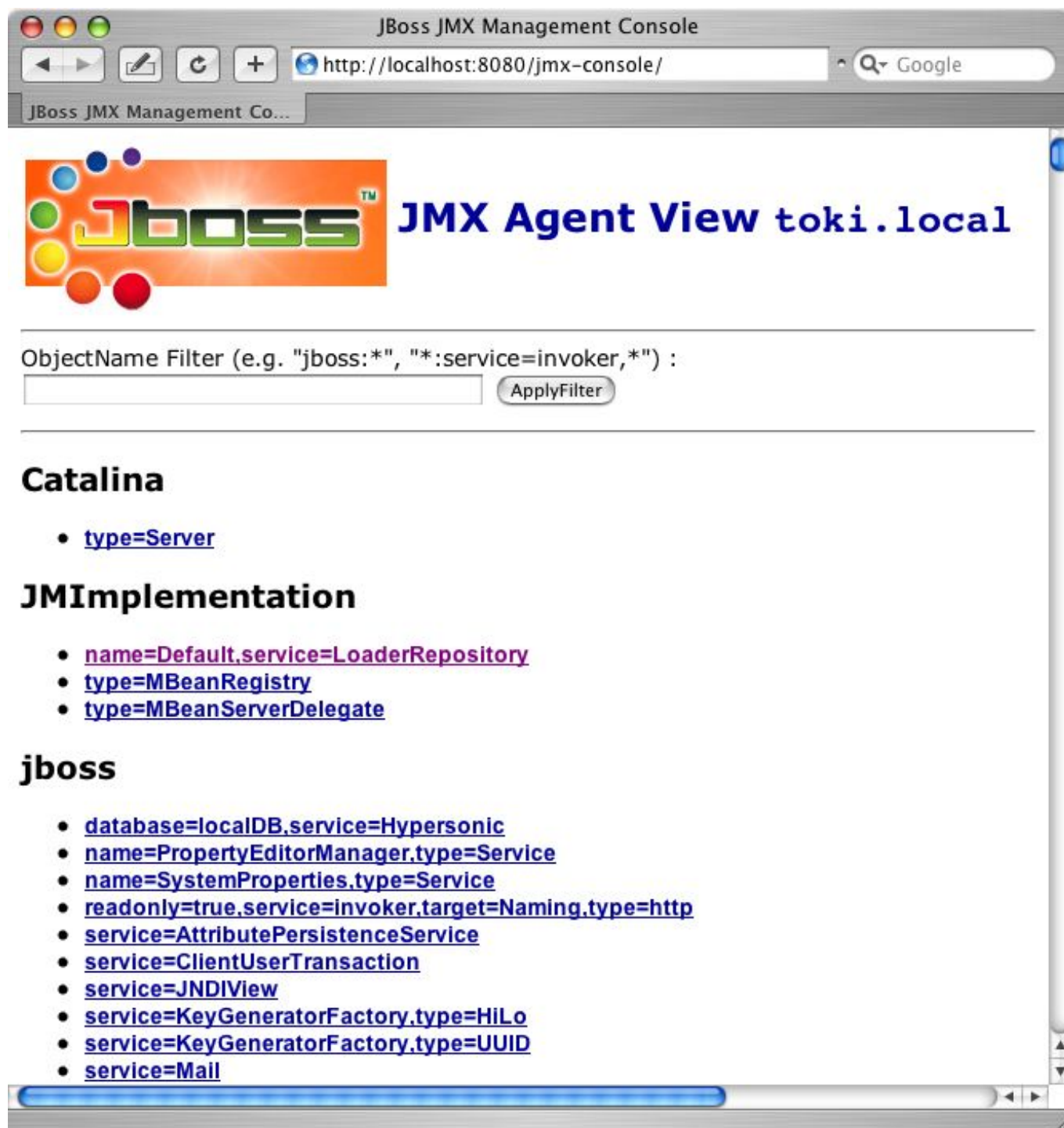
Figure 2.13. The MBean view for the "jboss.system:type=Server" MBean
