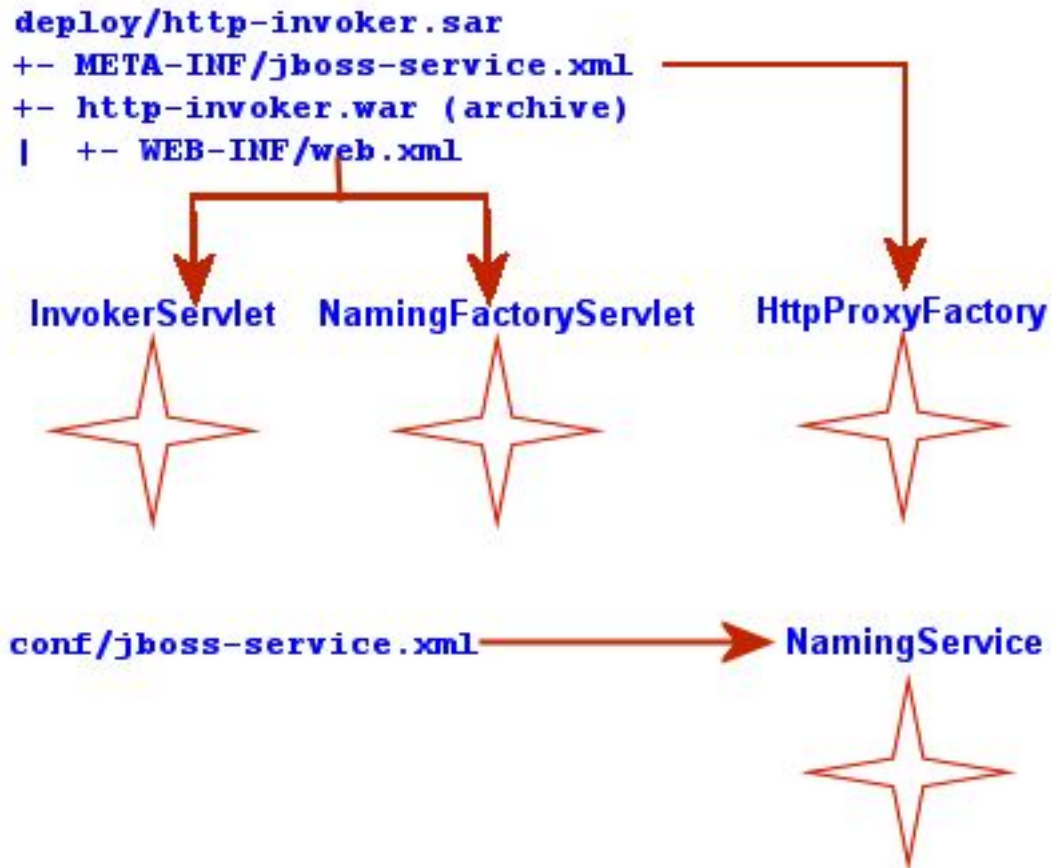
Figure 3.3. The relationship between configuration files and JNDI/HTTP component
