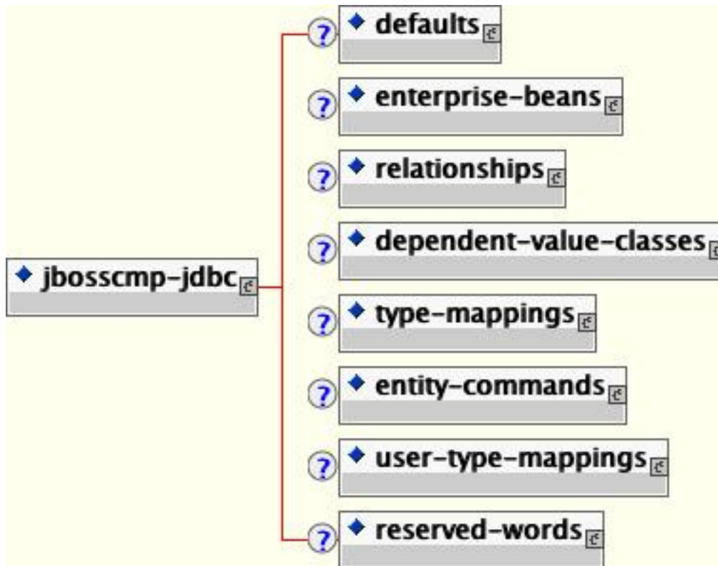
Figure 11.2. The jbosscmp-jdbc content model.
