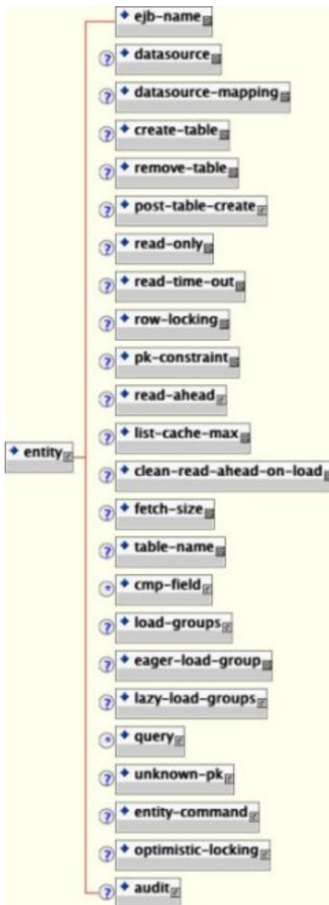
Figure 11.3. The entity element content model
