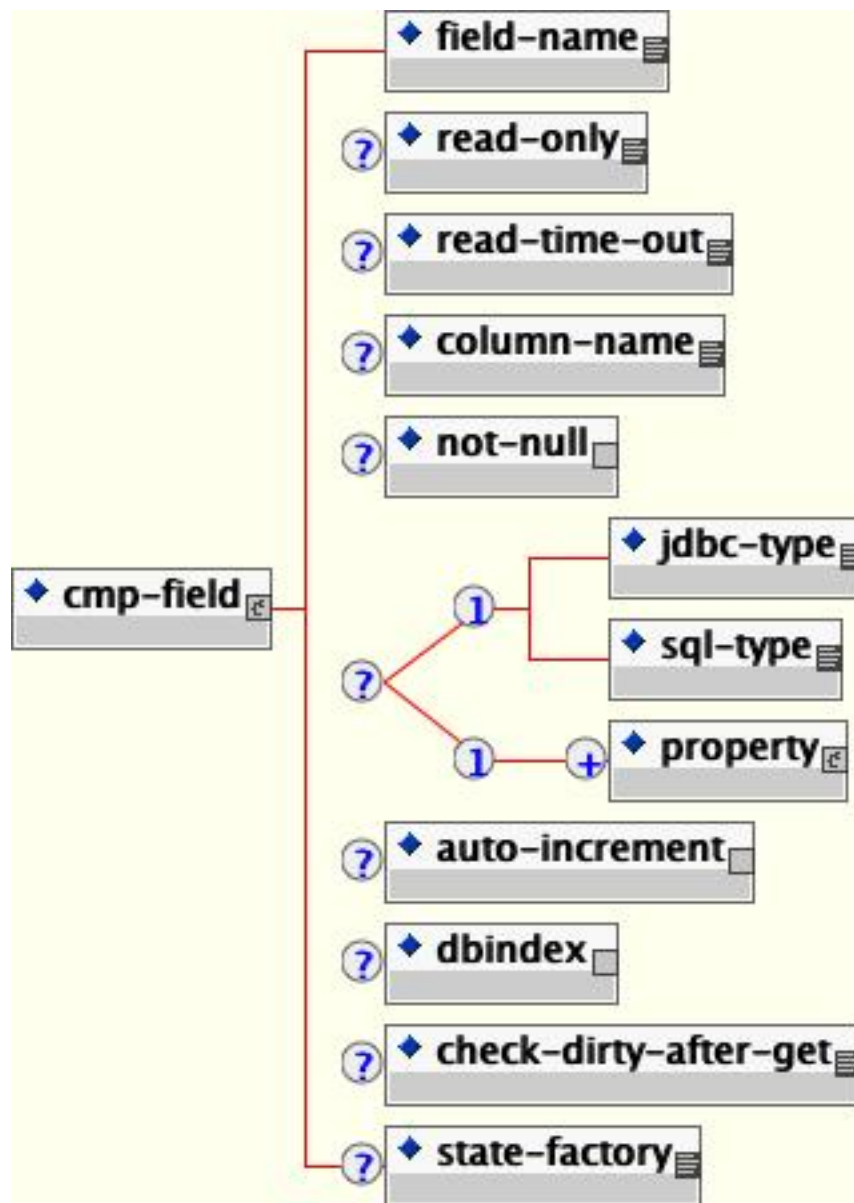
Figure 11.4. The JBoss entity element content model
