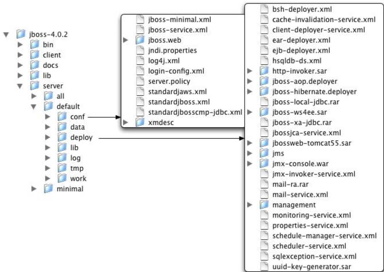
Figure 1.2. An expanded view of the default server configuration file set conf and deploy directories
