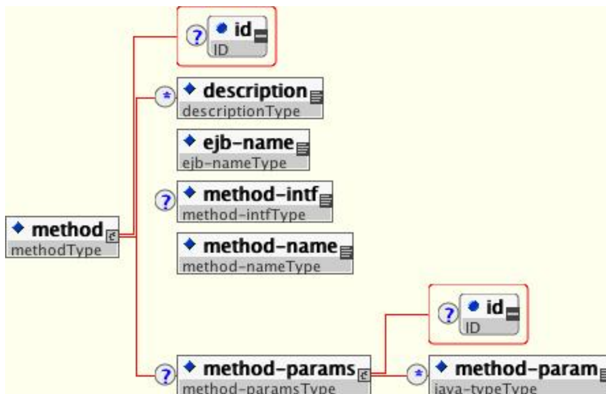
Figure 8.4. The method-permissions element
