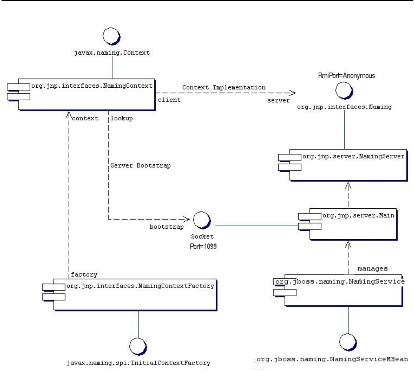
Figure 3.1. Key components in the JBossNS architecture.
