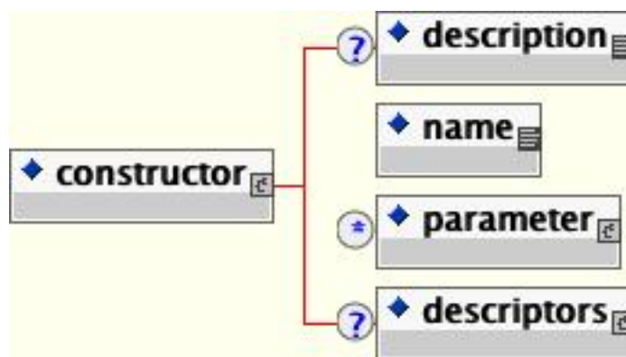
Figure 2.8. The XMBean constructor element and its content model
