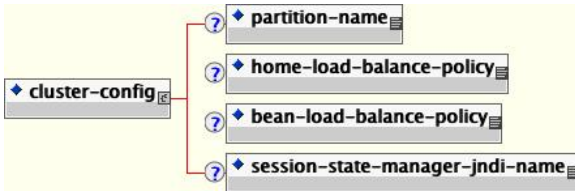
Figure 5.7. The cluster-config and related elements
