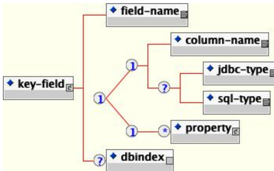
Figure 11.9. The jbosscmp-jdbc key-fields element content model
