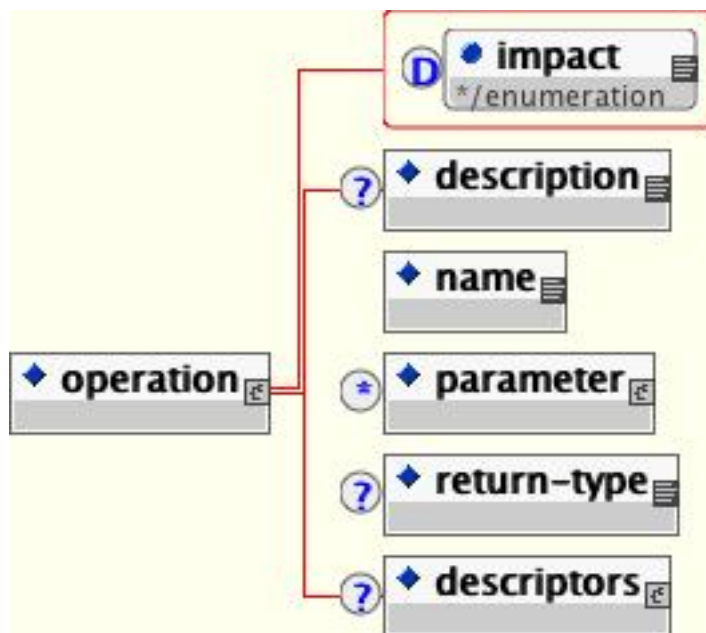
Figure 2.10. The XMBean operation element and its content model
