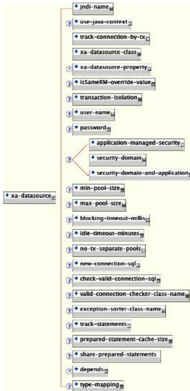
Figure 7.9. The XA DataSource configuration schema
