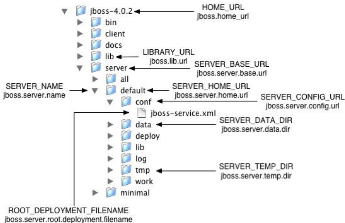
Figure 1.1. A view of the JBoss server installation directory structure with the default server configuration file set expanded and overridable locations identified
