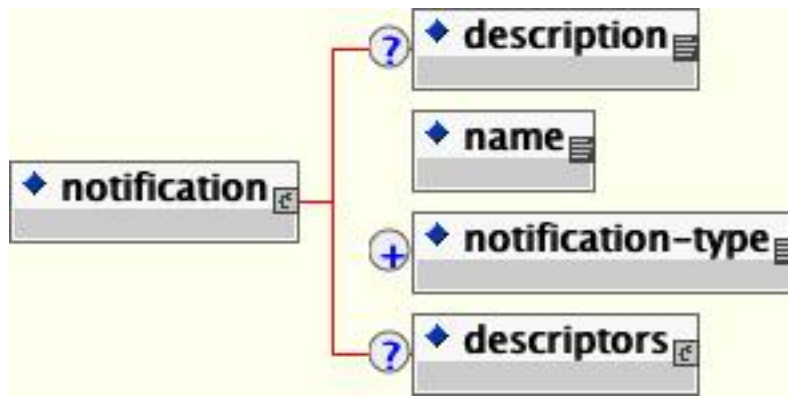
Figure 2.11. The XMBean notification element and content model
