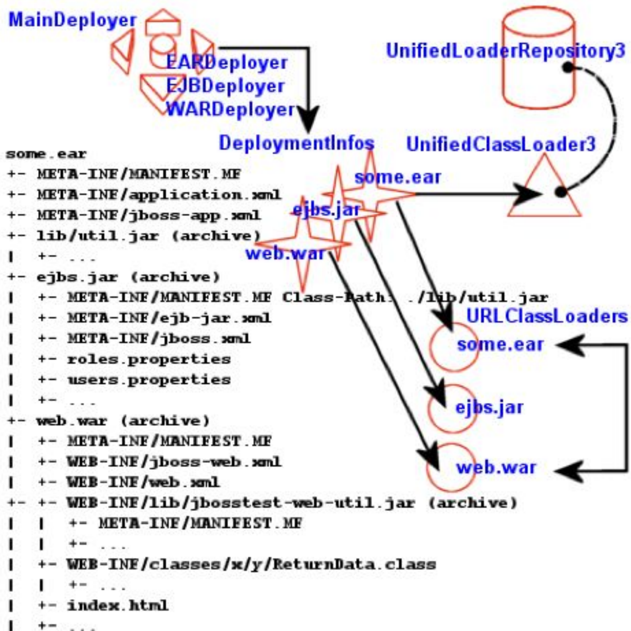
Figure 2.20. An illustration of the class loaders involved with an EAR deployment
