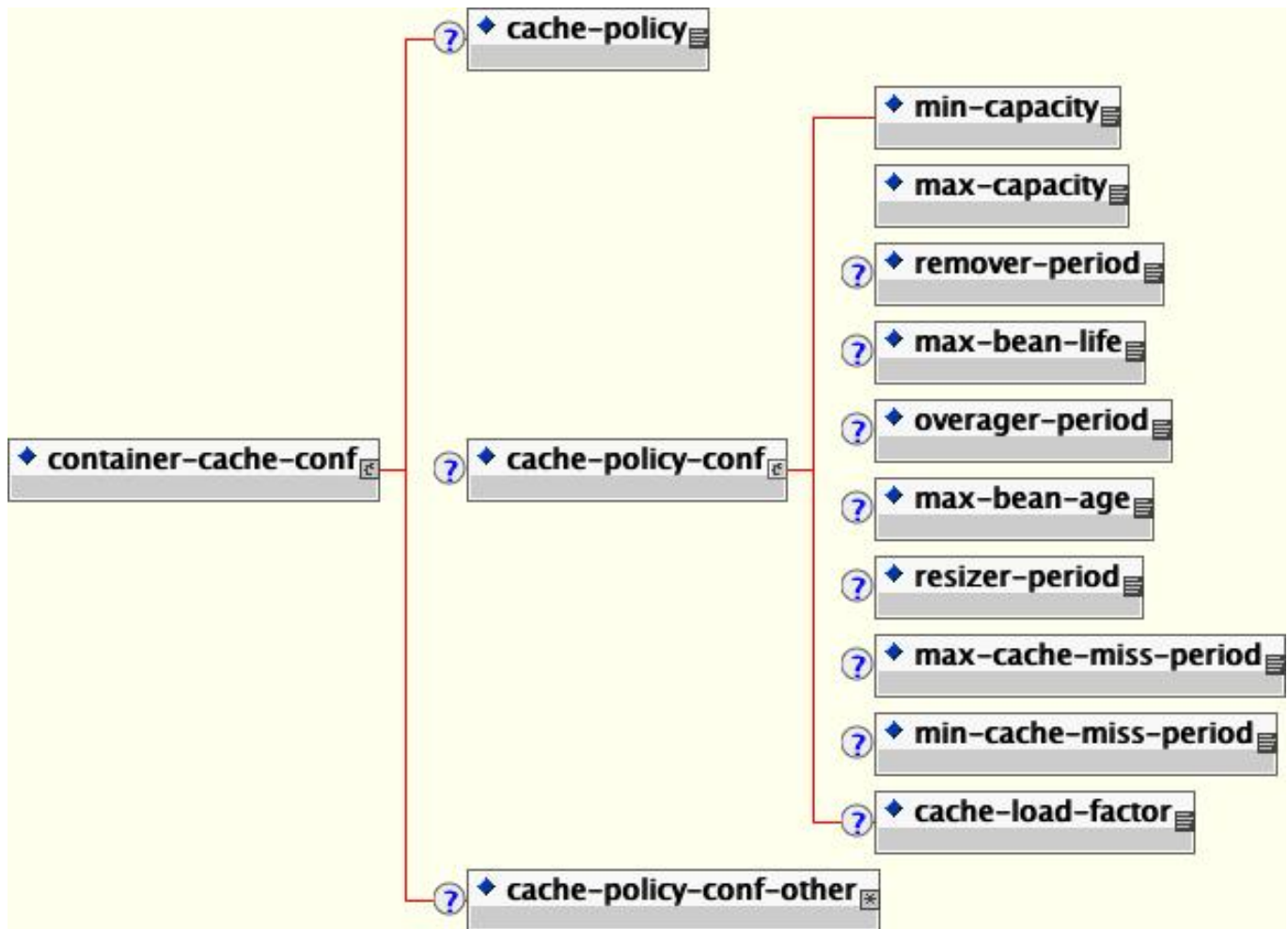
Figure 5.6. The container-cache-conf element DTD
