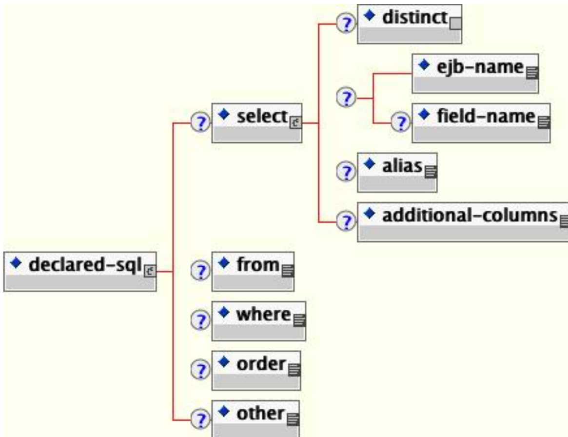
Figure 11.12. The jbosscomp-jdbc declared-sql element content model.>
