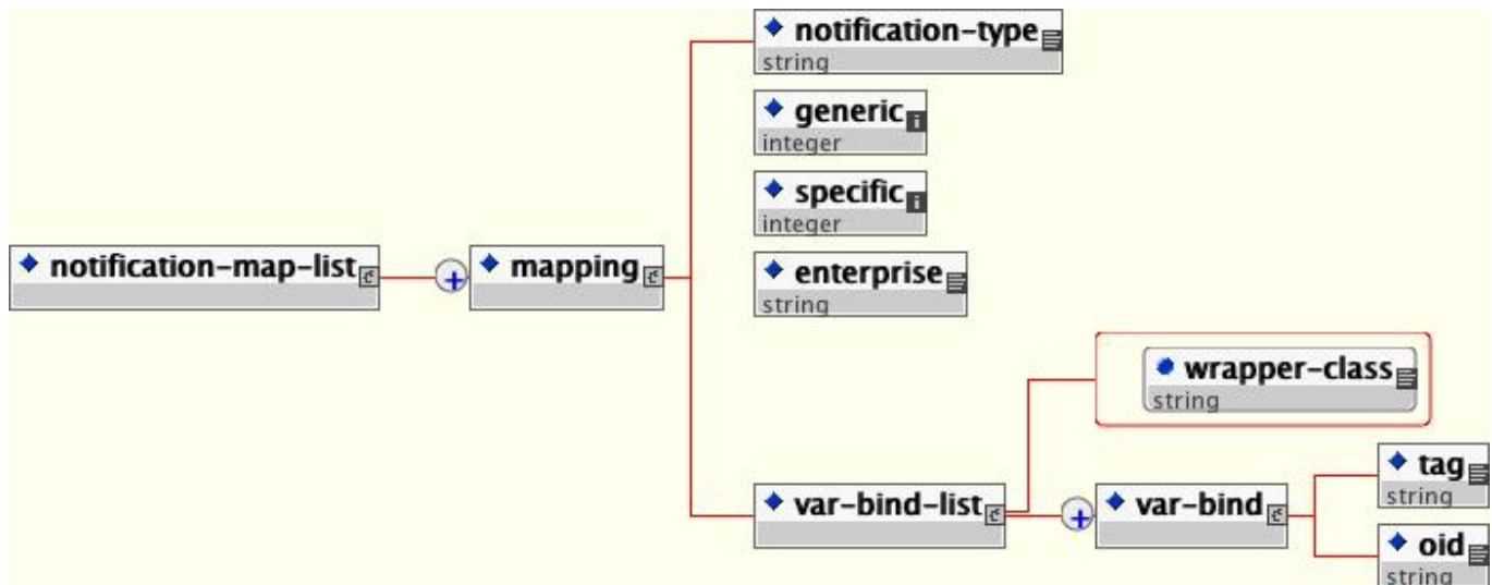
Figure 2.22. The schema for the notification to trap mapping file
