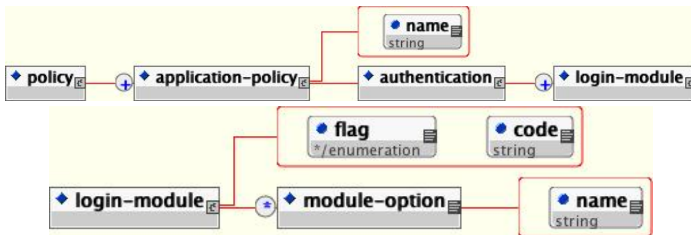
Figure 8.13. The XMLLoginConfig DTD
