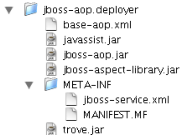
Figure 14.1. The directory structure of the JBoss AOP deployer in JBoss AS.
