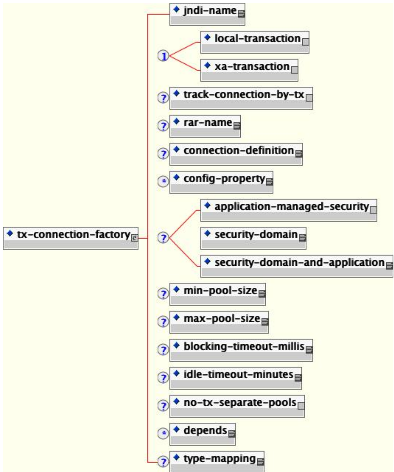
Figure 7.14. The tx-connection-factory element schema
