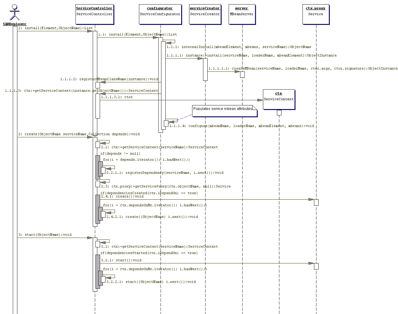
Figure 2.17. The interaction between the SARDeployer and ServiceController to start a service
