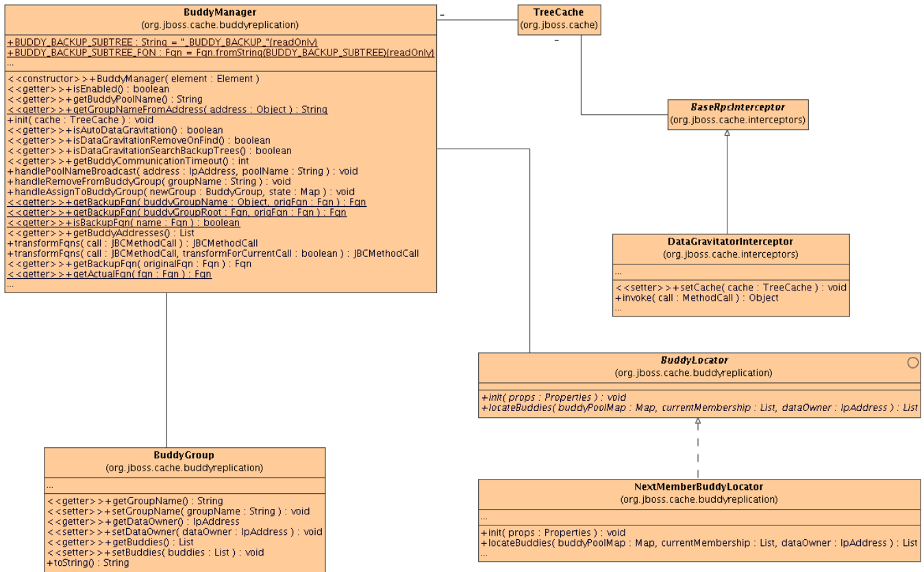
Figure 4.1. Class diagram of the classes involved in buddy replication and how they are related to each other
