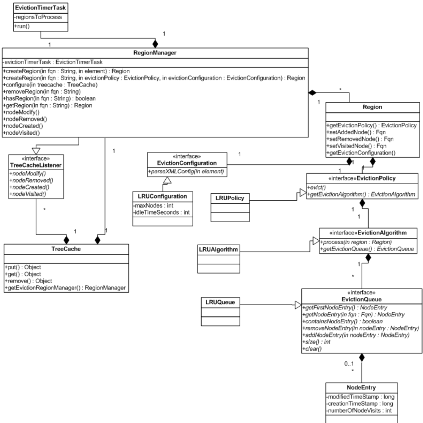
Figure 6.1. TreeCache eviction UML Diagram
