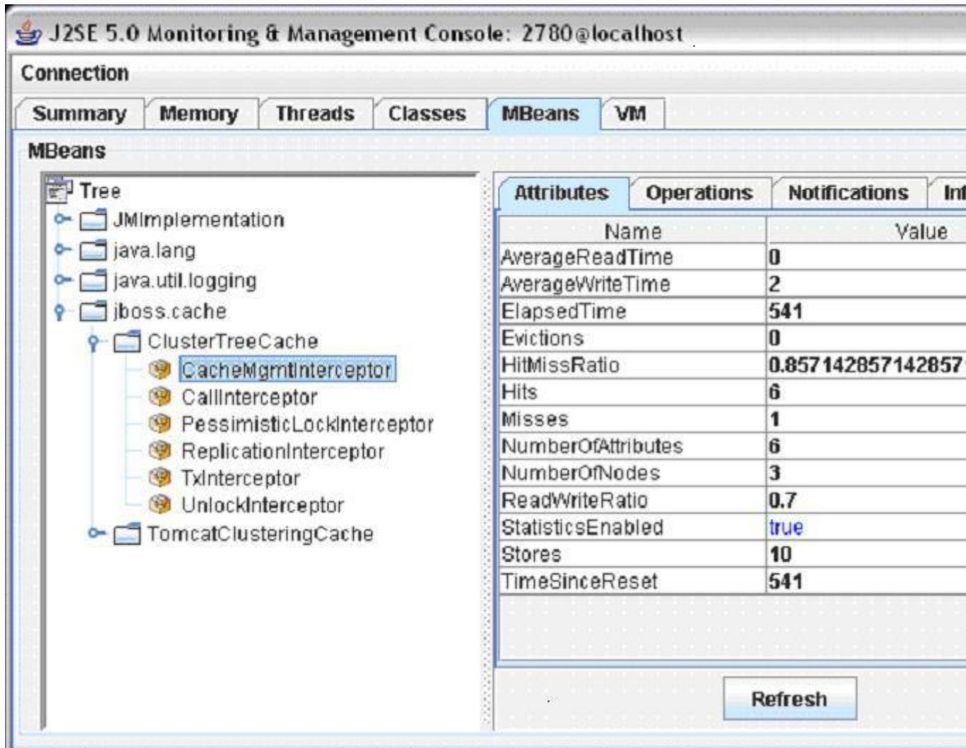
Figure 4.1. CacheMgmtInterceptor MBean in jconsole
