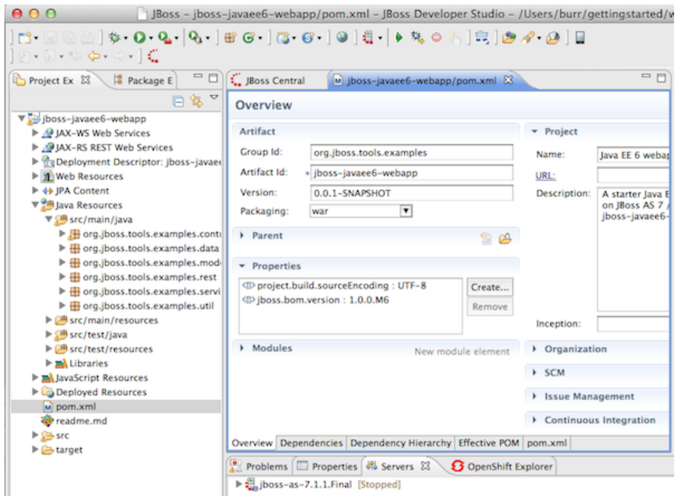
Figure 4.1: Project Explorer
