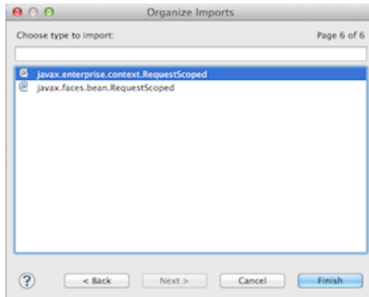
Figure 9.9: javax.enterprise.context.RequestScoped
