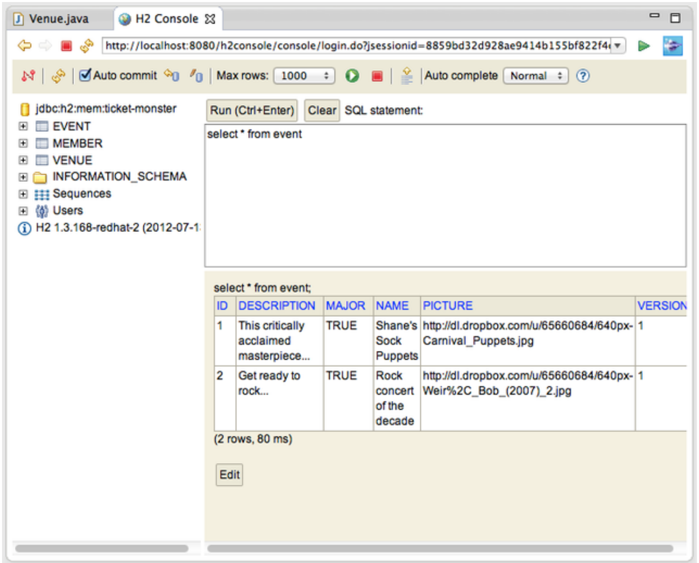
Figure 13.4: h2console Select * from Event
