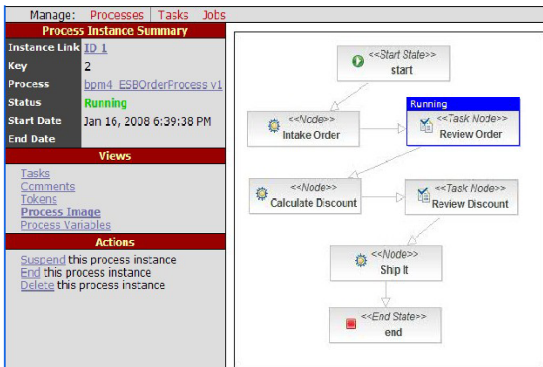
Figure 7.4. The Order Process Has Reached the “Review Order” Node
