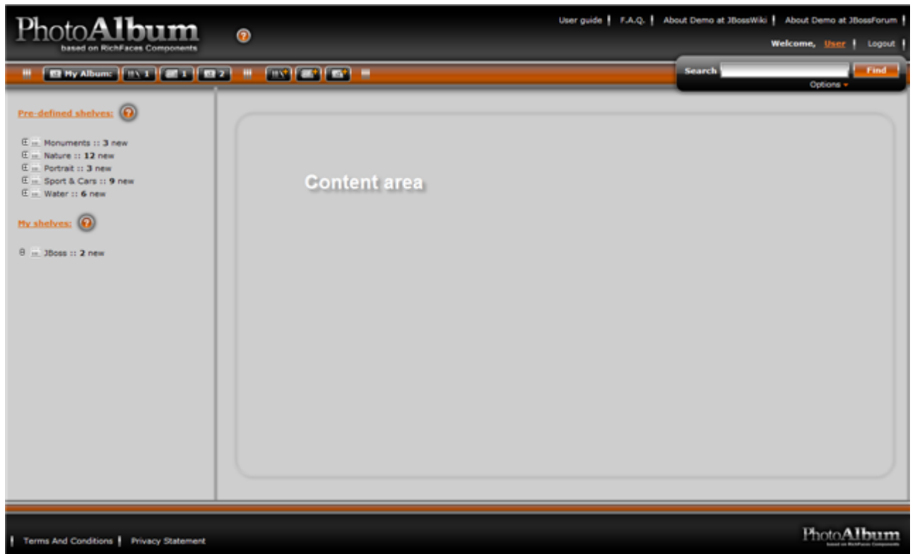
Figure 3.2. Content Area
