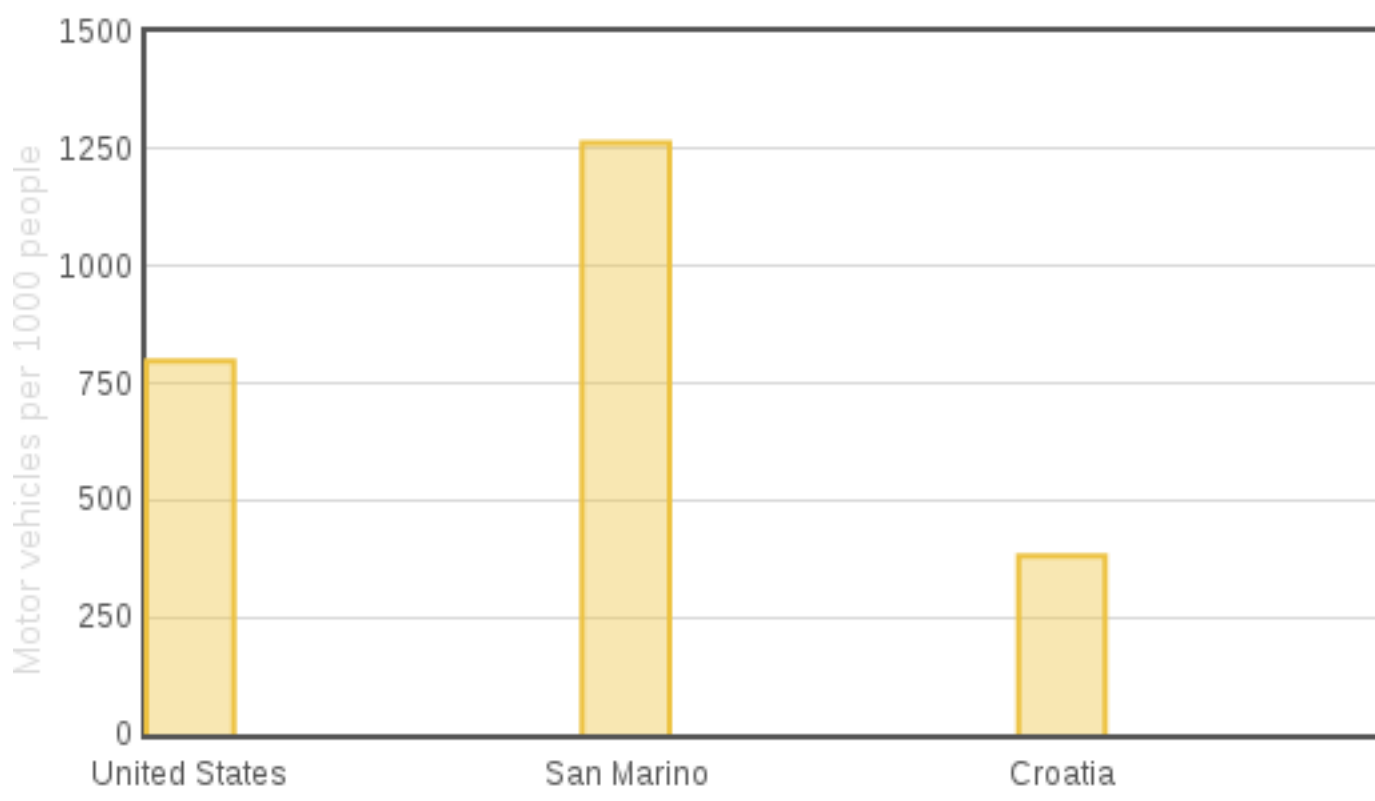
Figure 13.1. rich:chart component
