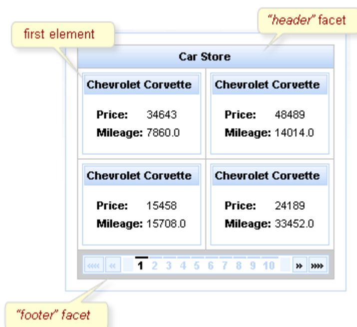
Figure 10.14. <rich:dataGrid> example
