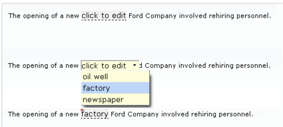
Figure 8.3. <rich:inplaceSelect>
