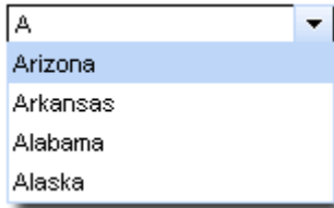
Figure 8.6. <rich:select>
