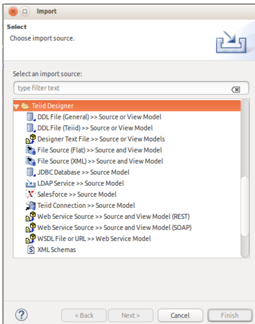
Figure 5.1. Import Wizard
