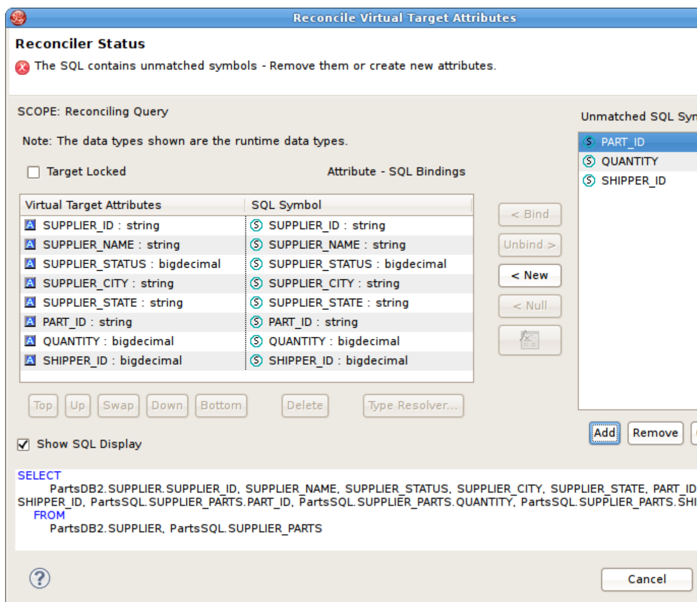
Figure 6.30. Reconciler Dialog
