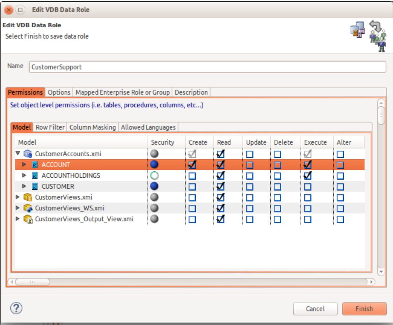
Figure D.59. VDB Data Roles Tab
