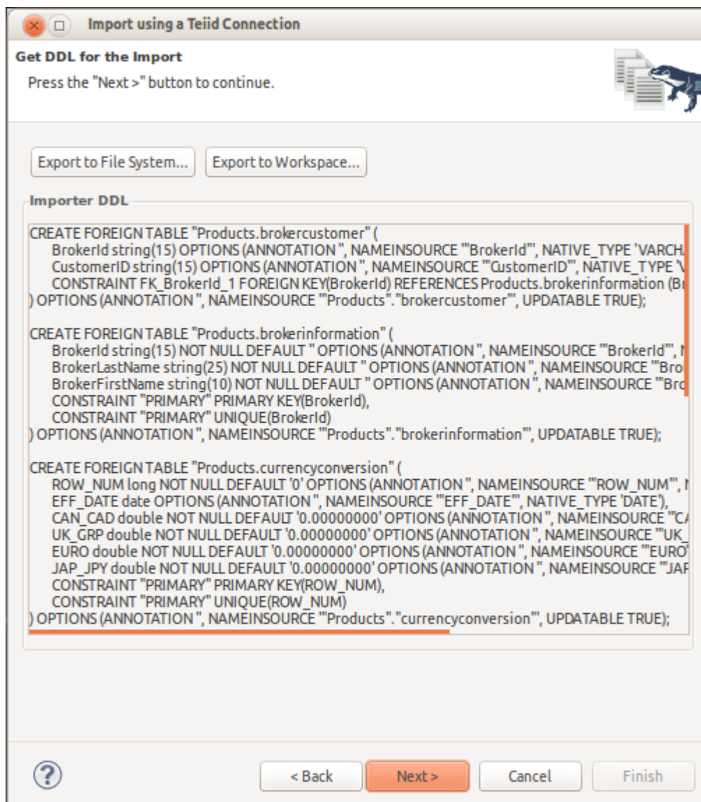
Figure 5.14. Review DDL Dialog
