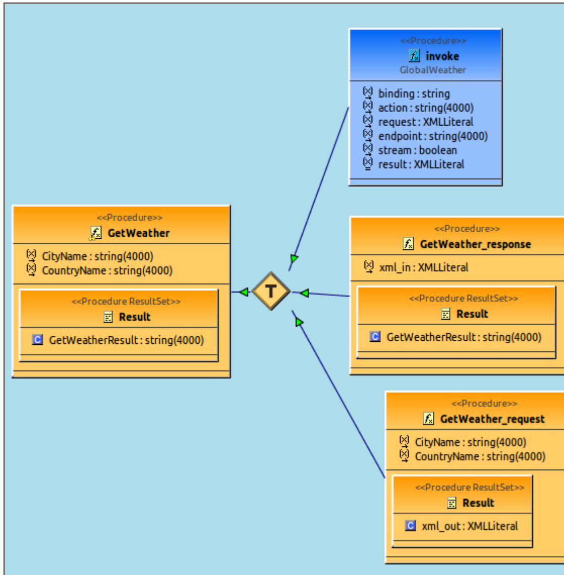
Figure 5.57. Example Web Services Wrapper Procedure
