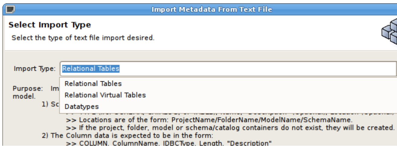
Figure 3.26. Import Wizard
