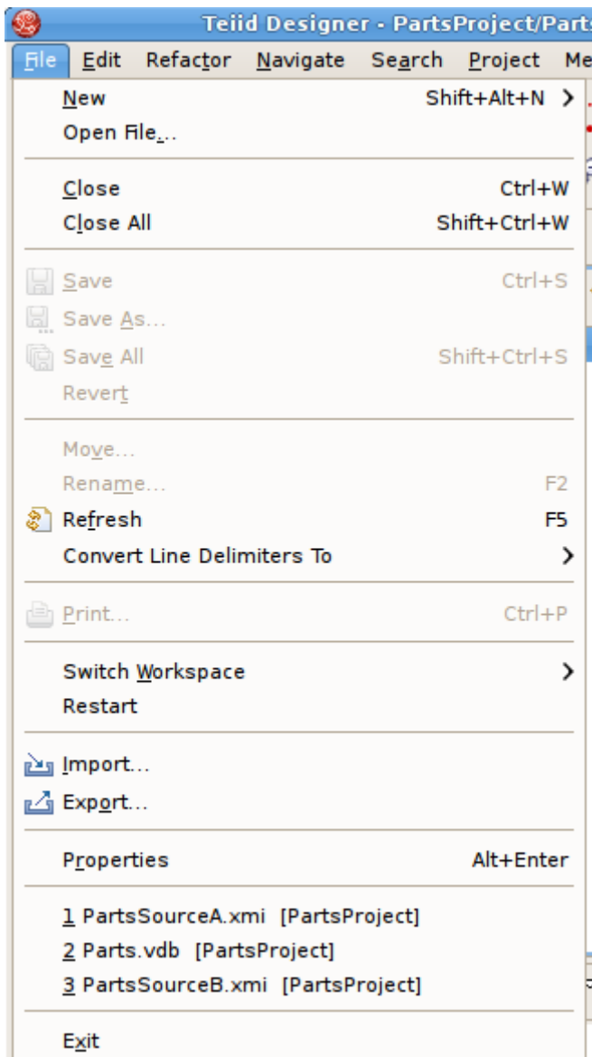
Figure 10.59. File Menu
