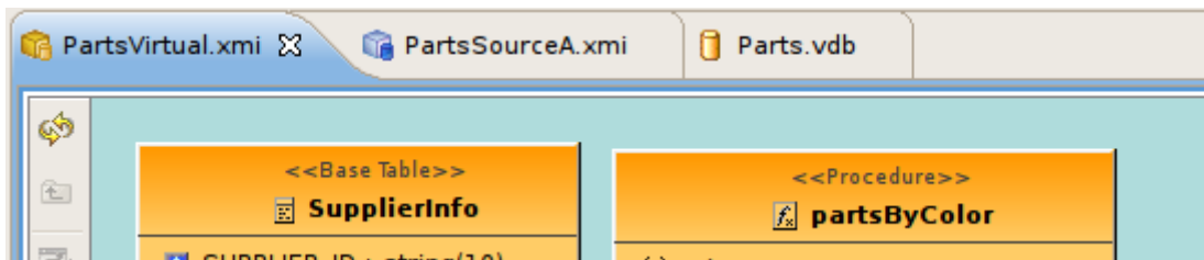
Figure 10.33. Editor Tabs
