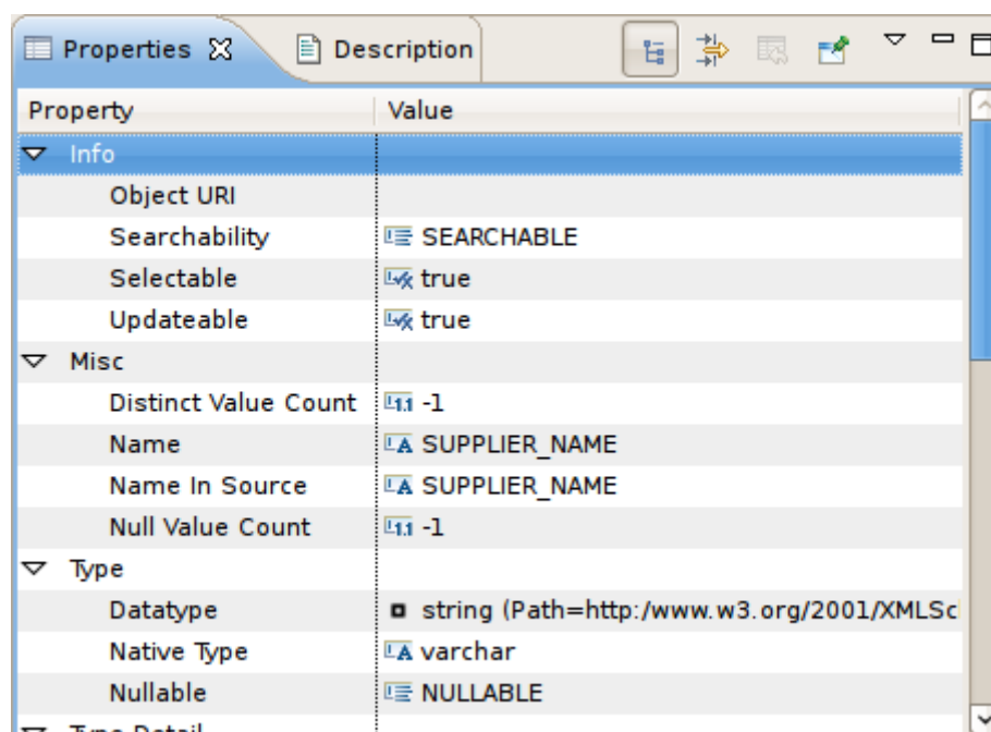
Figure 10.16. Properties View
