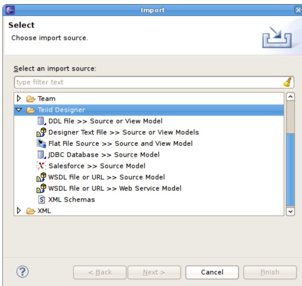
Figure 3.1. Import Wizard
