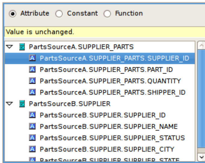
Figure 4.15. Attribute Panel
