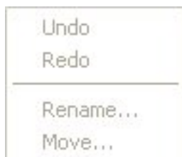
Figure 10.62. Refactor Menu
