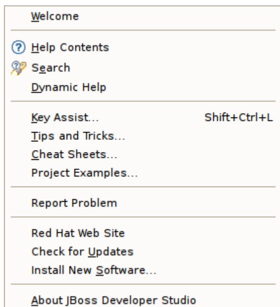
Figure 10.71. Help Menu
