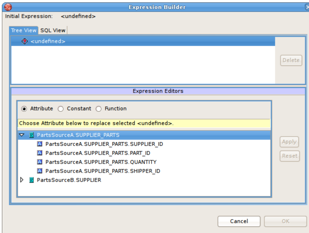
Figure 4.18. Expression Builder
