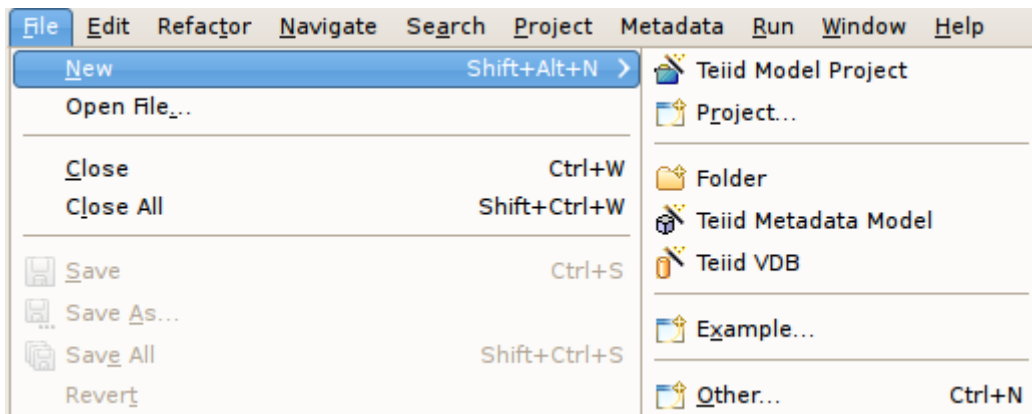
Figure 10.60. File Menu
