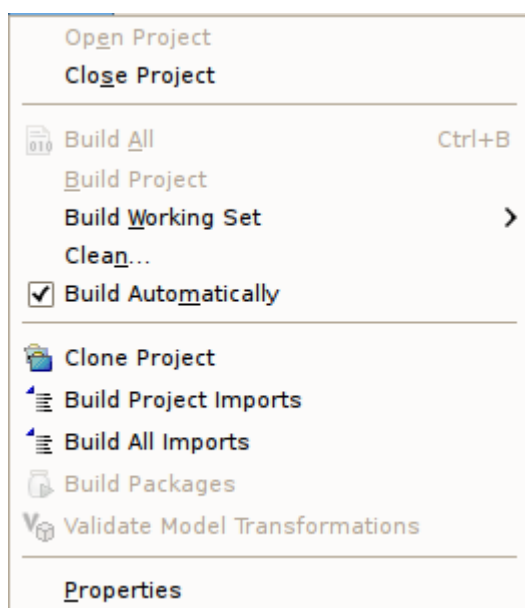
Figure 10.66. Project Menu
