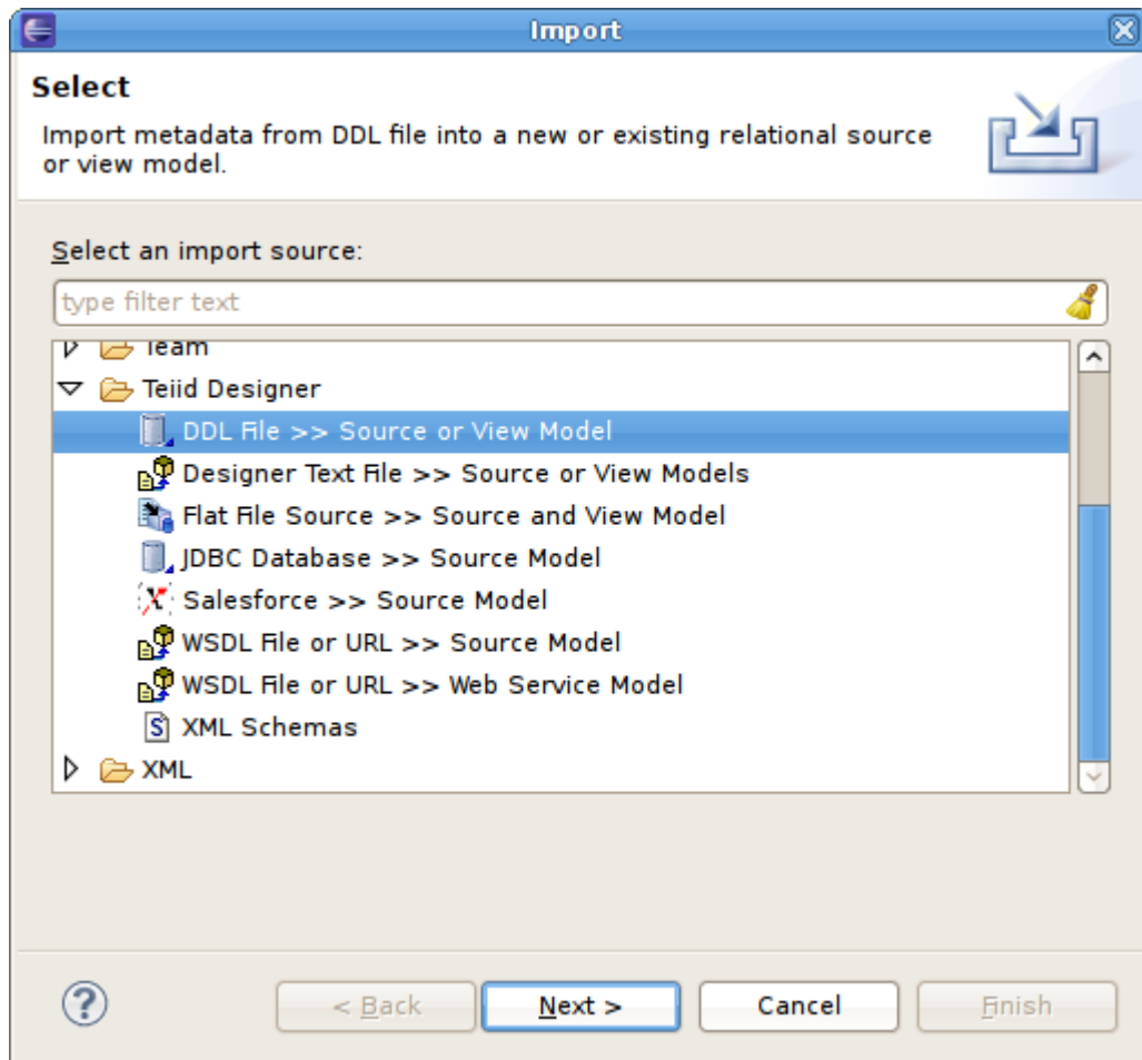
Figure 3.2. Import DDL
