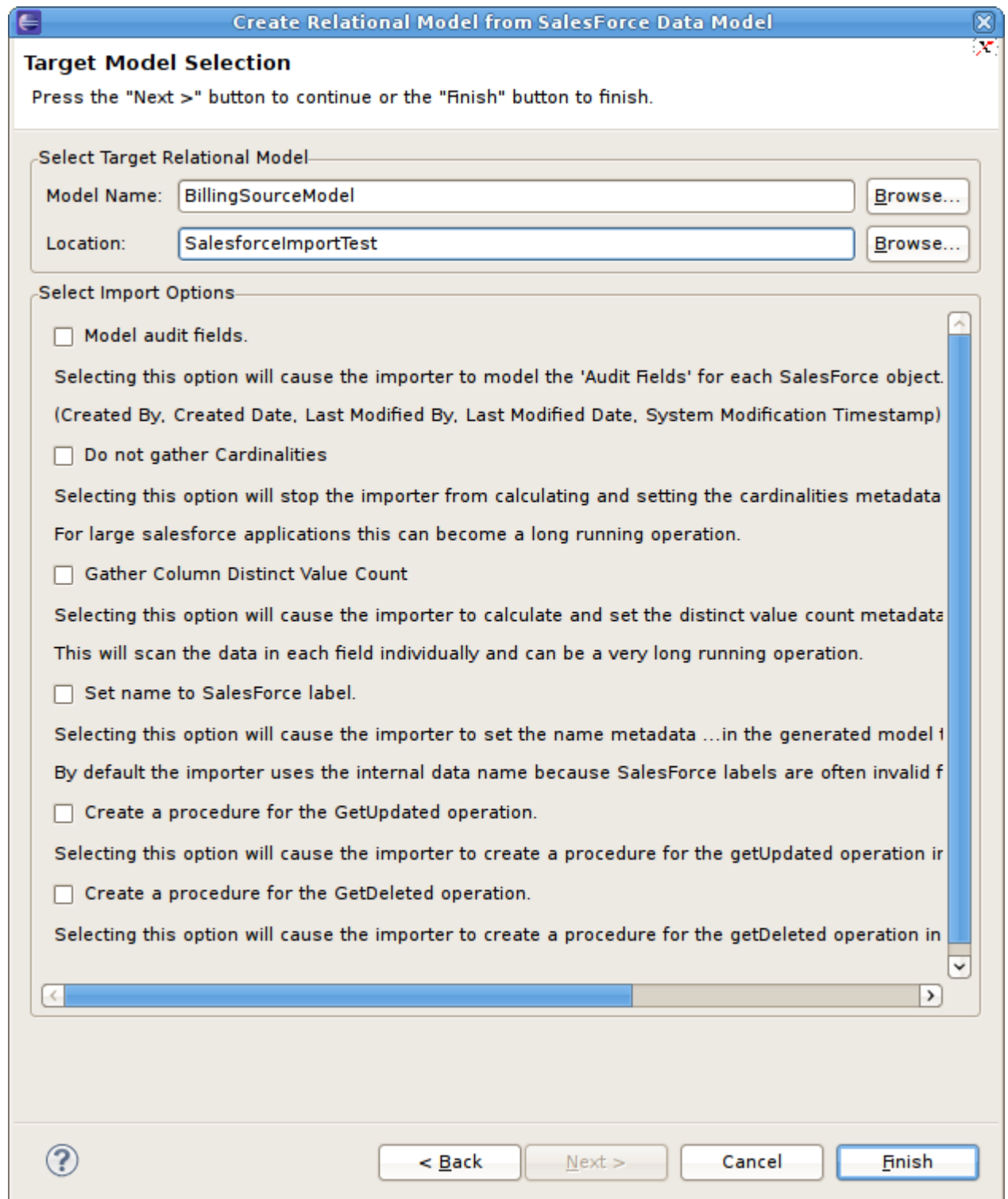
Figure 5.30. Target Model Selection Dialog
