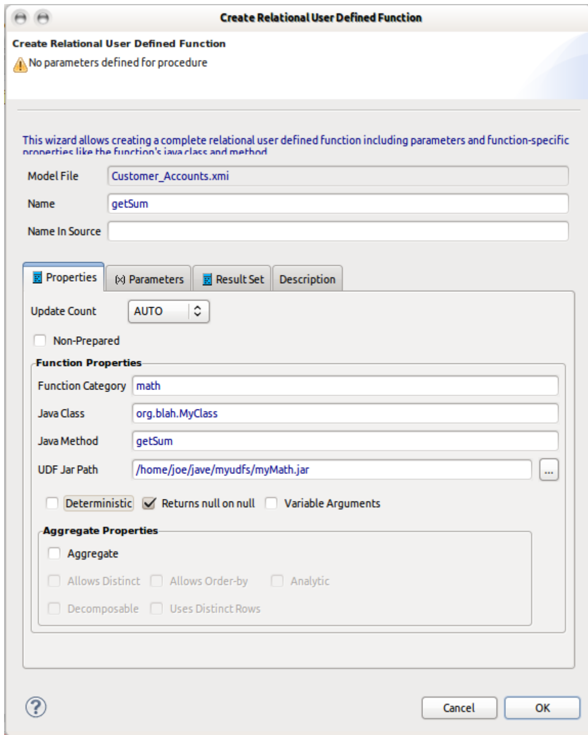
Figure 6.16. Create Relational User Defined Fuction Dialog
