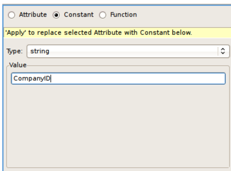
Figure 6.27. Constants Panel
