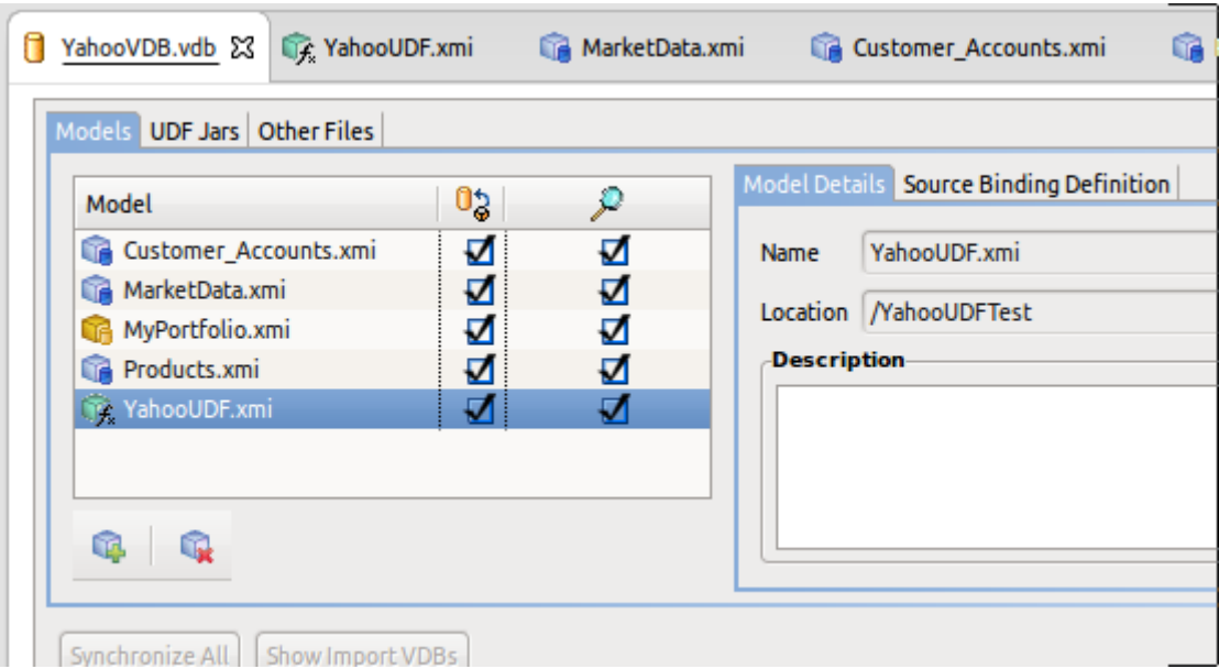
Figure 9.4. VDB Models
