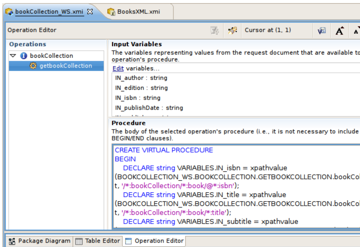
Figure 6.40. Operation Editor
