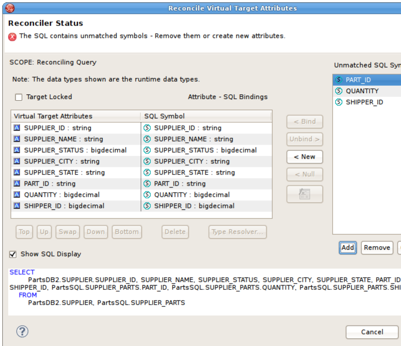
Figure 6.23. Reconciler Dialog
