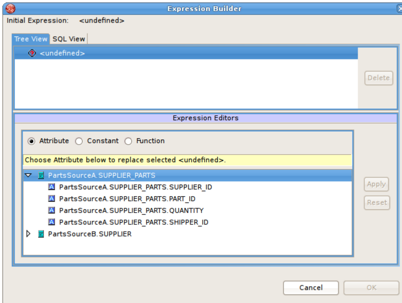
Figure 6.29. Expression Builder
