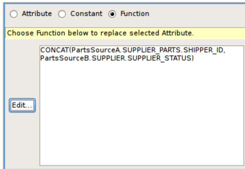
Figure 6.28. Functions
