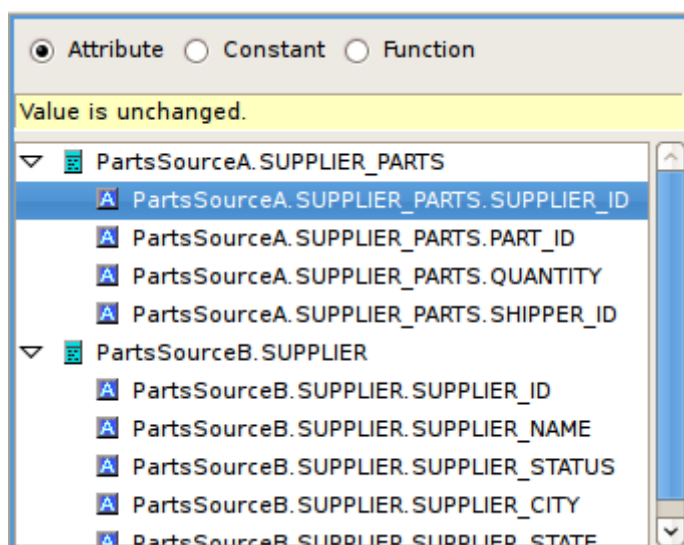
Figure 6.26. Attribute Panel
