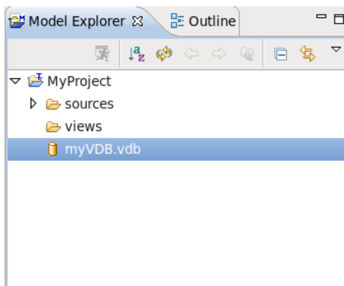
Figure 2.18. Model Explorer
