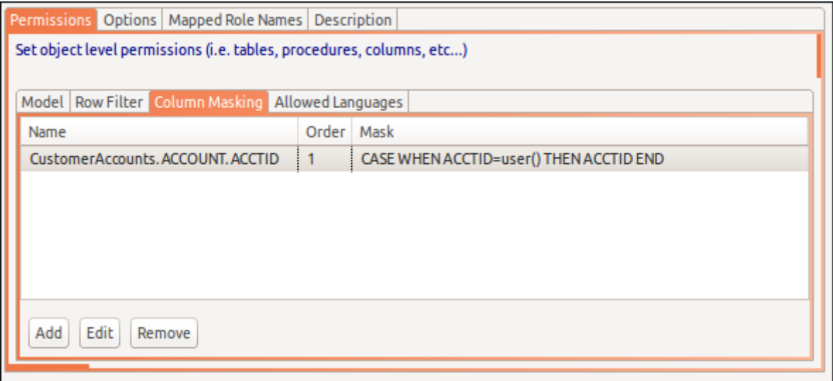
Figure 10.8. Column Masking Tab
