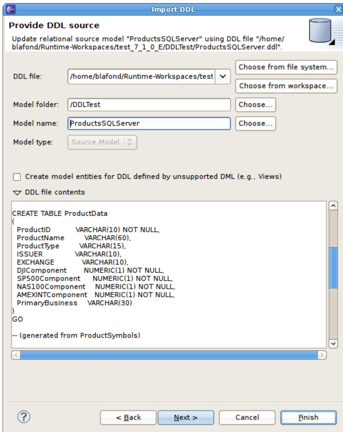
Figure 5.2. DDL Import Options
