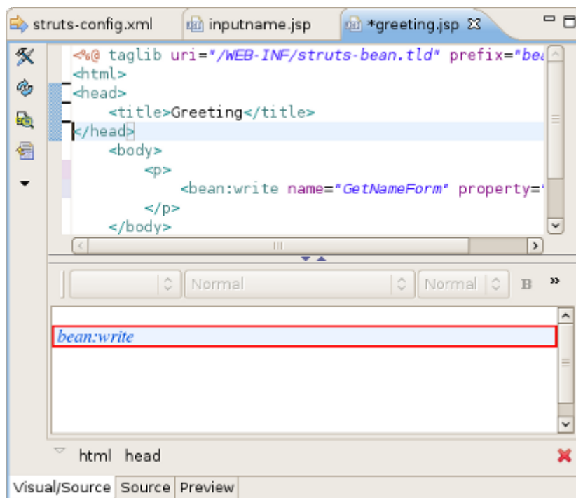
Figure 4.3. Editor Window
