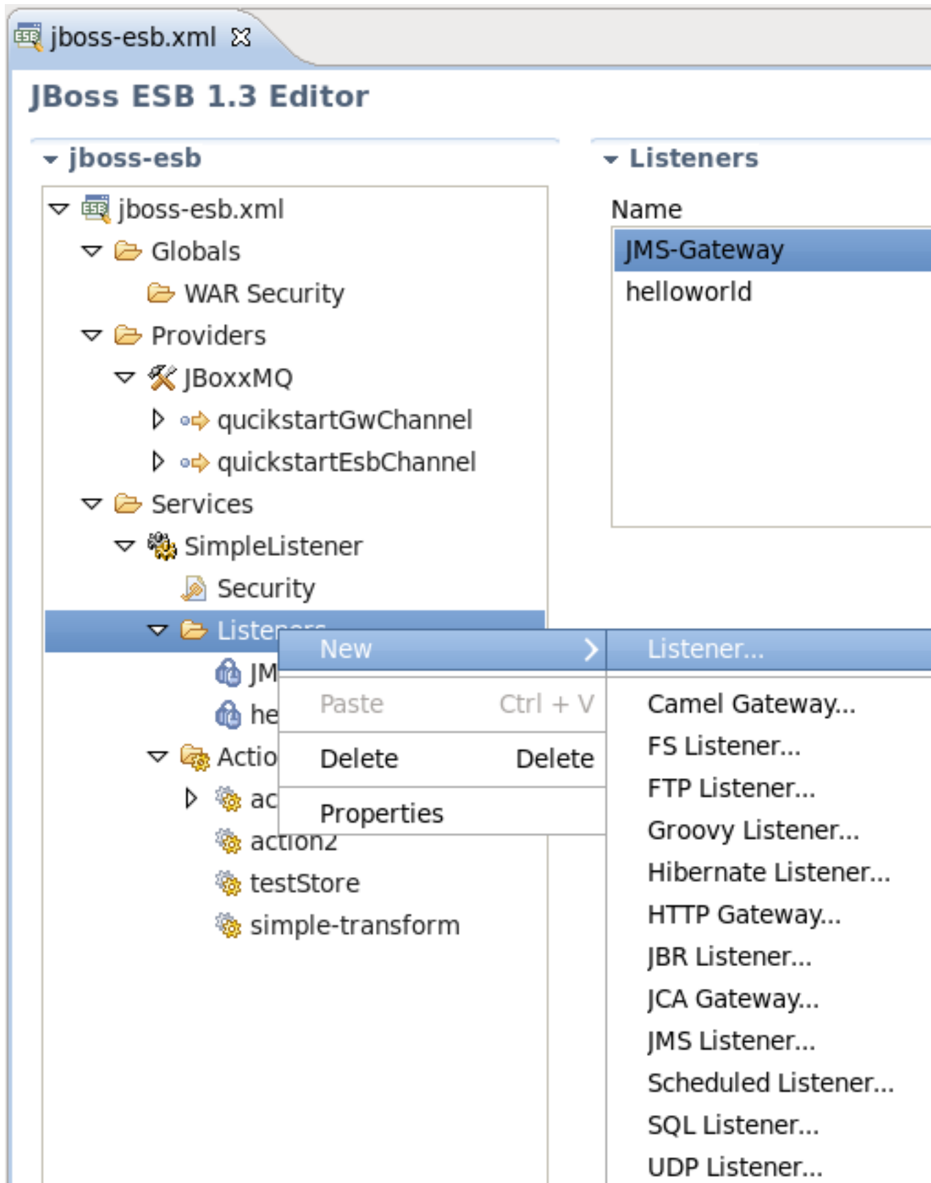
Figure 3.8. Adding New Listener for Service
