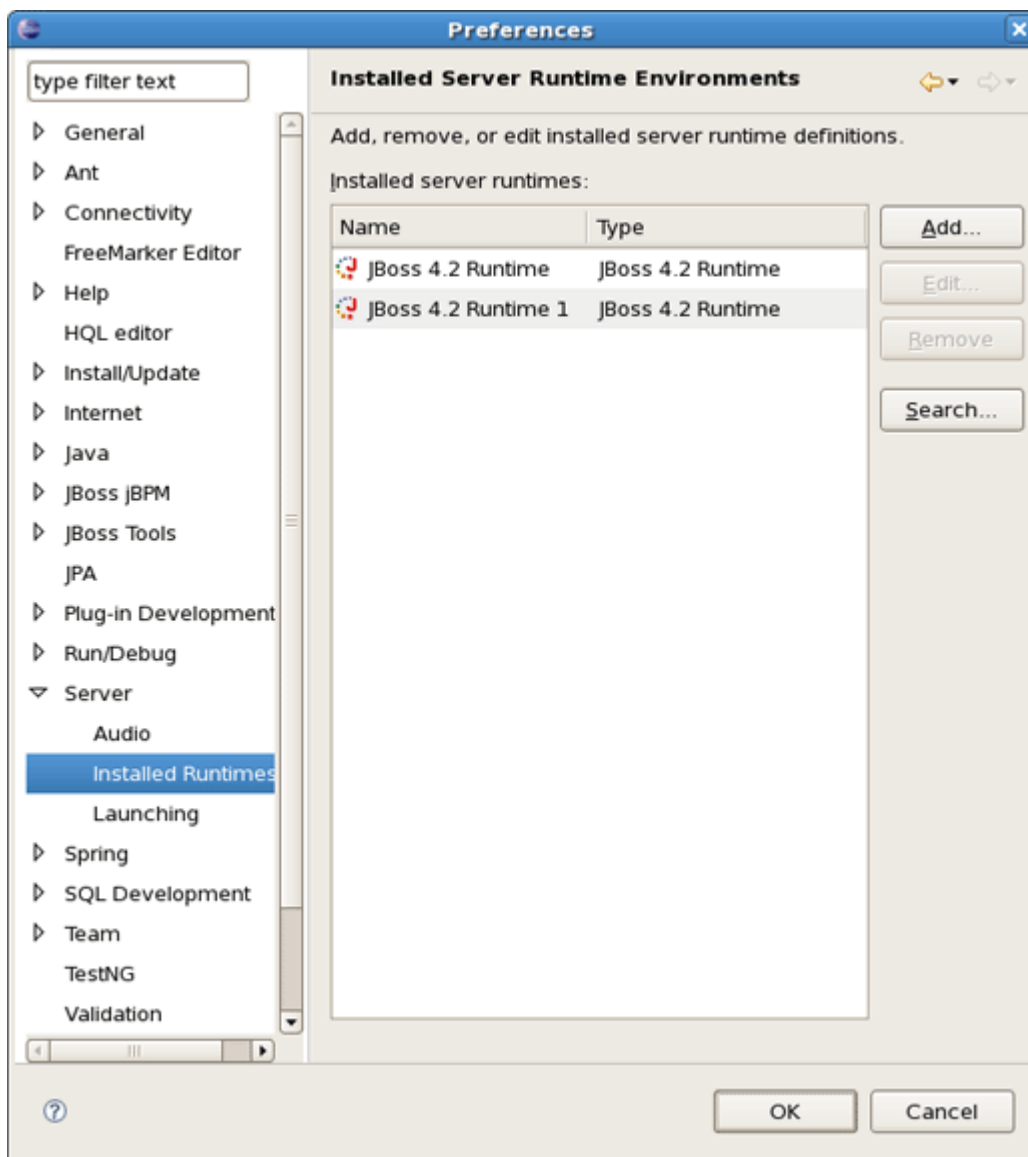
Figure 2.1. Installed Runtimes
