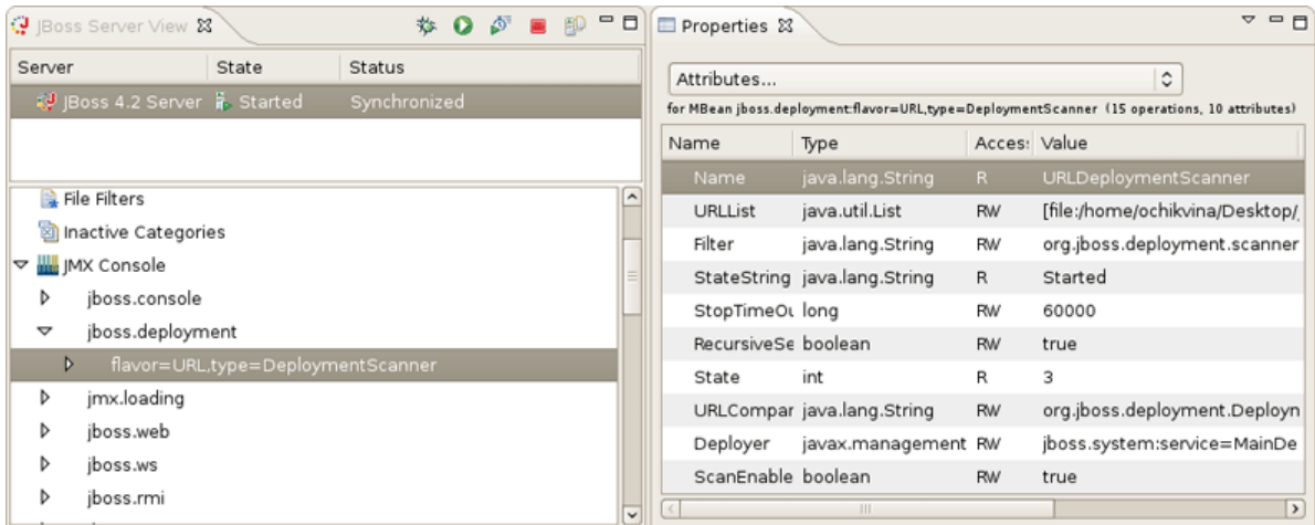
Figure 3.18. JMX Console
