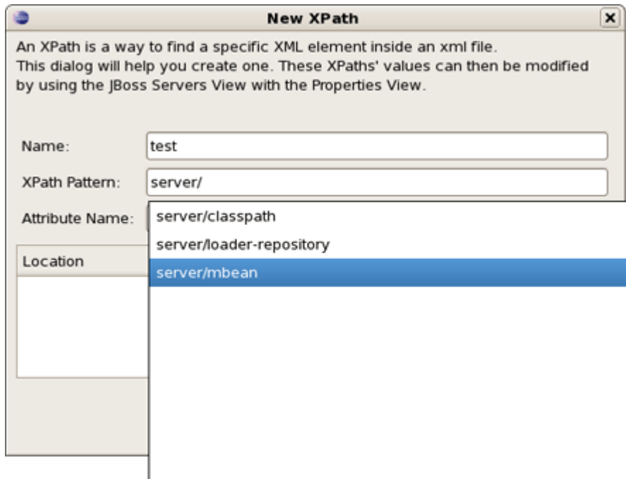
Figure 3.16. XPath Preview
