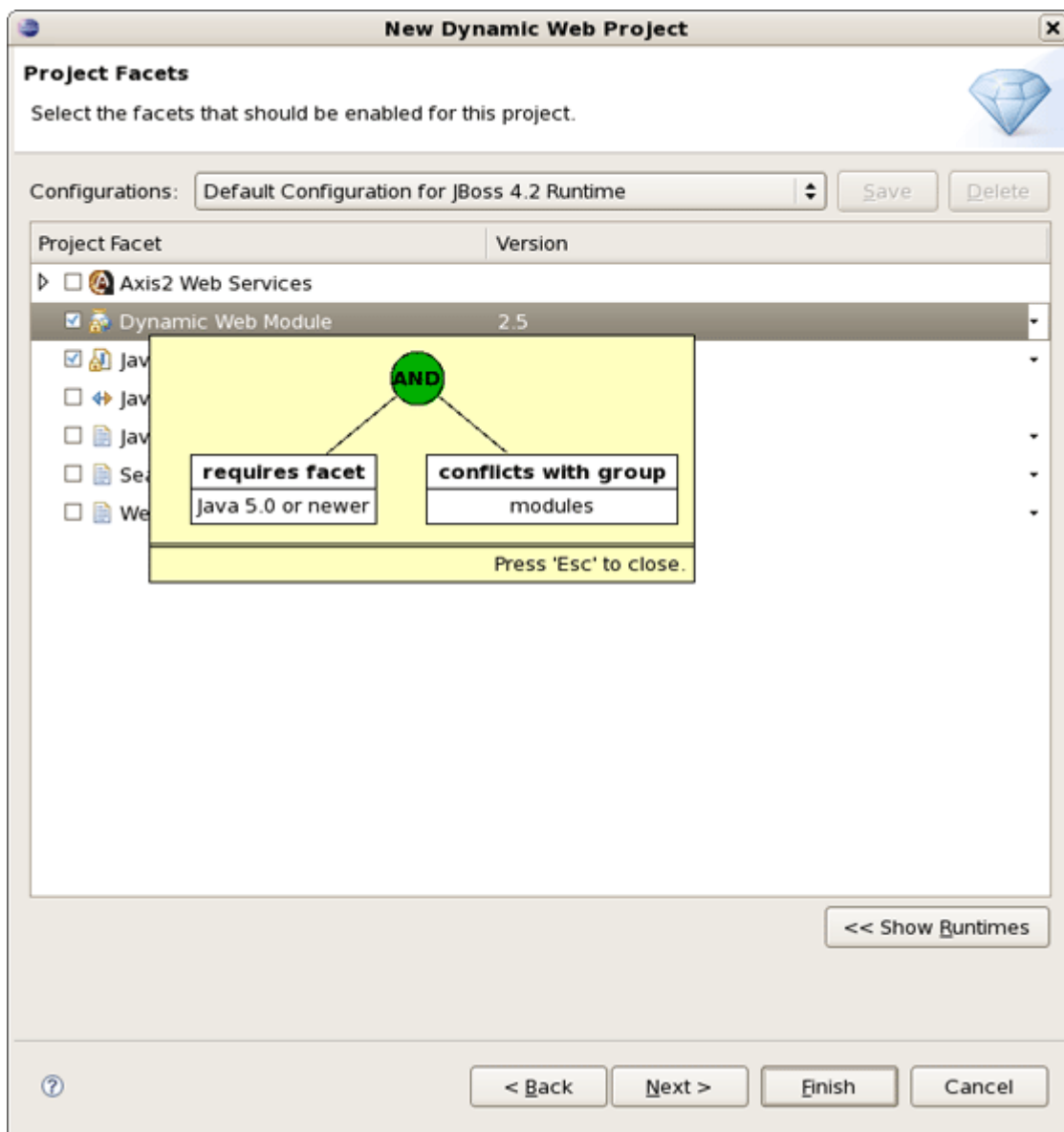
Figure 4.5. Facet Constraints
