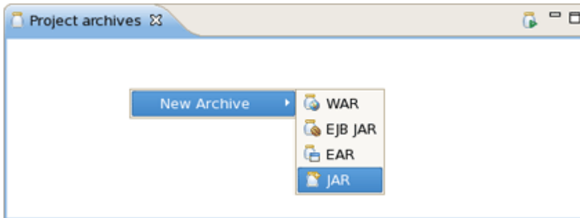
Figure 1.4. Archive Creating
