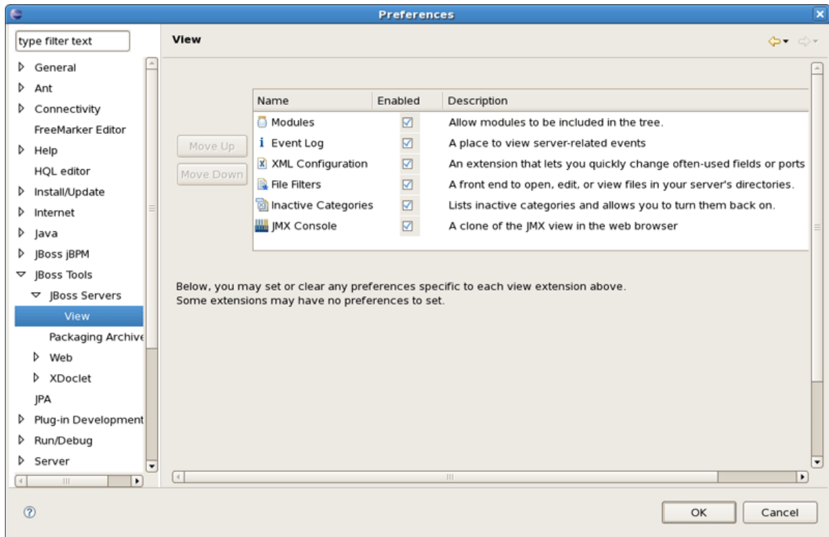
Figure 3.8. View Preferences
