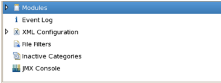
Figure 3.7. View Extensions
