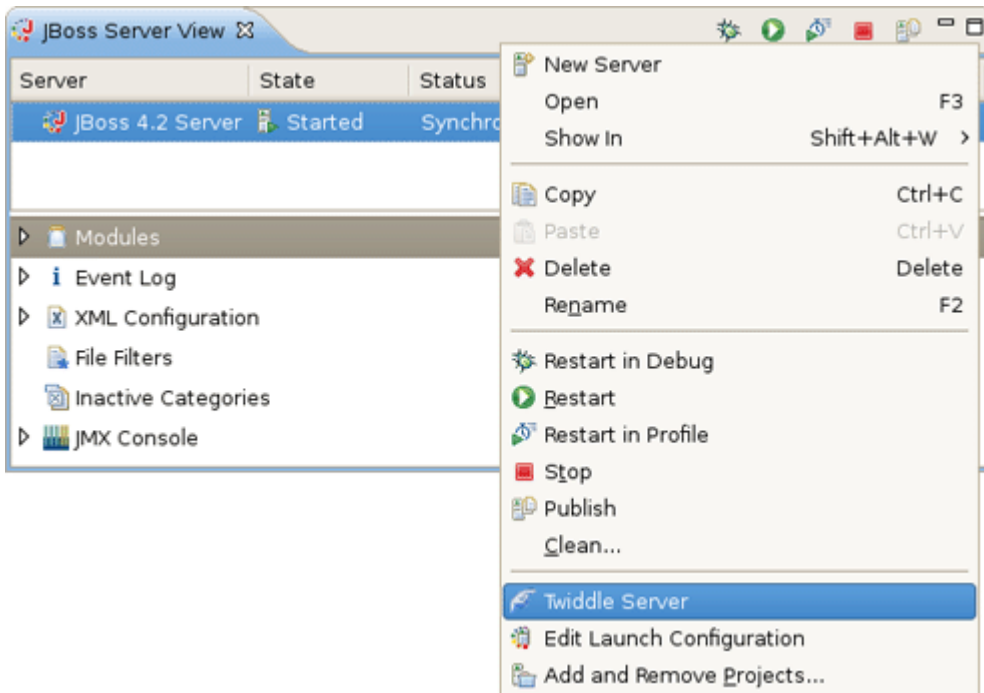
Figure 3.6. Twiddle Server
