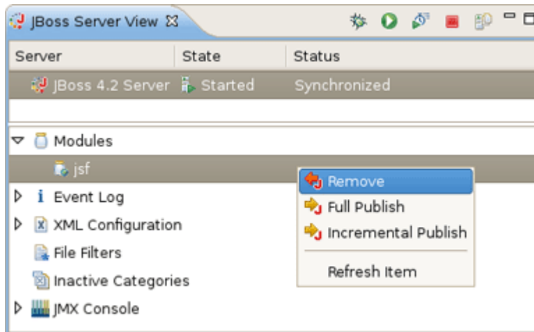
Figure 3.9. Modules Action
