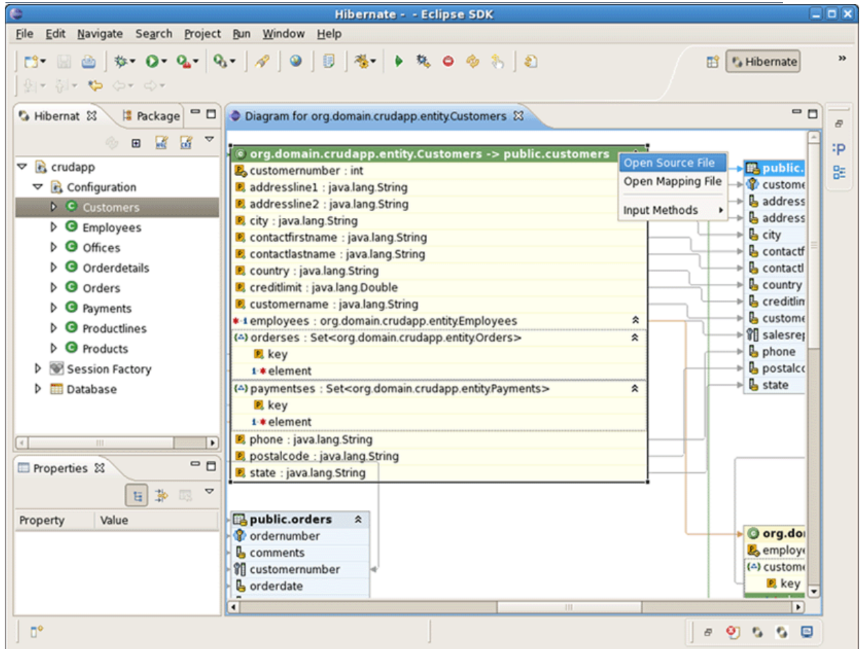
Figure 10.20. Mapping Diagram
