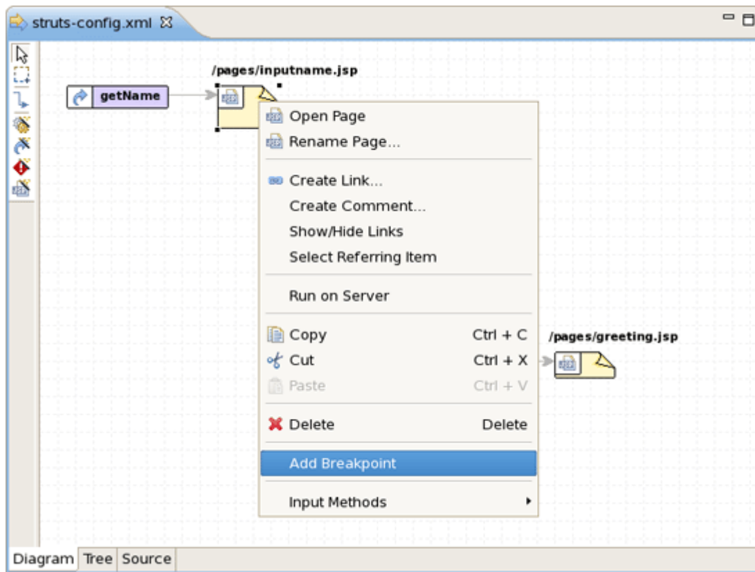
Figure 6.1. Adding Breakpoint
