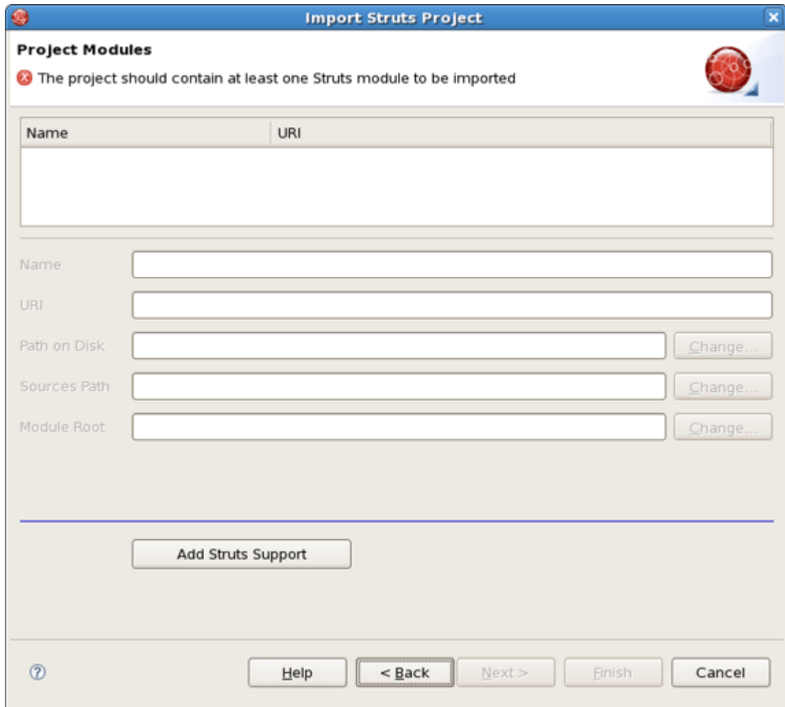
Figure 2.9. Project Modules
