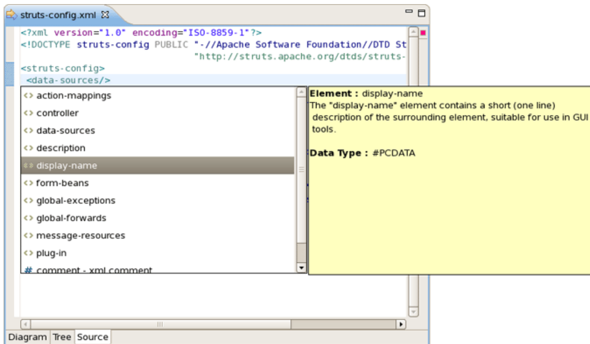
Figure 3.7. Code Assist
