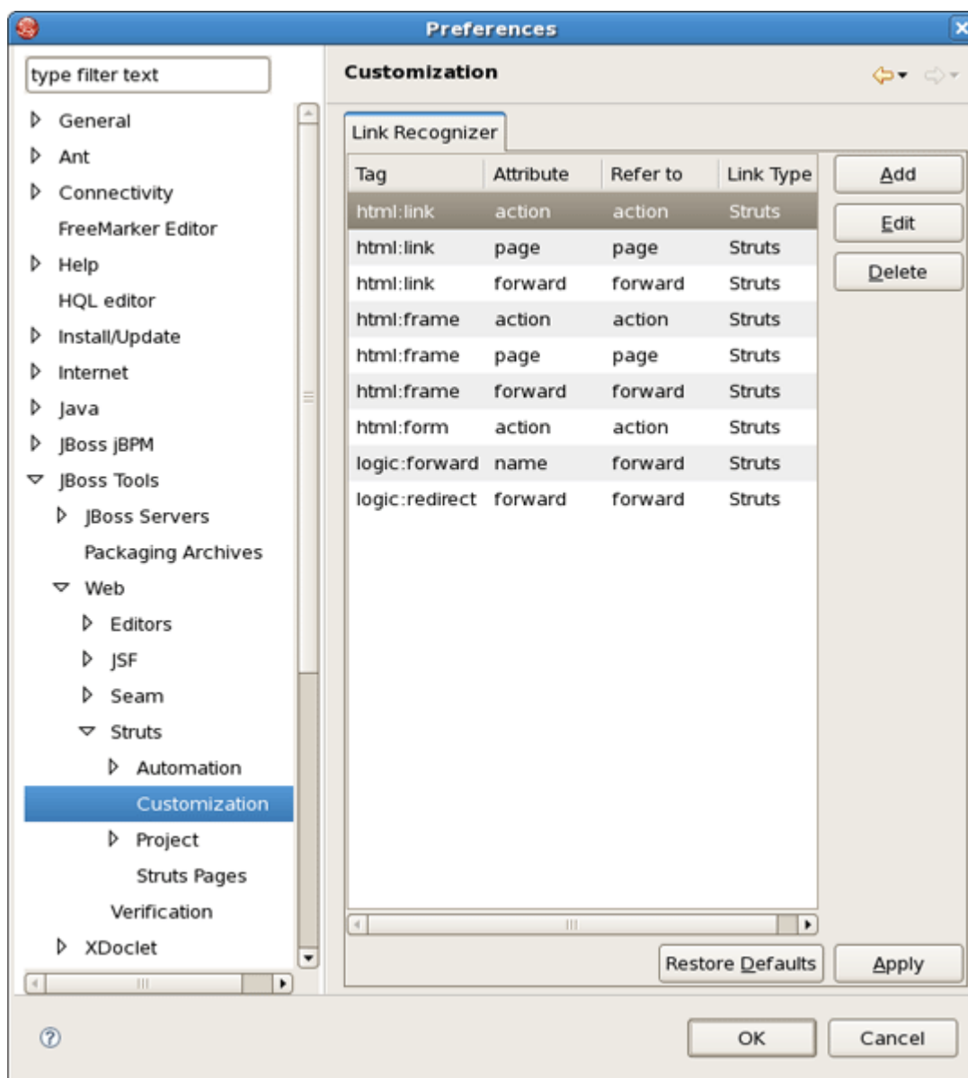
Figure 7.1. Customization Panel
