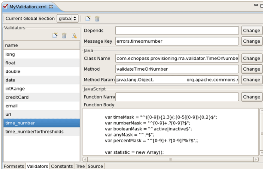
Figure 3.25. Validators View
