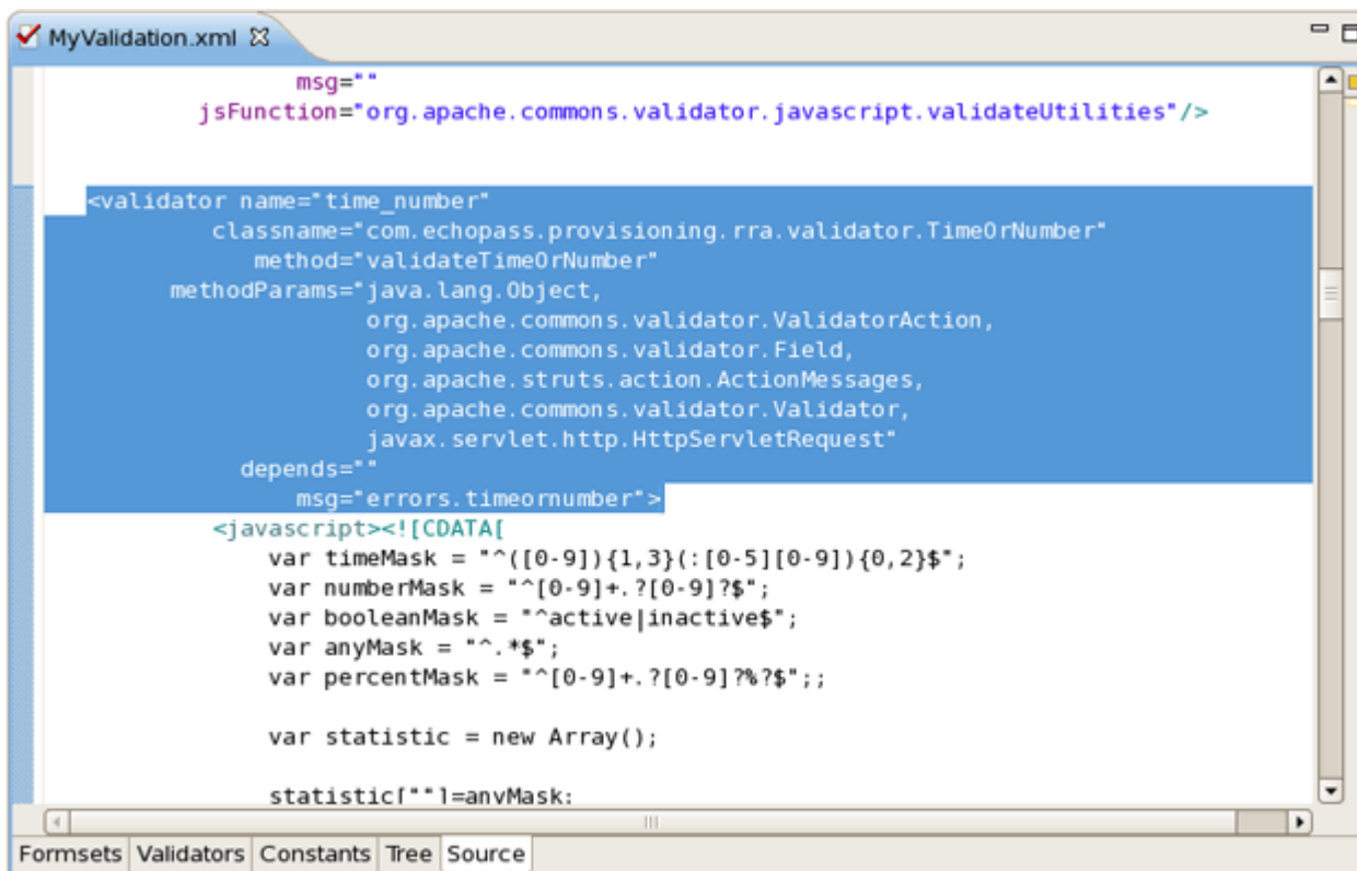
Figure 3.26. Validation Rules
