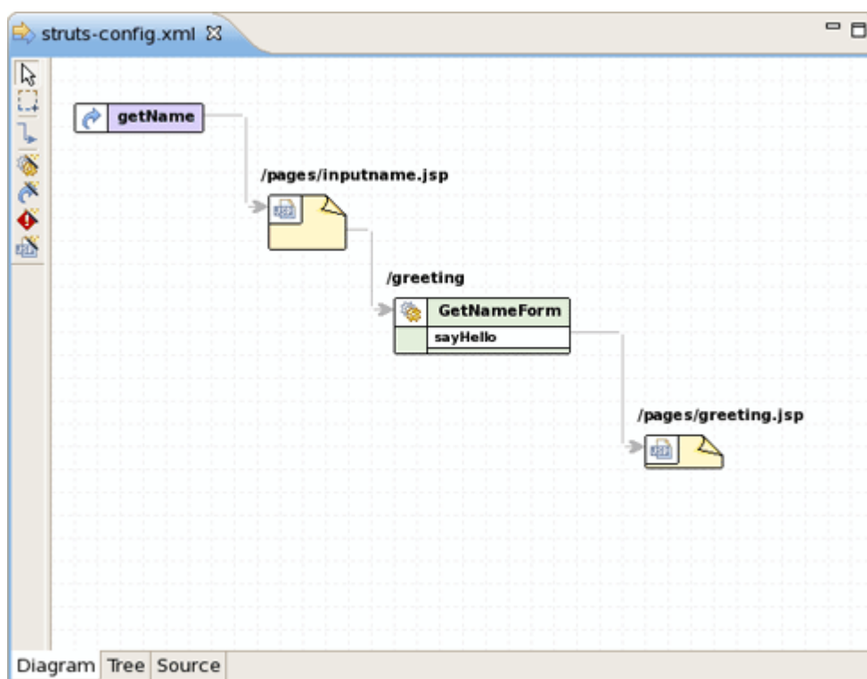
Figure 3.1. Diagram View
