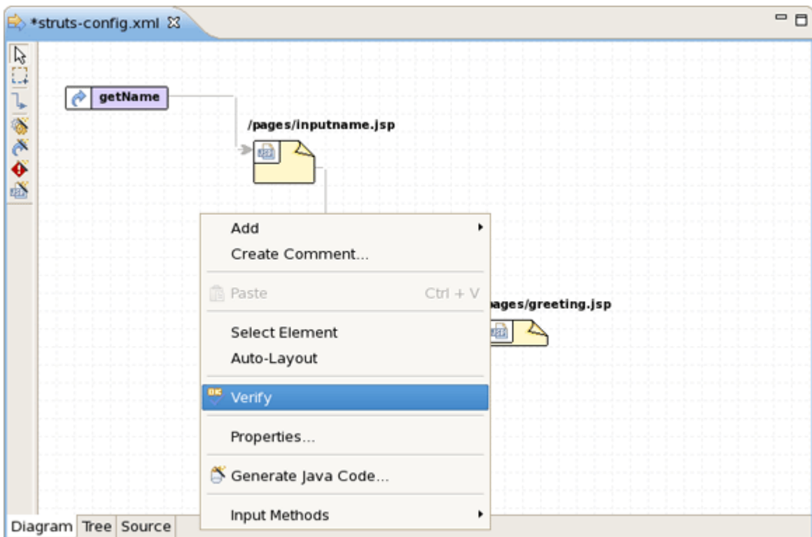
Figure 8.7. Verify Command
