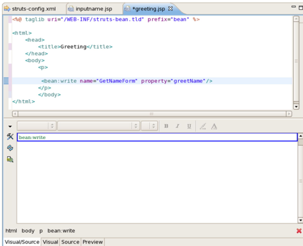
Figure 4.3. Editor Window
