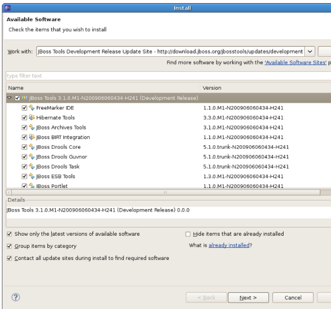
Figure 1.10. Updating Jboss Tools
