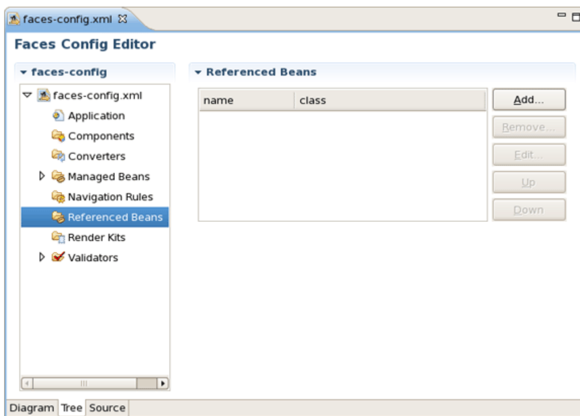
Figure 6.11. Referenced Beans in Faces Config Editor
