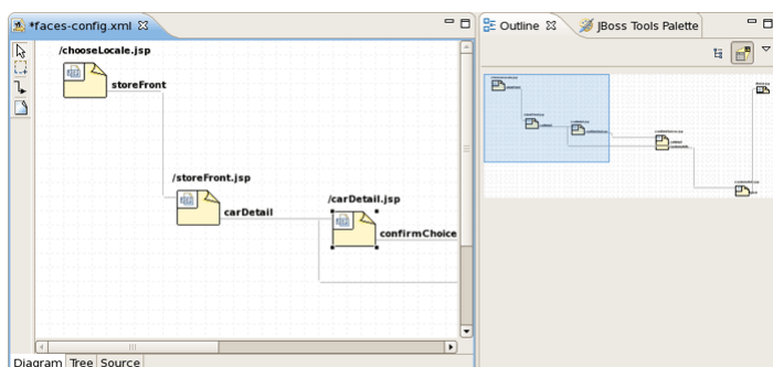
Figure 4.2. Outline View for Diagram
