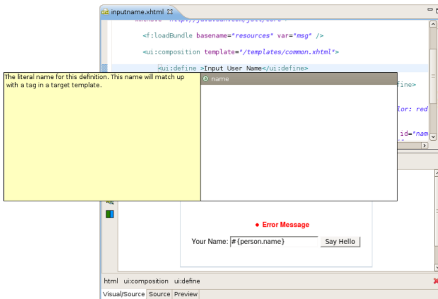
Figure 2.5. XHTML File Code Assist
