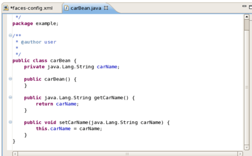
Figure 5.7. Generated Java Source Code for Property
