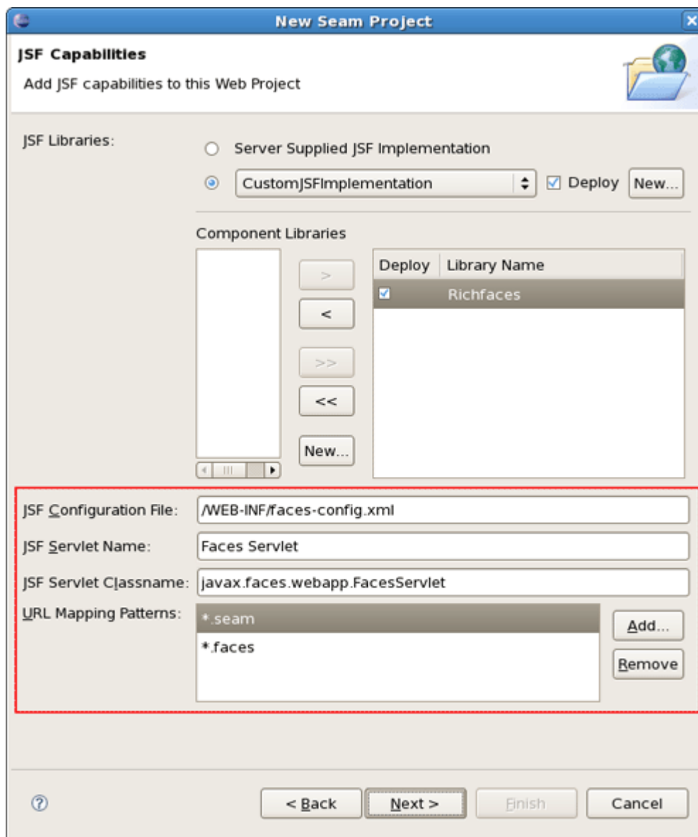
Figure 2.16. JSF Capabilities Wizard
